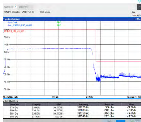
1-N78-3700-3800-PC2-30-20-H-6-CP-QPSK-Outer_Full-51@0-Ant1-1--PASS-see graph
