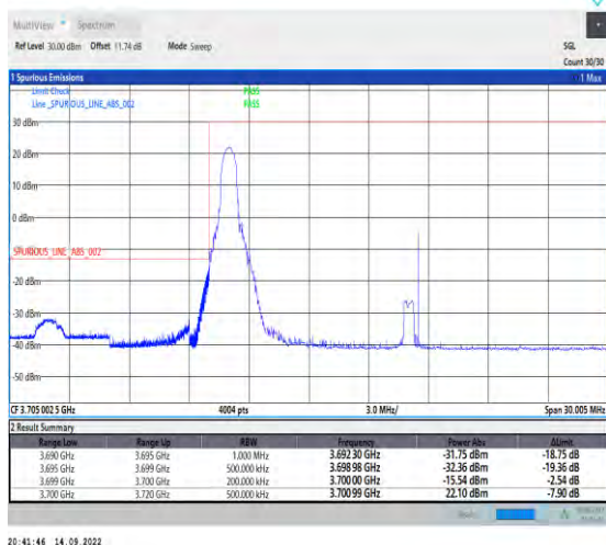
1-N78-3700-3800-PC2-30-20-L-1-DFT-PI2BPSK-Edge_1RB_Left-1@0-Ant1-1--PASS-see graph
