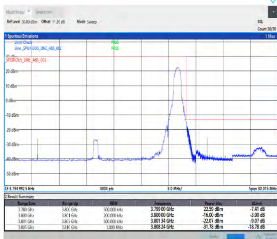
1-N78-3700-3800-PC2-30-20-H-2-DFT-PI2BPSK-Edge_1RB_Right-1@50-Ant1-1--PASS-see graph
