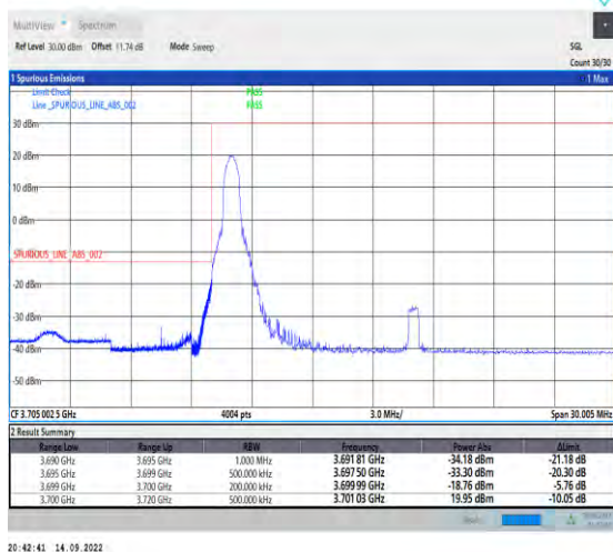
1-N78-3700-3800-PC2-30-20-L-4-CP-QPSK-Edge_1RB_Left-1@0-Ant1-1--PASS-see graph
