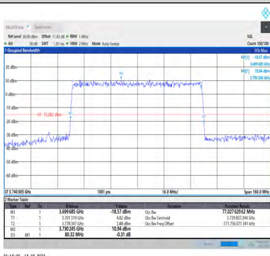
1-N78-3700-3800-PC2-30-80-L-4-DFT-64QAM-Outer r_Full-216@0-Ant1-77.028-80.320-≤80-PASS
