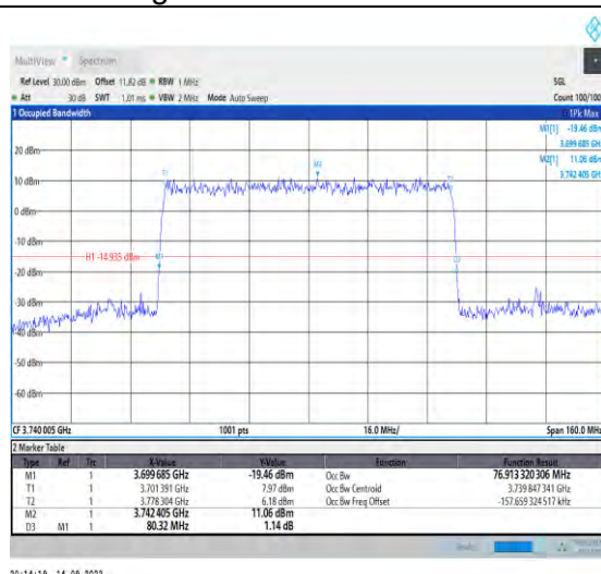
1-N78-3700-3800-PC2-30-80-L-3-DFT-16QAM-Outer _Full-216@0-Ant1-76.913-80.320-≤80-PASS
