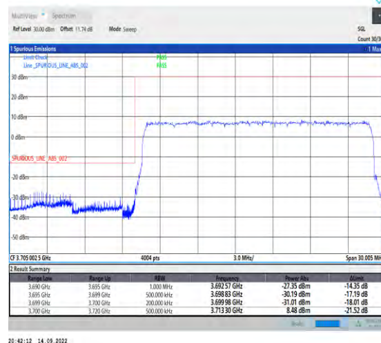
1-N78-3700-3800-PC2-30-20-L-3-DFT-PI2BPSK-Outer_Full-50@0-Ant1-1--PASS-see graph
