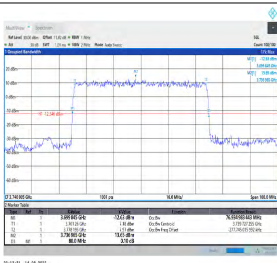
1-N78-3700-3800-PC2-30-80-L-2-DFT-PI2BPSK-Out er_Full-216@0-Ant1-76.935-80.000-≤80-PASS
