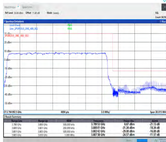
1-N78-3700-3800-PC2-30-20-H-3-DFT-PI2BPSK-Outer_Full-50@0-Ant1-1--PASS-see graph
