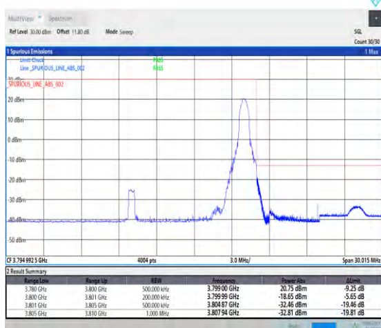
1-N78-3700-3800-PC2-30-20-H-5-CP-QPSK-Edge_1RB_Right-1@50-Ant1-1--PASS-see graph
