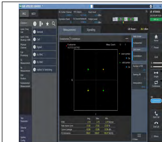
1-N78-3700-3800--30-100-M-1-DFT-PI2BPSK-Outter_Full-270@0-Ant1-see graph-PASS
