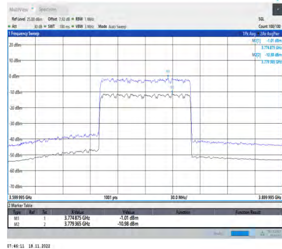
1-N78-3700-3800-PC2-30-100-L-2-CP-256QAM-Out er_Full-273@0-Ant1-9.97-100%-0.00-9.97-PASS-≤13
