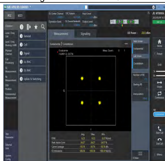
1-N78-3700-3800--30-100-M-6-CP-QPSK-Outer_Full-273@0-Ant1-see graph-PASS
