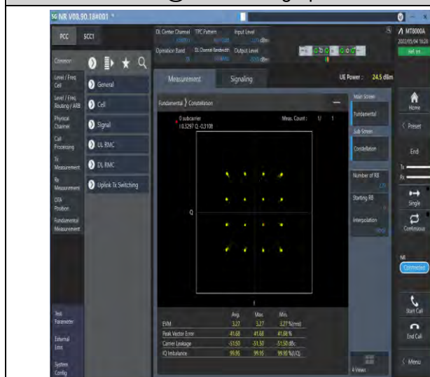
1-N78-3700-3800--30-100-M-3-DFT-16QAM-Outter_Full-270@0-Ant1-see graph-PASS
