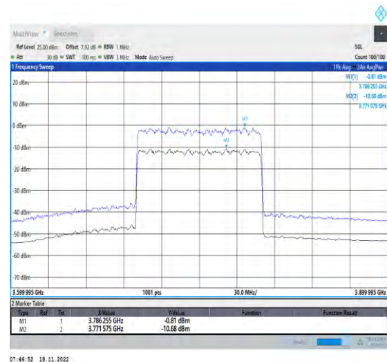
1-N78-3700-3800-PC2-30-100-M-2-CP-256QAM-Out er_Full-273@0-Ant1-9.87-100%-0.00-9.87-PASS-≤13
