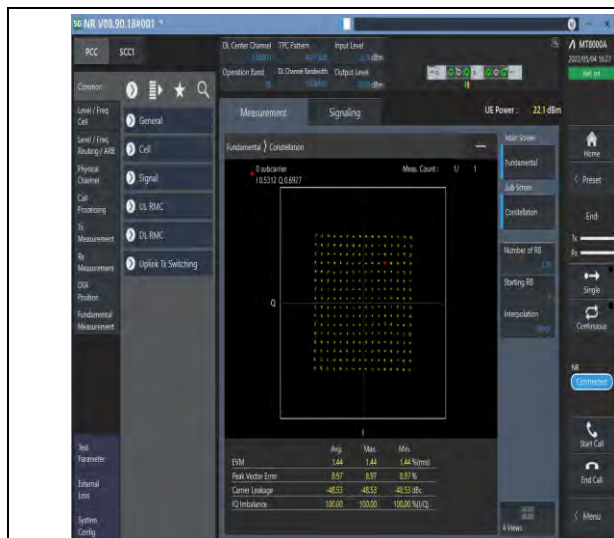
1-N78-3700-3800--30-100-M-5-DFT-256QAM-Outer_Full-270@0-Ant1-see graph-PASS
