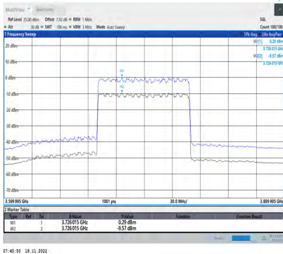
1-N78-3700-3800-PC2-30-100-L-1-DFT-256QAM-Out er_Full-270@0-Ant1-9.86-100%-0.00-9.86-PASS-≤13
