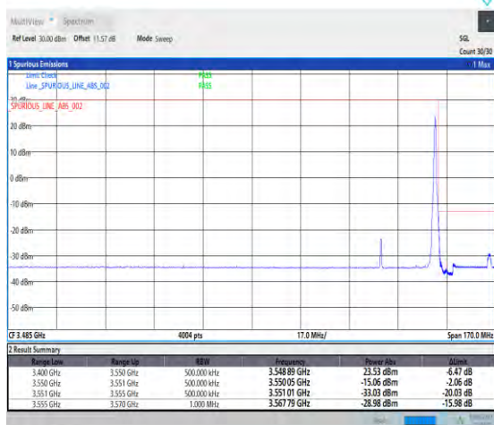
1-N78-3450-3550-PC2-30-40-H-2-DFT-PI2BPSK-Edge_1RB_Right-1@105-Ant1-1--PASS-see graph
