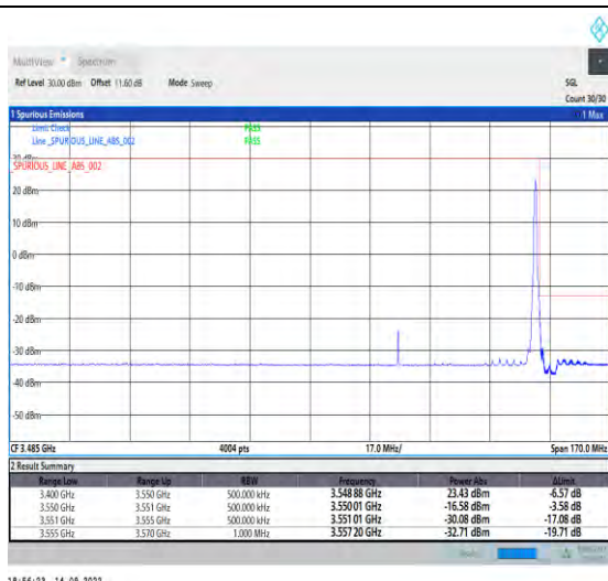
1-N78-3450-3550-PC2-30-80-H-2-DFT-PI2BPSK-Edge_1RB_Right-1@216-Ant1-1--PASS-see graph
