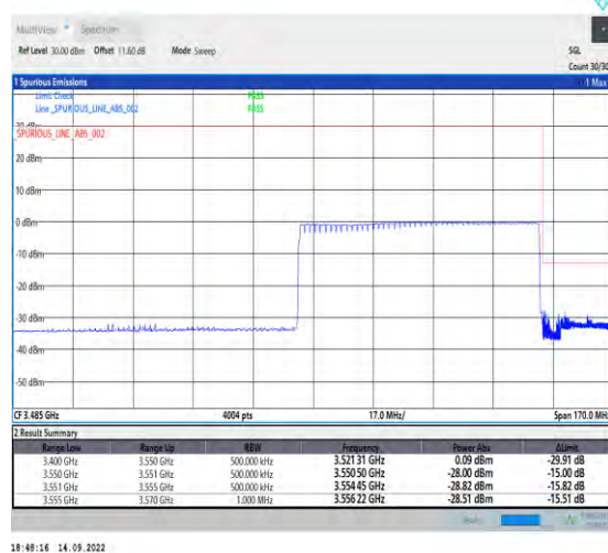
1-N78-3450-3550-PC2-30-70-H-6-CP-QPSK-Outer_Full-189@0-Ant1-1--PASS-see graph
