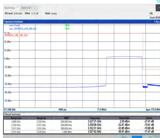
1-N78-3450-3550-PC2-30-40-H-6-CP-QPSK-Outer_Full-106@0-Ant1-1--PASS-see graph
