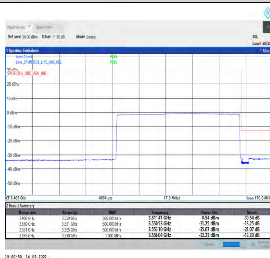
1-N78-3450-3550-PC2-30-80-H-6-CP-QPSK-Outer_Full-217@0-Ant1-1--PASS-see graph
