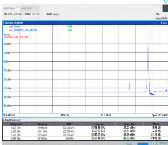
1-N78-3450-3550-PC2-30-40-H-5-CP-QPSK-Edge_1RB_Right-1@105-Ant1-1--PASS-see graph
