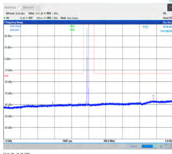
1-N78-3450-3550-PC2-30-100-M-1-DFT-PI2BPSK-In ner_1RB_Left-1@1-1000-6000-Ant1-5412.50--35.58--13-PASS
