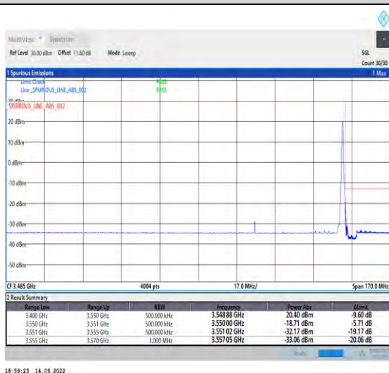
1-N78-3450-3550-PC2-30-80-H-5-CP-QPSK-Edge_1RB_Right-1@216-Ant1-1--PASS-see graph
