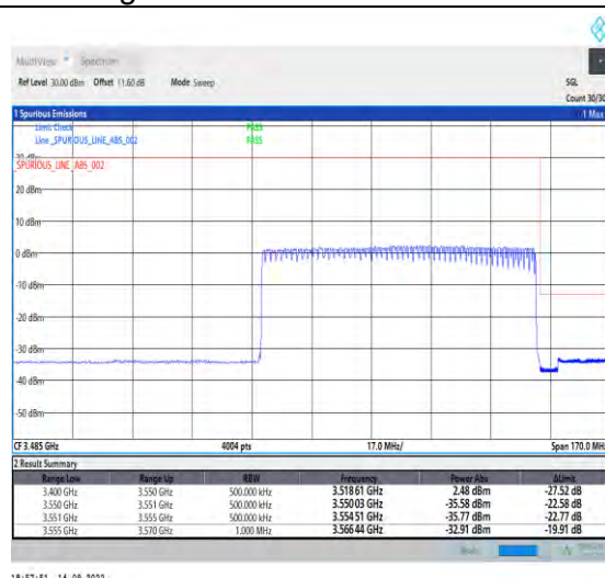
1-N78-3450-3550-PC2-30-80-H-3-DFT-PI2BPSK-Outer_Full-216@0-Ant1-1--PASS-see graph
