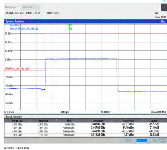
1-N78-3450-3550-PC2-30-90-L-3-DFT-PI2BPSK-Outer_Full-243@0-Ant1-1--PASS-see graph
