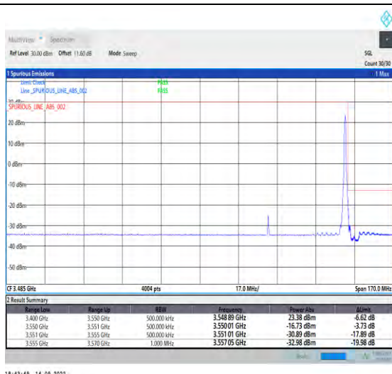
1-N78-3450-3550-PC2-30-70-H-2-DFT-PI2BPSK-Edge_1RB_Right-1@188-Ant1-1--PASS-see graph
