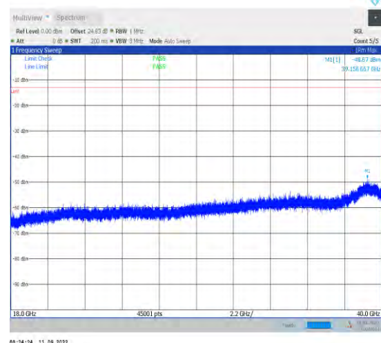
1-N78-3450-3550-PC2-30-100-M-1-DFT-PI2BPSK-In ner_1RB_Left-1@1-18000-40000-Ant1-18000.00--54.97--13-PASS
