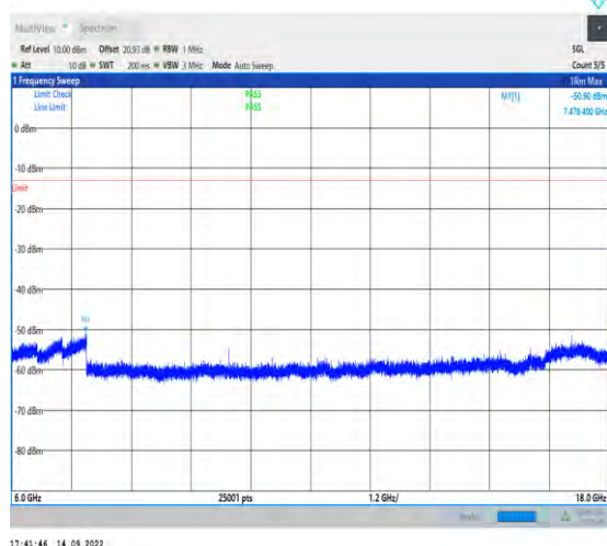
1-N78-3450-3550-PC2-30-100-M-1-DFT-PI2BPSK-I nner_1RB_Left-1@1-6000-18000-Ant1-7478.40--50.90--13-PASS
