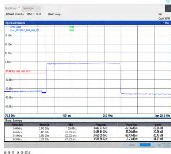
1-N78-3450-3550-PC2-30-90-L-6-CP-QPSK-Outer_Full-245@0-Ant1-1--PASS-see graph
