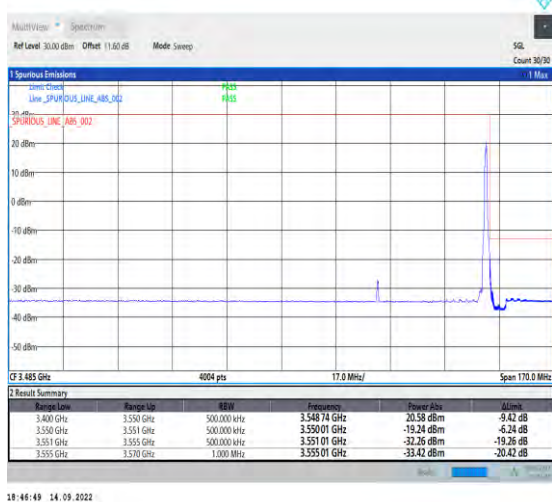
1-N78-3450-3550-PC2-30-70-H-5-CP-QPSK-Edge_1RB_Right-1@188-Ant1-1--PASS-see graph
