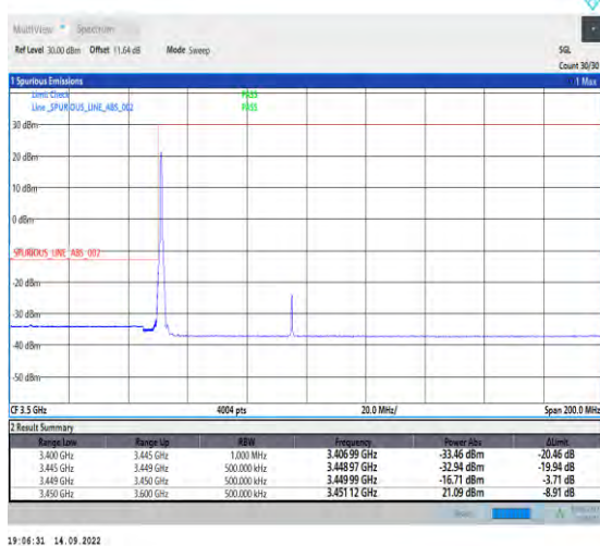
1-N78-3450-3550-PC2-30-90-L-4-CP-QPSK-Edge_1RB_Left-1@0-Ant1-1--PASS-see graph
