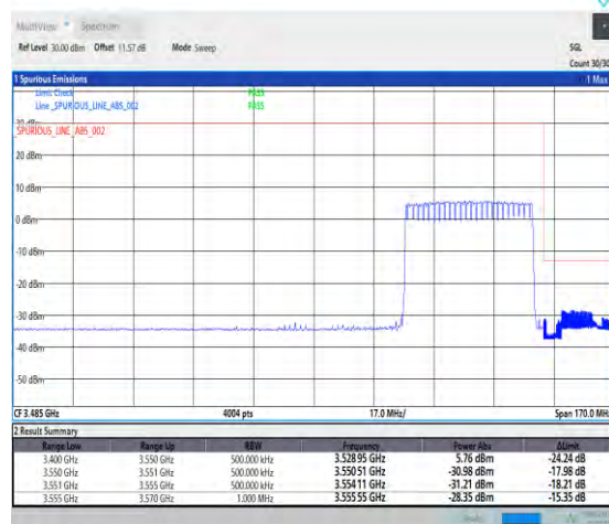
1-N78-3450-3550-PC2-30-40-H-3-DFT-PI2BPSK-Outer_Full-100@0-Ant1-1--PASS-see graph
