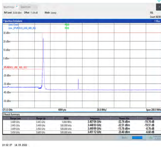
1-N78-3450-3550-PC2-30-90-L-1-DFT-PI2BPSK-Edge_1RB_Left-1@0-Ant1-1--PASS-see graph
