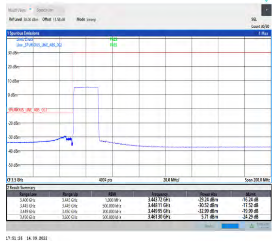
1-N78-3450-3550-PC2-30-20-L-6-CP-QPSK-Outer_Full-51@0-Ant1-1--PASS-see graph
