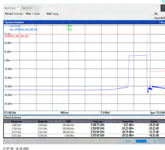
1-N78-3450-3550-PC2-30-20-H-6-CP-QPSK-Outer_Full-51@0-Ant1-1--PASS-see graph
