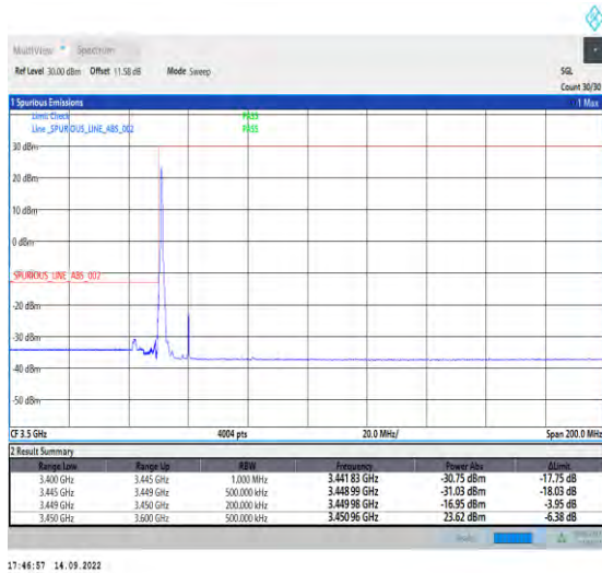
1-N78-3450-3550-PC2-30-20-L-1-DFT-PI2BPSK-Edge_1RB_Left-1@0-Ant1-1--PASS-see graph
