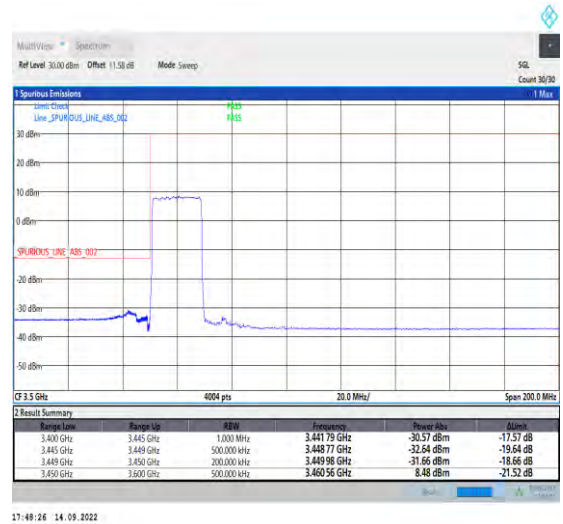
1-N78-3450-3550-PC2-30-20-L-3-DFT-PI2BPSK-Outer_Full-50@0-Ant1-1--PASS-see graph
