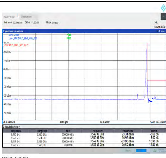
1-N78-3450-3550-PC2-30-20-H-2-DFT-PI2BPSK-Edge_1RB_Right-1@50-Ant1-1--PASS-see graph
