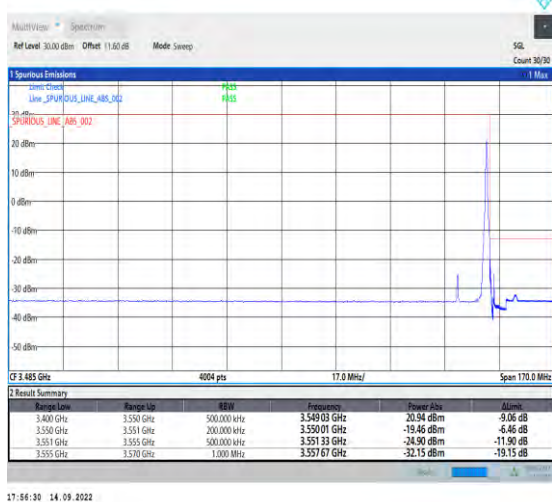
1-N78-3450-3550-PC2-30-20-H-5-CP-QPSK-Edge_1RB_Right-1@50-Ant1-1--PASS-see graph
