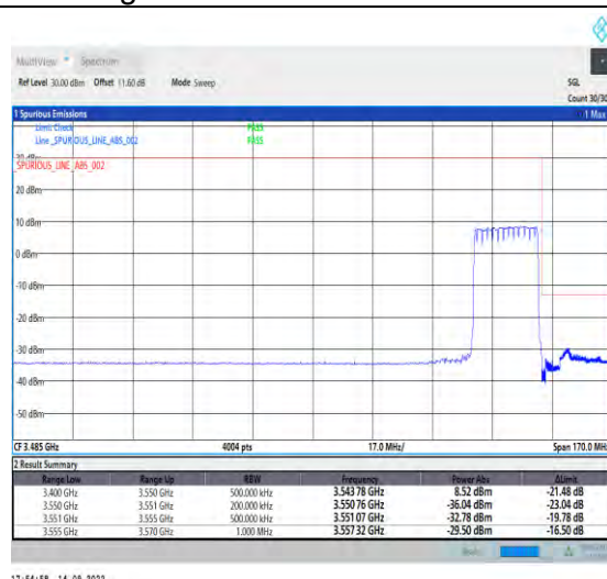
1-N78-3450-3550-PC2-30-20-H-3-DFT-PI2BPSK-Outer_Full-50@0-Ant1-1--PASS-see graph
