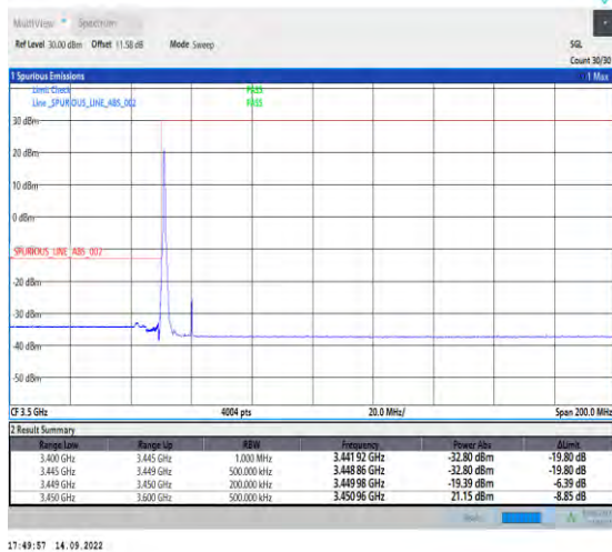
1-N78-3450-3550-PC2-30-20-L-4-CP-QPSK-Edge_1RB_Left-1@0-Ant1-1--PASS-see graph
