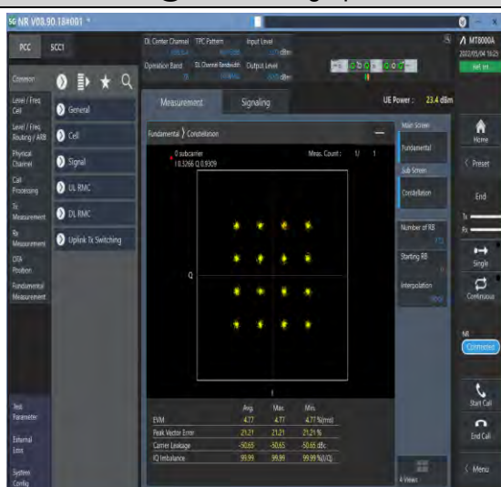
1-N78-3450-3550--30-100-M-7-CP-16QAM-Outer_Full-273@0-Ant1-see graph-PASS
