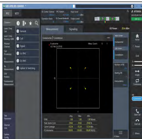
1-N78-3450-3550--30-100-M-2-DFT-QPSK-Outter_Full-270@0-Ant1-see graph-PASS
