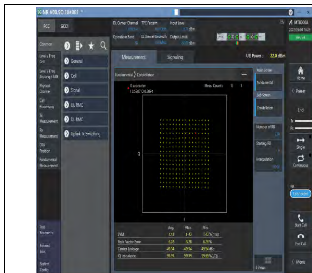
1-N78-3450-3550--30-100-M-5-DFT-256QAM-Outer_Full-270@0-Ant1-see graph-PASS
