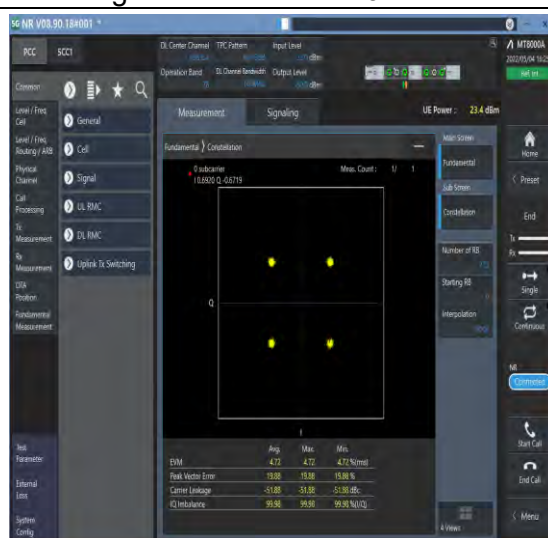
1-N78-3450-3550--30-100-M-6-CP-QPSK-Outer_Full-273@0-Ant1-see graph-PASS
