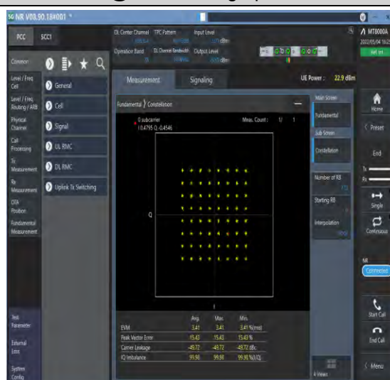
1-N78-3450-3550--30-100-M-8-CP-64QAM-Outer_Full-273@0-Ant1-see graph-PASS
