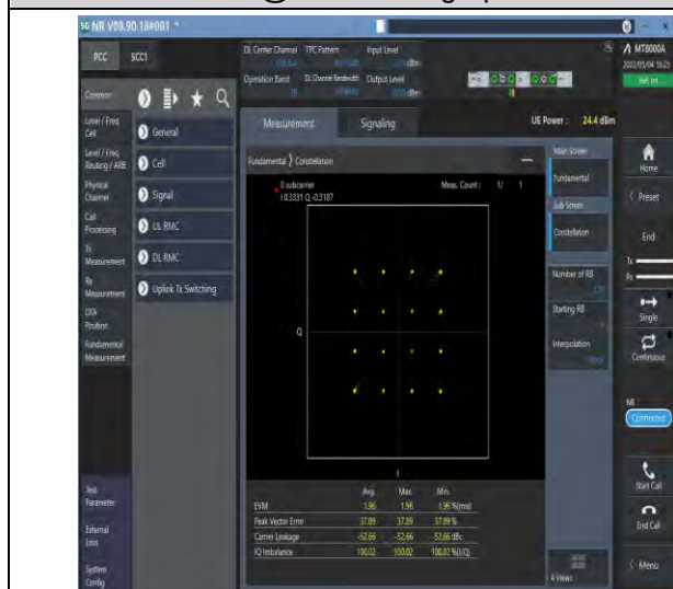
1-N78-3450-3550--30-100-M-3-DFT-16QAM-Outter_Full-270@0-Ant1-see graph-PASS
