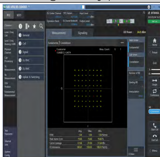
1-N78-3450-3550--30-100-M-4-DFT-64QAM-Outter_Full-270@0-Ant1-see graph-PASS
