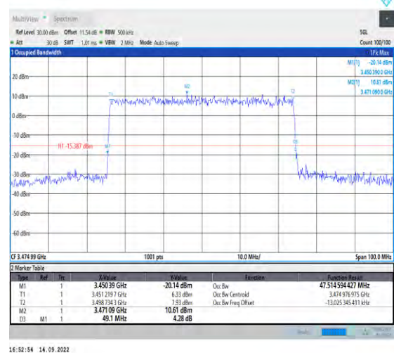
1-N78-3450-3550-PC2-30-50-L-6-CP-QPSK-Outer_Full-133@0-Ant1-47.515-49.100-≤50-PASS
