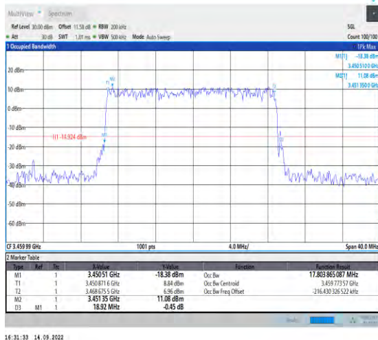
1-N78-3450-3550-PC2-30-20-L-3-DFT-16QAM-Outer_Full-50@0-Ant1-17.804-18.920-≤20-PASS
