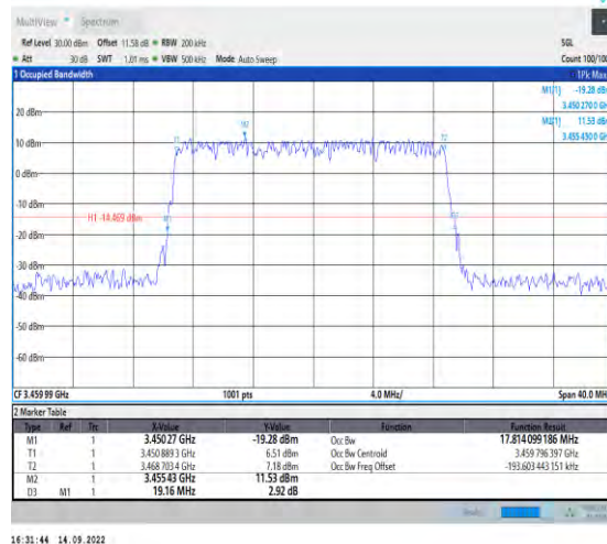
1-N78-3450-3550-PC2-30-20-L-4-DFT-64QAM-Outer_Full-50@0-Ant1-17.814-19.160-≤20-PASS
