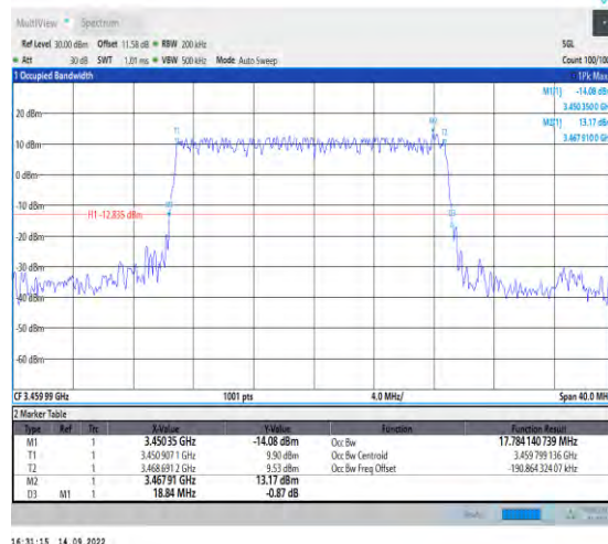
1-N78-3450-3550-PC2-30-20-L-2-DFT-PI2BPSK-Outer_Full-50@0-Ant1-17.784-18.840-≤20-PASS
