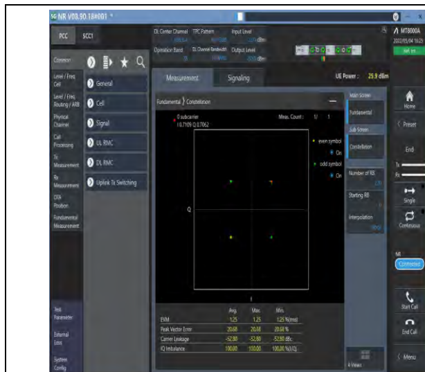
1-N78-3450-3550--30-100-M-1-DFT-PI2BPSK-Outter_Full-270@0-Ant1-see graph-PASS
