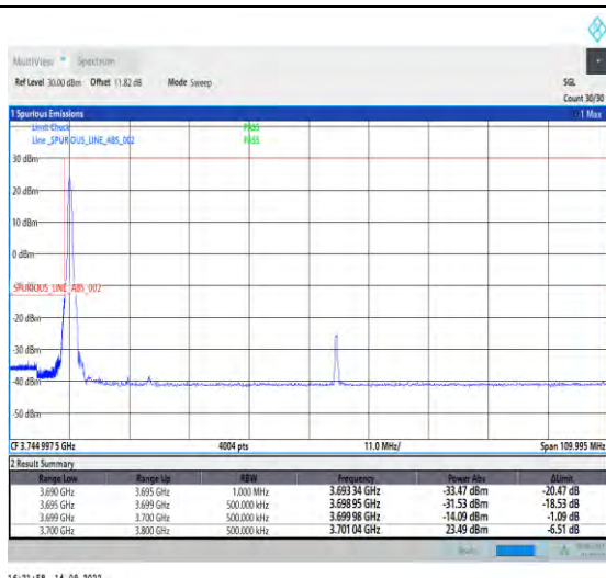
1-N77-3700-3980-PC2-30-100-L-1-DFT-PI2BPSK-Edge_1RB_Left-1@0-Ant1-1--PASS-see graph
