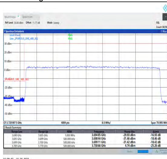
1-N77-3700-3980-PC2-30-70-L-3-DFT-PI2BPSK-Outer_Full-180@0-Ant1-1--PASS-see graph
