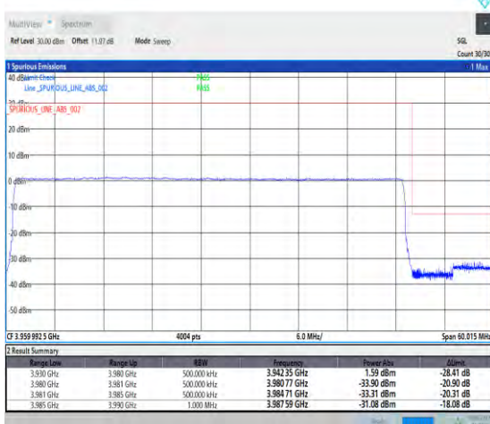
1-N77-3700-3980-PC2-30-50-H-6-CP-QPSK-Outer_Full-133@0-Ant1-1--PASS-see graph
