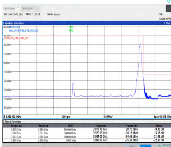
1-N77-3700-3980-PC2-30-50-H-5-CP-QPSK-Edge_1RB_Right-1@132-Ant1-1--PASS-see graph
