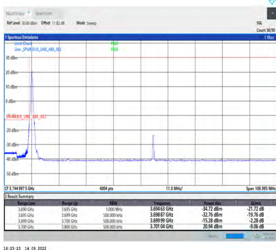
1-N77-3700-3980-PC2-30-100-L-4-CP-QPSK-Edge_1RB_Left-1@0-Ant1-1--PASS-see graph
