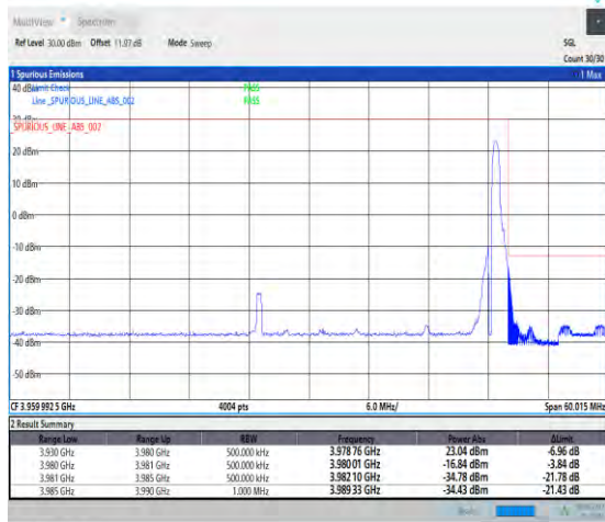
1-N77-3700-3980-PC2-30-50-H-2-DFT-PI2BPSK-Edge_1RB_Right-1@132-Ant1-1--PASS-see graph
