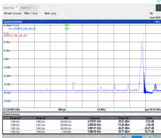
1-N77-3700-3980-PC2-30-80-H-5-CP-QPSK-Edge_1RB_Right-1@216-Ant1-1--PASS-see graph
