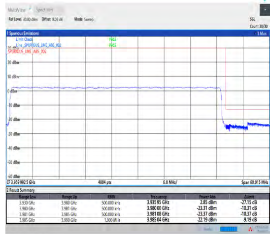
1-N77-3700-3980-PC2-30-50-H-3-DFT-PI2BPSK-Outer_Full-128@0-Ant1-1--PASS-see graph
