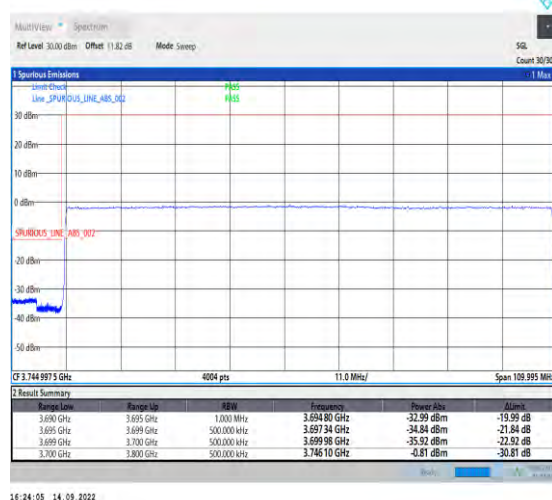
1-N77-3700-3980-PC2-30-100-L-6-CP-QPSK-Outer_Full-273@0-Ant1-1--PASS-see graph
