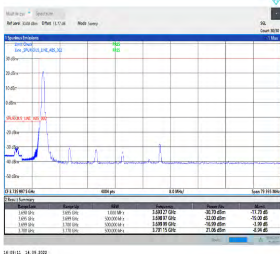
1-N77-3700-3980-PC2-30-70-L-4-CP-QPSK-Edge_1RB_Left-1@0-Ant1-1--PASS-see graph
