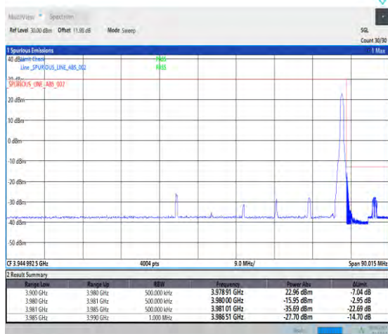
1-N77-3700-3980-PC2-30-80-H-2-DFT-PI2BPSK-Edge_1RB_Right-1@216-Ant1-1--PASS-see graph
