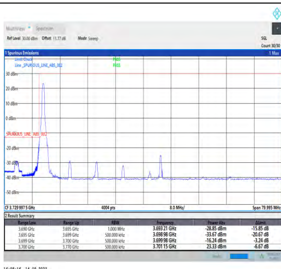
1-N77-3700-3980-PC2-30-70-L-1-DFT-PI2BPSK-Edge_1RB_Left-1@0-Ant1-1--PASS-see graph
