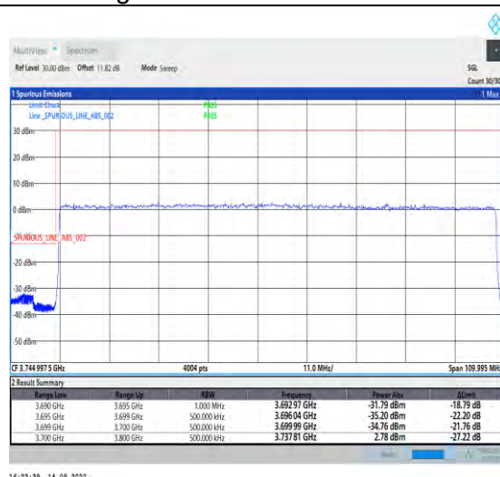
1-N77-3700-3980-PC2-30-100-L-3-DFT-PI2BPSK-Outer_Full-270@0-Ant1-1--PASS-see graph
