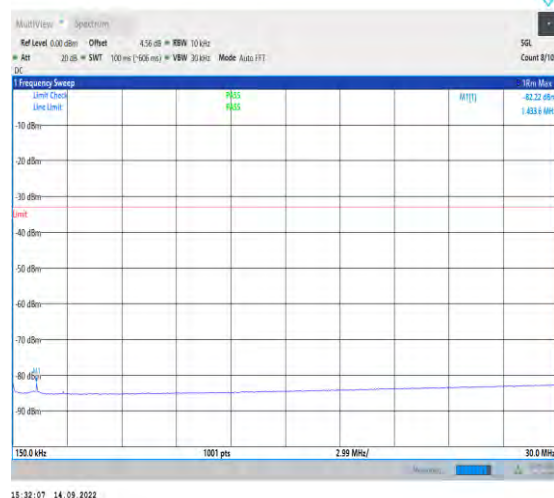
1-N77-3700-3980-PC2-30-100-H-1-DFT-PI2BPSK-Inner_1RB_Left-1@1-0.15-30-Ant1-1.43--82.22--33-PA SS
