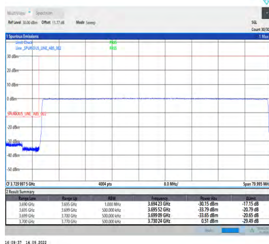
1-N77-3700-3980-PC2-30-70-L-6-CP-QPSK-Outer_Full-189@0-Ant1-1--PASS-see graph
