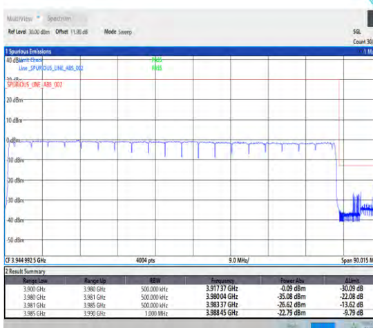
1-N77-3700-3980-PC2-30-80-H-6-CP-QPSK-Outer_Full-217@0-Ant1-1--PASS-see graph
