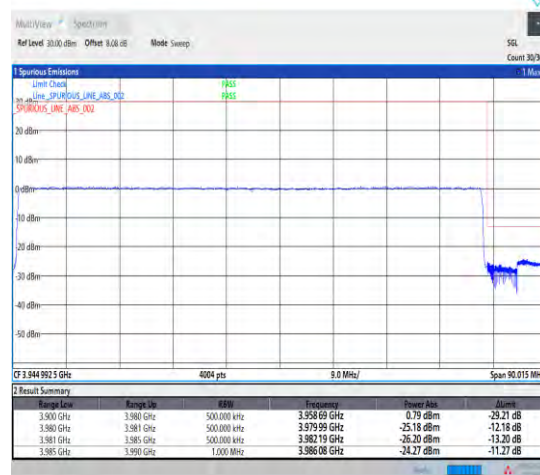
1-N77-3700-3980-PC2-30-80-H-3-DFT-PI2BPSK-Outer_Full-216@0-Ant1-1--PASS-see graph
