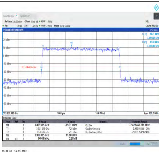
1-N77-3700-3980-PC2-30-80-H-8-CP-64QAM-Outer_Full-217@0-Ant1-77.472-80.480-≤80-PASS
