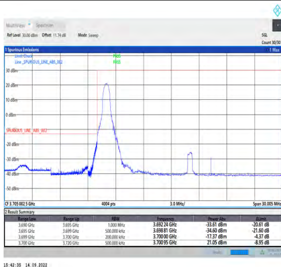
1-N77-3700-3980-PC2-30-20-L-4-CP-QPSK-Edge_1RB_Left-1@0-Ant1-1--PASS-see graph
