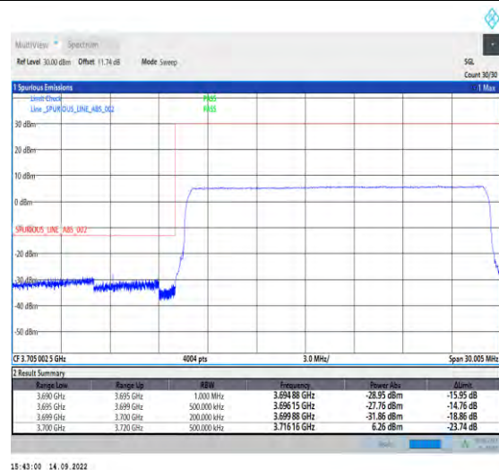
1-N77-3700-3980-PC2-30-20-L-6-CP-QPSK-Outer_Full-51@0-Ant1-1--PASS-see graph
