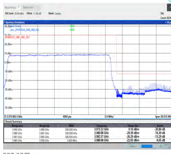
1-N77-3700-3980-PC2-30-20-H-3-DFT-PI2BPSK-Outer_Full-50@0-Ant1-1--PASS-see graph
