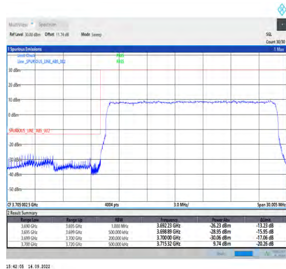
1-N77-3700-3980-PC2-30-20-L-3-DFT-PI2BPSK-Outer_Full-50@0-Ant1-1--PASS-see graph
