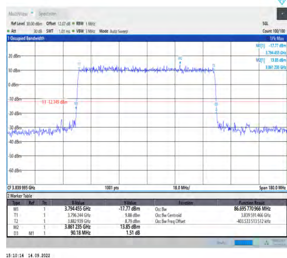
1-N77-3700-3980-PC2-30-90-M-1-DFT-QPSK-Outer_Full-243@0-Ant1-86.696-90.180-≤90-PASS
