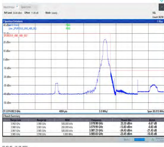
1-N77-3700-3980-PC2-30-20-H-2-DFT-PI2BPSK-Edge_1RB_Right-1@50-Ant1-1--PASS-see graph
