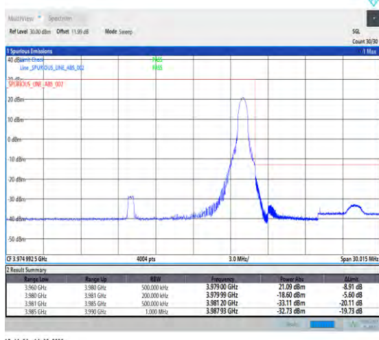
1-N77-3700-3980-PC2-30-20-H-5-CP-QPSK-Edge_1RB_Right-1@50-Ant1-1--PASS-see graph
