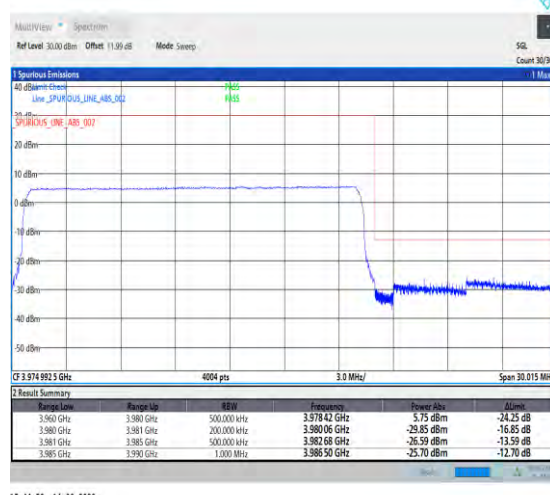
1-N77-3700-3980-PC2-30-20-H-6-CP-QPSK-Outer_Full-51@0-Ant1-1--PASS-see graph
