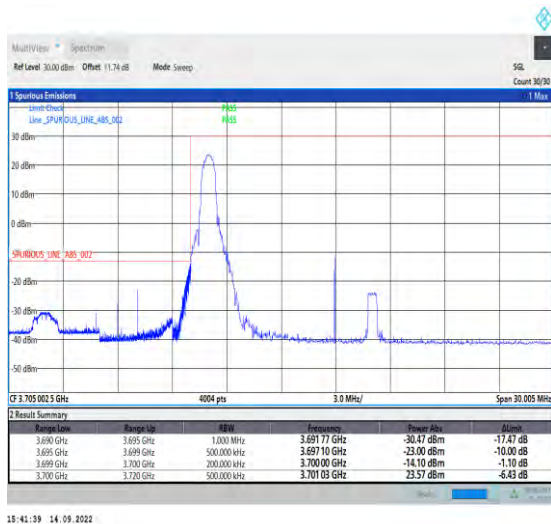
1-N77-3700-3980-PC2-30-20-L-1-DFT-PI2BPSK-Edge_1RB_Left-1@0-Ant1-1--PASS-see graph
