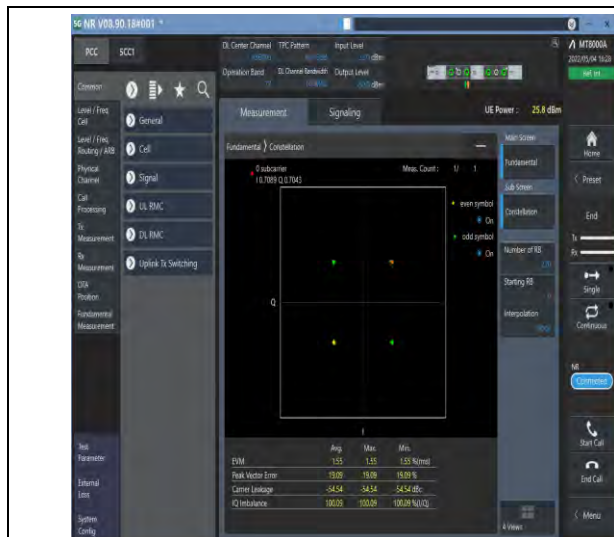
1-N77-3700-3980-PC2-30-100-M-1-DFT-PI2BPSK-Out_Full-270@0-Ant1-see graph-PASS
