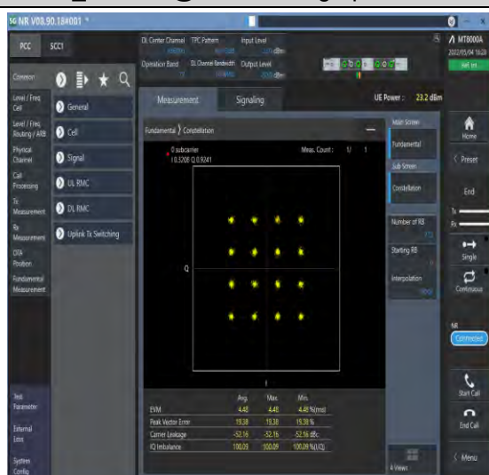
1-N77-3700-3980-PC2-30-100-M-7-CP-16QAM-Outer _Full-273@0-Ant1-see graph-PASS
