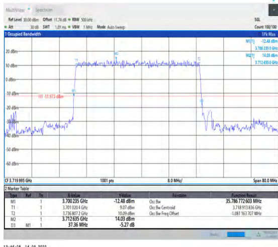
1-N77-3700-3980-PC2-30-40-L-2-DFT-PI2BPSK-Out er_Full-100@0-Ant1-35.787-37.360-≤40-PASS
