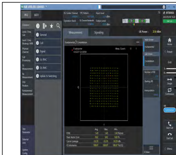
1-N77-3700-3980-PC2-30-100-M-5-DFT-256QAM-Out _Full-270@0-Ant1-see graph-PASS
