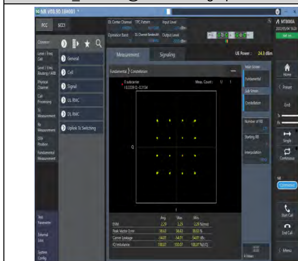
1-N77-3700-3980-PC2-30-100-M-3-DFT-16QAM-Out_Full-270@0-Ant1-see graph-PASS
