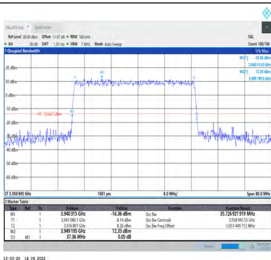
1-N77-3700-3980-PC2-30-40-H-4-DFT-64QAM-Out r_Full-100@0-Ant1-35.727-37.360-≤40-PASS
