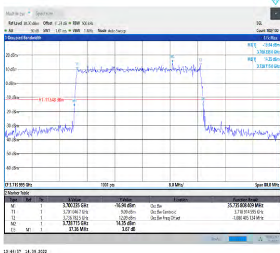
1-N77-3700-3980-PC2-30-40-L-4-DFT-64QAM-Outer r_Full-100@0-Ant1-35.736-37.360-≤40-PASS
