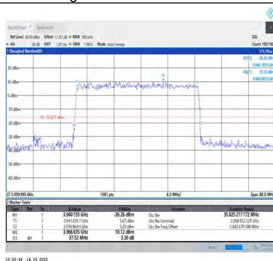
1-N77-3700-3980-PC2-30-40-H-5-DFT-256QAM-Out er_Full-100@0-Ant1-35.825-37.520-≤40-PASS
