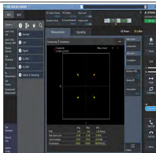
1-N77-3700-3980-PC2-30-100-M-2-DFT-QPSK-Out_Full-270@0-Ant1-see graph-PASS
