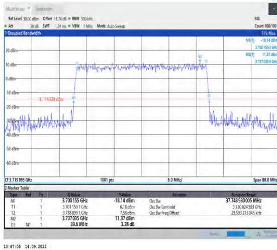
1-N77-3700-3980-PC2-30-40-L-6-CP-QPSK-Outer_Full-106@0-Ant1-37.749-39.600-≤40-PASS
