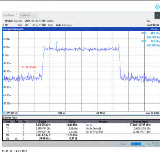
1-N77-3700-3980-PC2-30-40-H-6-CP-QPSK-Outer Full-106@0-Ant1-37.889-39.440-≤40-PASS
