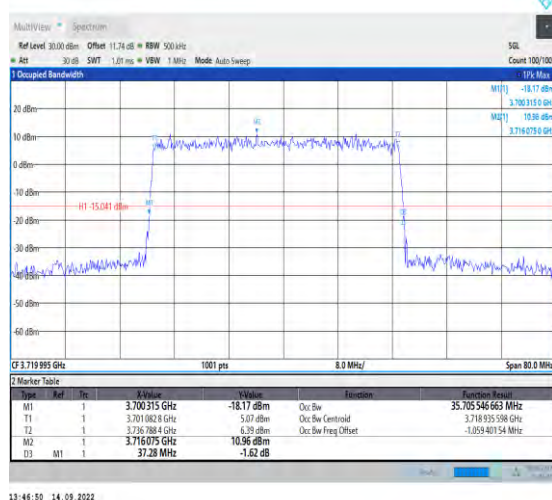
1-N77-3700-3980-PC2-30-40-L-5-DFT-256QAM-Outer er_Full-100@0-Ant1-35.706-37.280-≤40-PASS
