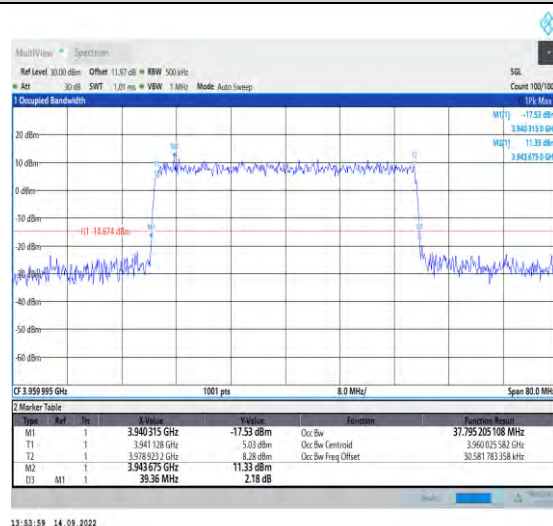
1-N77-3700-3980-PC2-30-40-H-7-CP-16QAM-Outer _Full-106@0-Ant1-37.795-39.360-≤40-PASS
