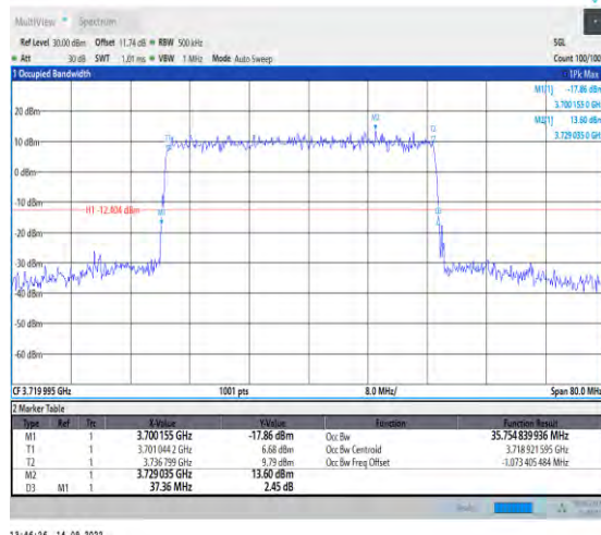
1-N77-3700-3980-PC2-30-40-L-3-DFT-16QAM-Outer _Full-100@0-Ant1-35.755-37.360-≤40-PASS
