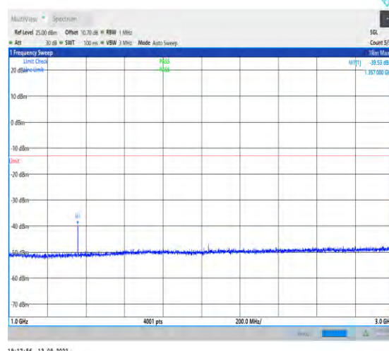
1-N71-15-20-H-1-DFT-PI2BPSK-Inner_1RB_Left-1@ 1-1000-3000-Ant1-1357.50--39.53--13-PASS
