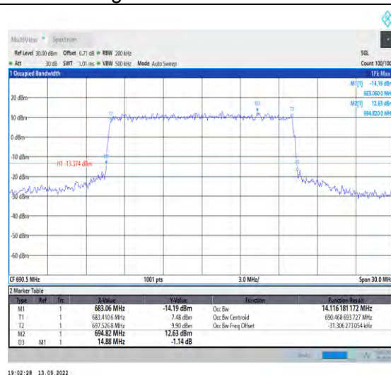
1-N71-15-15-H-6-CP-QPSK-Outer_Full-79@0-Ant1- 14.116-14.880-≤15-PASS
