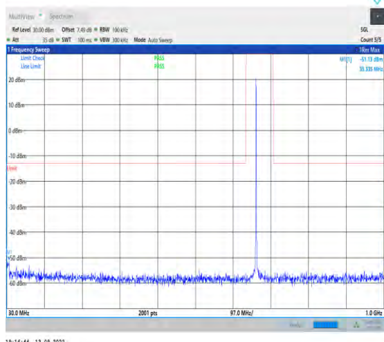
1-N71-15-20-M-1-DFT-PI2BPSK-Inner_1RB_Left-1 @ 1-30-1000-Ant1-34.37--51.13--13-PASS
