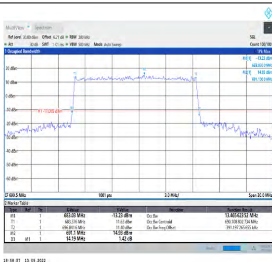
1-N71-15-15-H-1-DFT-QPSK-Outer_Full-75@0-Ant1 -13.466-14.190≤15-PASS
