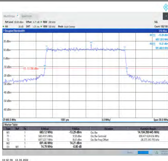
1-N71-15-15-H-7-CP-16QAM-Outer_Full-79@0-Ant1 -14.104-14.790-≤15-PASS
