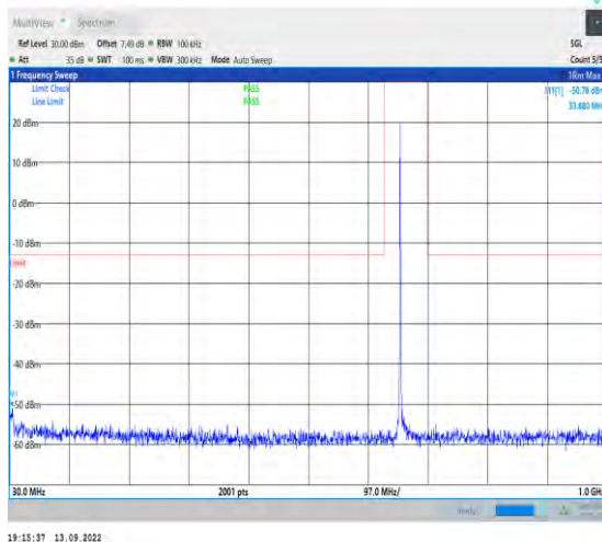
1-N71-15-20-L-1-DFT-PI2BPSK-Inner_1RB_Left-1 @1-30-1000-Ant1-34.85--50.78--13-PASS
