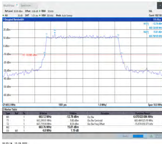
1-N71-15-5-L-1-DFT-QPSK-Outer_Full-25@0-Ant1-4 -4.7-4.800-≤5-PASS
