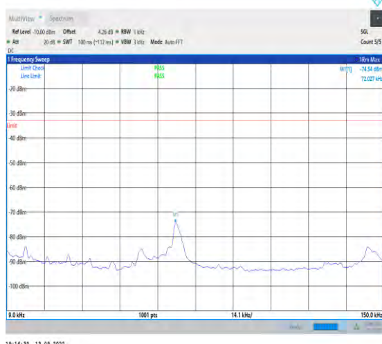
1-N71-15-20-M-1-DFT-PI2BPSK-Inner_1RB_Left-1 @ 1-0.009-0.15-Ant1-0.03--74.54--33-PASS
