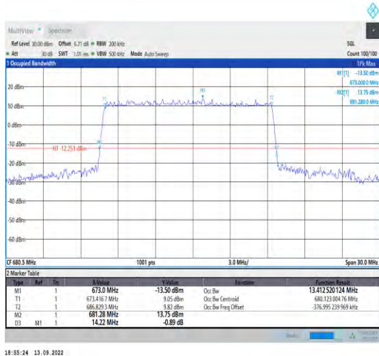
1-N71-15-15-M-4-DFT-64QAM-Outer_Full-75@0-Ant 1-13.413-14.220-≤15-PASS
