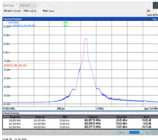
1-N71-15-5-L-4-CP-QPSK-Edge_1RB_Left-1@0-Ant1-1--PASS-see graph
