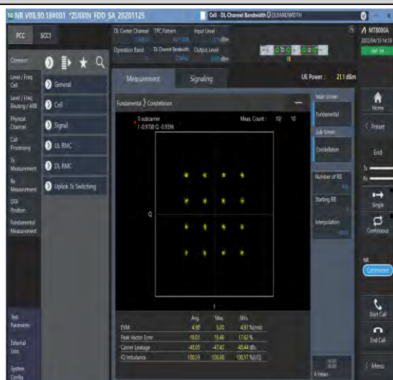
1-N71--15-20-M-7-CP-16QAM-Outer_Full-106@0-Ant 1-see graph-PASS
