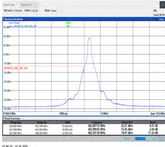
1-N71-15-5-L-1-DFT-PI2BPSK-Edge_1RB_Left-1@0-Ant1-1--PASS-see graph
