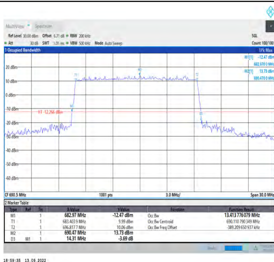
1-N71-15-15-H-3-DFT-16QAM-Outer_Full-75@0-Ant1 1-13.414-14.310≤15-PASS
