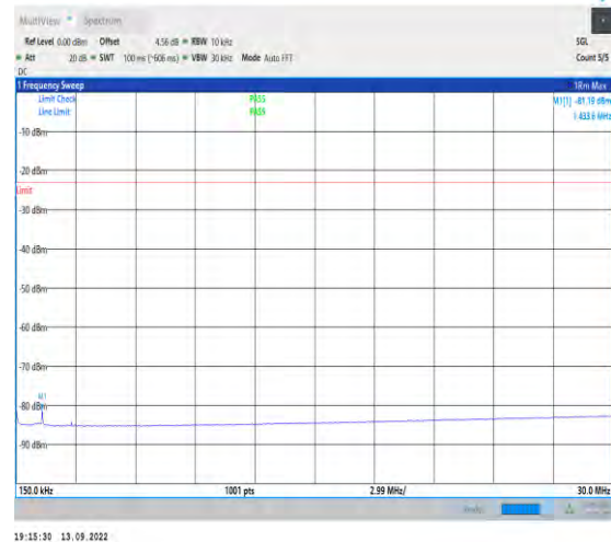
1-N71-15-20-L-1-DFT-PI2BPSK-Inner_1RB_Left-1@ 1-0.15-30-Ant1-0.51--81.19--23-PASS
