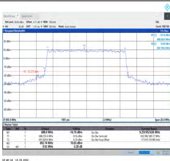
1-N71-15-10-H-6-CP-QPSK-Outer_Full-52@0-Ant1 9.254-9.920-≤10-PASS
