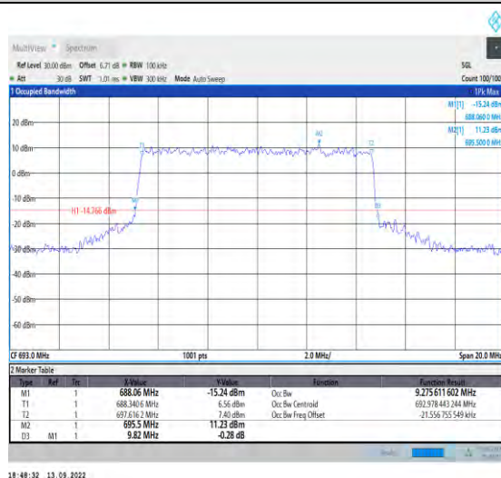
1-N71-15-10-H-7-CP-16QAM-Outer_Full-52@0-Ant1 -9.276-9.820-≤10-PASS
