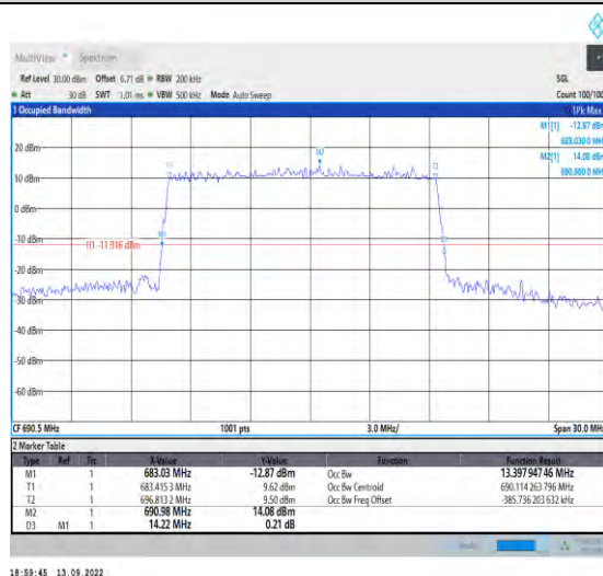
1-N71-15-15-H-4-DFT-64QAM-Outer_Full-75@0-Ant1 1-13.398-14.220≤15-PASS
