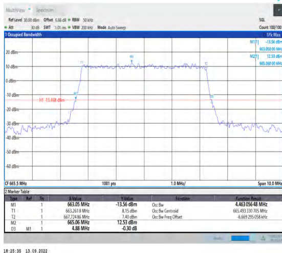
1-N71-15-5-L-3-DFT-16QAM-Outer_Full-25@0-Ant1-4 -4.463-4.880-≤5-PASS
