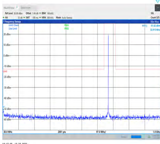
1-N71-15-20-H-1-DFT-PI2BPSK-Inner_1RB_Left-1 @1-30-1000-Ant1-33.40--51.62--13-PASS
