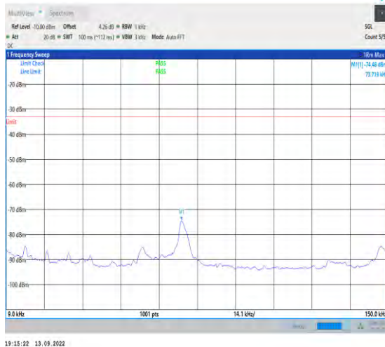
1-N71-15-20-L-1-DFT-PI2BPSK-Inner_1RB_Left-1 @1-0.009-0.15-Ant1-0.04--74.48--33-PASS
