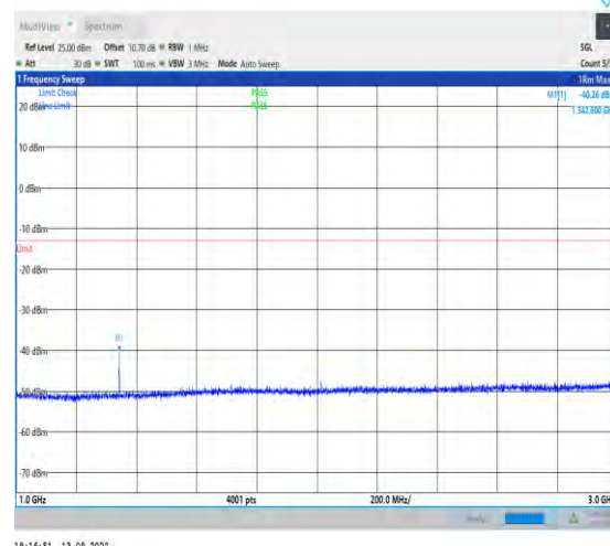
1-N71-15-20-M-1-DFT-PI2BPSK-Inner_1RB_Left-1@ 1-1000-3000-Ant1-1342.00--40.26--13-PASS
