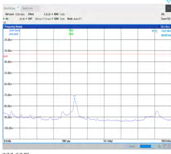
1-N71-15-20-H-1-DFT-PI2BPSK-Inner_1RB_Left-1 @1-0.009-0.15-Ant1-0.04--74.47--33-PASS
