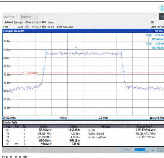
1-N71-15-10-M-9-CP-256QAM-Outet_Full-52@0-An t1-9.289-9.860-≤10-PASS
