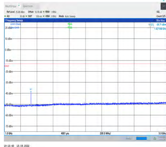
1-N71-15-20-L-1-DFT-PI2BPSK-Inner_1RB_Left-1@ 1-1000-3000-Ant1-1327.00--39.71--13-PASS
