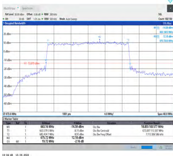
1-N71-15-20-L-6-CP-QPSK-Outer_Full-106@0-Ant1 -18.855-19.720-≤20-PASS
