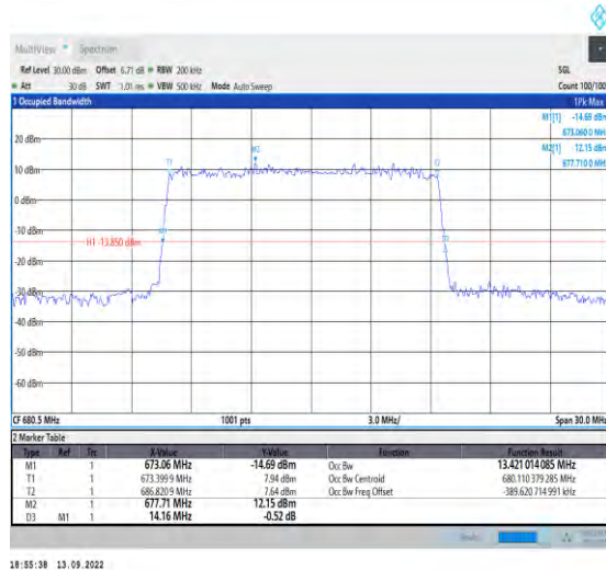
1-N71-15-15-M-5-DFT-256QAM-Outer_Full-75@0-A nt1-13.421-14.160-≤15-PASS
