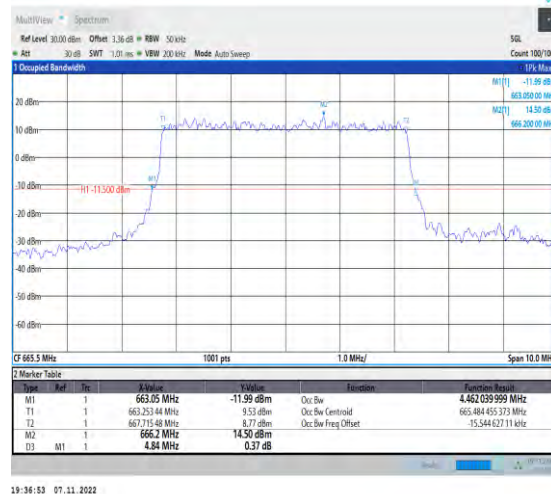
1-N71-15-5-L-4-DFT-64QAM-Outer_Full-25@0-Ant1-4 4.462-4.840-≤5-PASS
