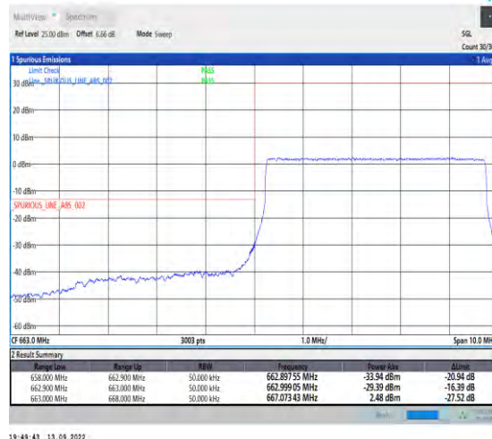
1-N71-15-5-L-6-CP-QPSK-Outer_Full-25@0-Ant1-1--PASS-see graph
