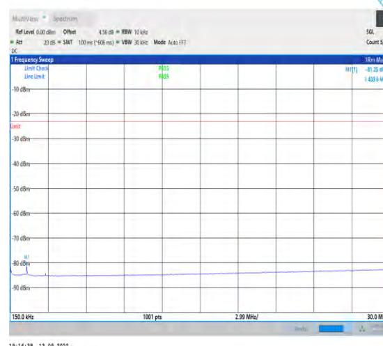
1-N71-15-20-M-1-DFT-PI2BPSK-Inner_1RB_Left-1@ 1-0.15-30-Ant1-0.51--81.25--23-PASS
