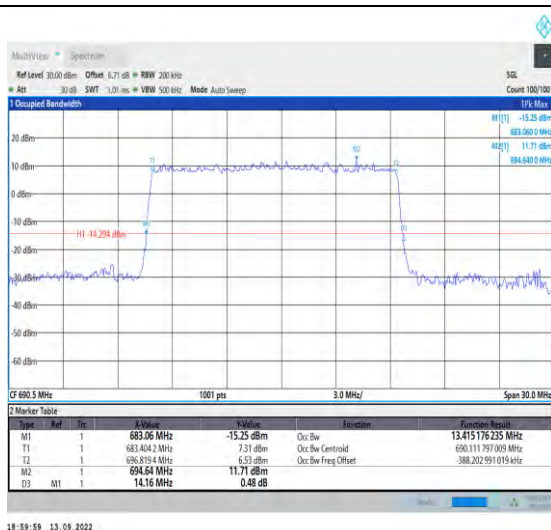
1-N71-15-15-H-5-DFT-256QAM-Outer_Full-75@0-A nt1-13.415-14.160-≤15-PASS
