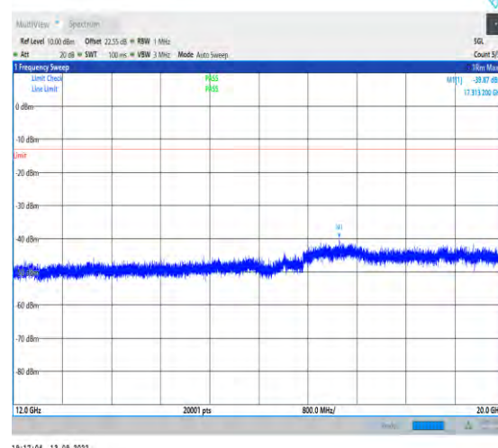
1-N71-15-20-M-1-DFT-PI2BPSK-Inner_1RB_Left-1@ 1-12000-20000-Ant1-17326.80--39.87--13-PASS
