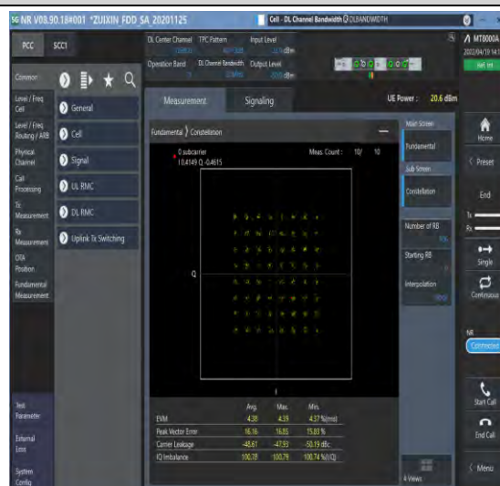
1-N71--15-20-M-8-CP-64QAM-Outer_Full-106@0-A nt1-see graph-PASS
