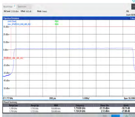
1-N66-PC3-15-15-L-6-CP-QPSK-Outer_Full-79@0-Ant1-1-seegraph-PASS-see graph
