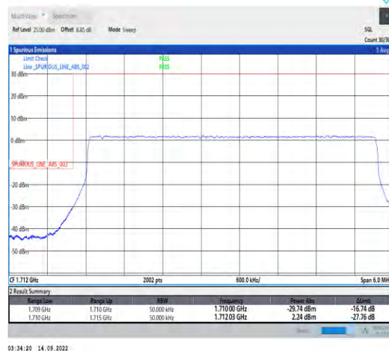
1-N66-PC3-15-5-L-6-CP-QPSK-Outer_Full-25@0-Ant1-1-seegraph-PASS-see graph
