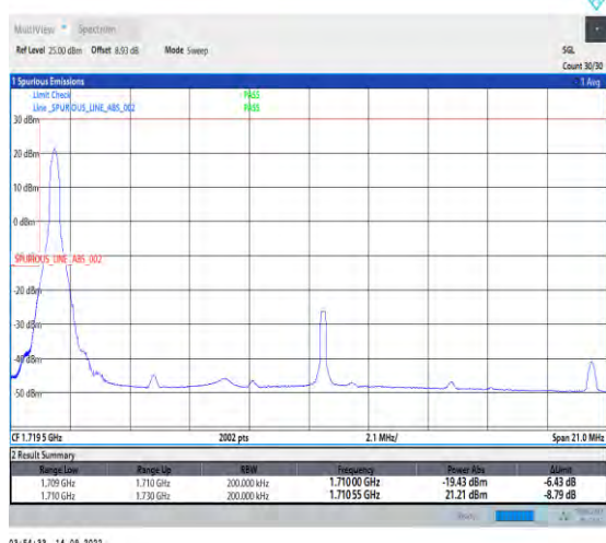
1-N66-PC3-15-20-L-4-CP-QPSK-Edge_1RB_Left-1@0-Ant1-1-seegraph-PASS-see graph
