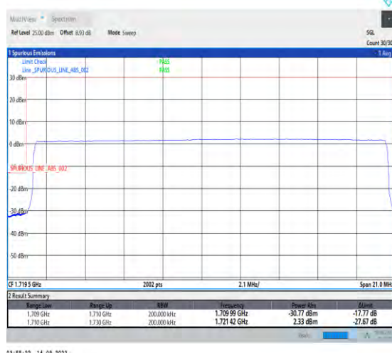
1-N66-PC3-15-20-L-6-CP-QPSK-Outer_Full-106@0-Ant1-1-seegraph-PASS-see graph
