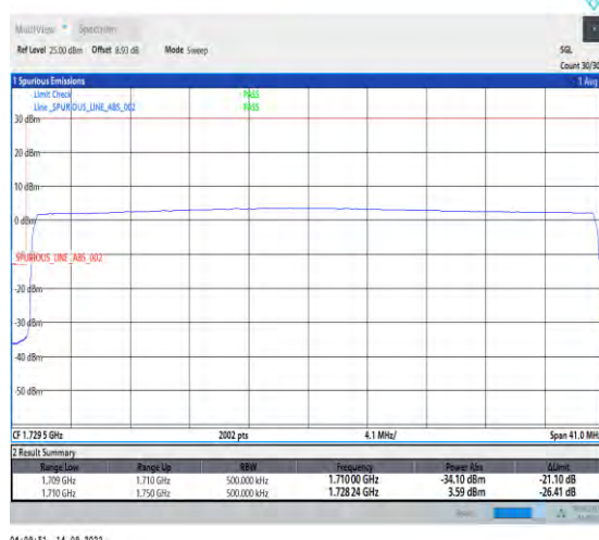
1-N66-PC3-15-40-L-6-CP-QPSK-Outer_Full-216@0-Ant1-1-seegraph-PASS-see graph
