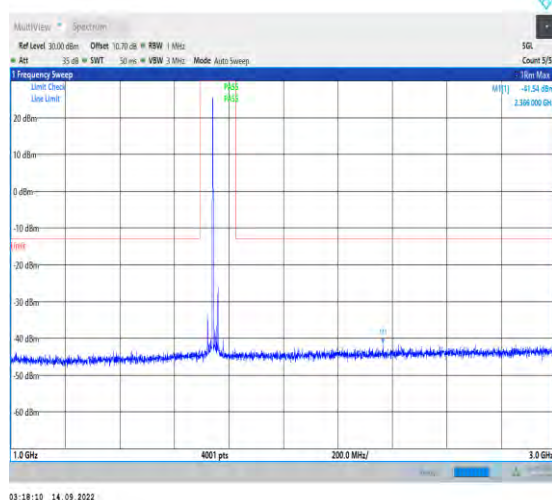
1-N66-PC3-15-40-H-1-DFT-PI2BPSK-Inner_1RB_Lef t-1@1-1000-3000-Ant1-2366.00--41.54--13-PASS
