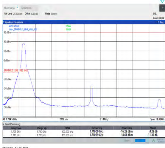
1-N66-PC3-15-10-L-4-CP-QPSK-Edge_1RB_Left-1@0-Ant1-1-seegraph-PASS-see graph
