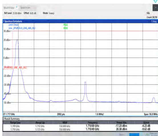
1-N66-PC3-15-15-L-4-CP-QPSK-Edge_1RB_Left-1@0-Ant1-1-seegraph-PASS-see graph
