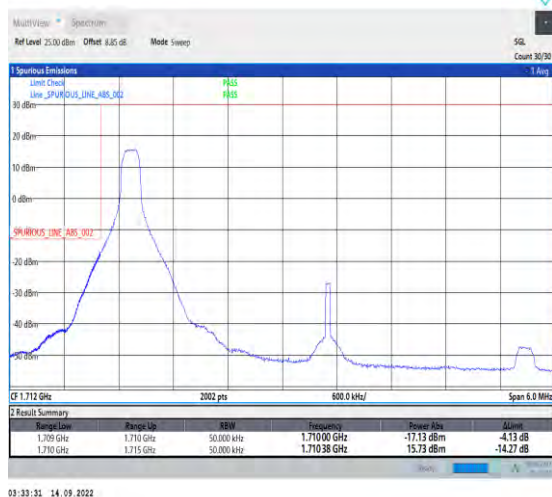
1-N66-PC3-15-5-L-4-CP-QPSK-Edge_1RB_Left-1@0-Ant1-1-seegraph-PASS-see graph
