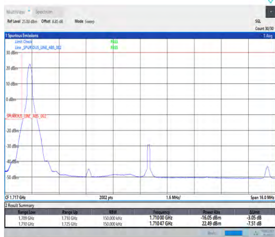
1-N66-PC3-15-15-L-1-DFT-PI2BPSK-Edge_1RB_Left-1@0-Ant1-1-seegraph-PASS-see graph
