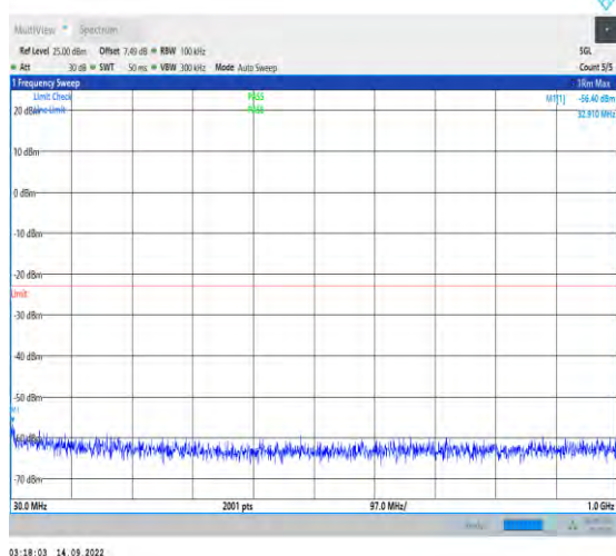
1-N66-PC3-15-40-H-1-DFT-PI2BPSK-Inner_1RB_L eft-1@1-30-1000-Ant1-32.91--56.40--23-PASS
