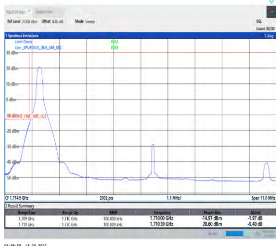
1-N66-PC3-15-10-L-1-DFT-PI2BPSK-Edge_1RB_Left-1@0-Ant1-1-seegraph-PASS-see graph
