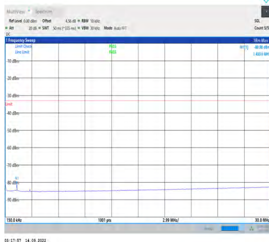
1-N66-PC3-15-40-H-1-DFT-PI2BPSK-Inner_1RB_Lef t-1@1-0.15-30-Ant1-1.43--80.98--33-PASS
