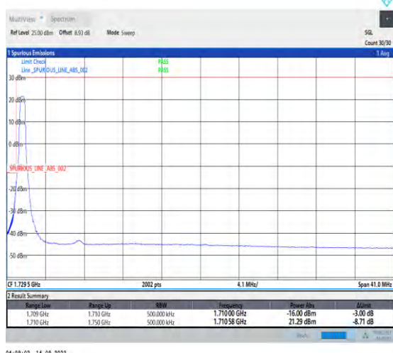
1-N66-PC3-15-40-L-4-CP-QPSK-Edge_1RB_Left-1@0-Ant1-1-seegraph-PASS-see graph
