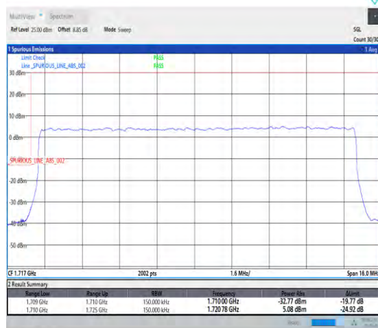
1-N66-PC3-15-15-L-3-DFT-PI2BPSK-Outer_Full-75@0-Ant1-1-seegraph-PASS-see graph
