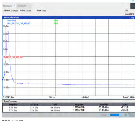
1-N66-PC3-15-40-L-1-DFT-PI2BPSK-Edge_1RB_Left-1@0-Ant1-1-seegraph-PASS-see graph
