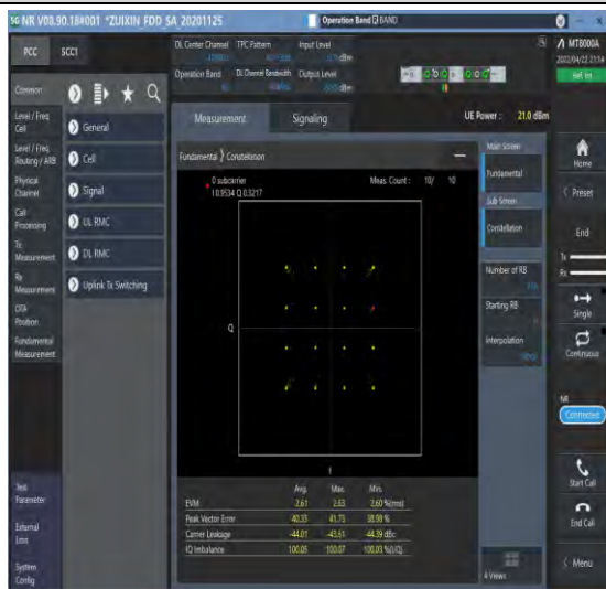
1-N66-PC3-15-40-M-3-DFT-16QAM-Outer_Full-216@ 0-Ant1-see graph-PASS
