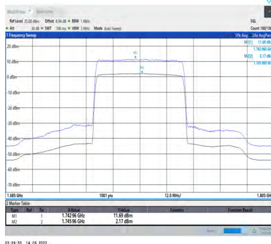
1-N66-PC3-15-40-M-2-CP-256QAM-Outer_Full-216 @0-Ant1-9.52-100%-0.00-9.52-PASS<13
