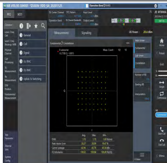
1-N66-PC3-15-40-M-4-DFT-64QAM-Outer_Full-216 @0-Ant1-see graph-PASS
