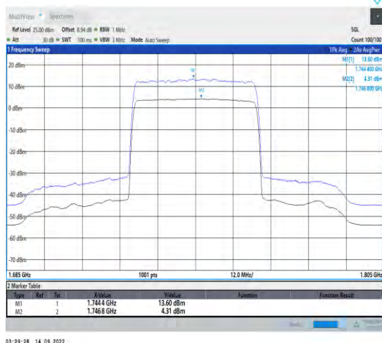
1-N66-PC3-15-40-M-1-DFT-256QAM-Outer_Full-216 @0-Ant1-9.29-100%-0.00-9.29-PASS<13
