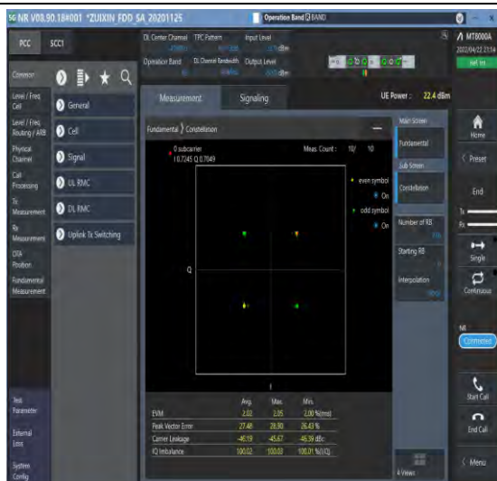
1-N66-PC3-15-40-M-1-DFT-PI2BPSK-Outer_Full-216 @0-Ant1-see graph-PASS
