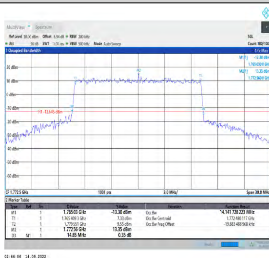
1-N66-PC3-15-15-H-8-CP-64QAM-Outer_Full-79@0 -Ant1-14.142-14.850-≤15-PASS
