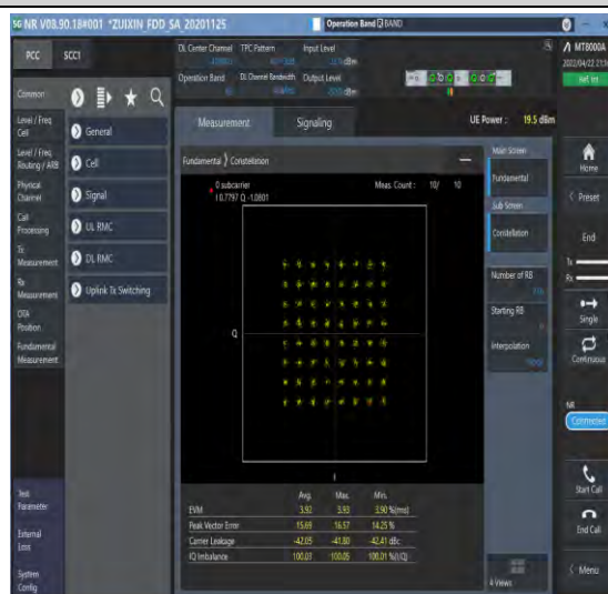
1-N66-PC3-15-40-M-8-CP-64QAM-Outer_Full-216@0-Ant1-see graph-PASS
