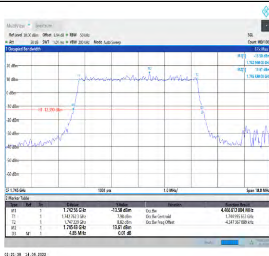
1-N66-PC3-15-5-M-3-DFT-16QAM-Outer_Full-25@0-Ant1-4.467-4.850-≤5-PASS
