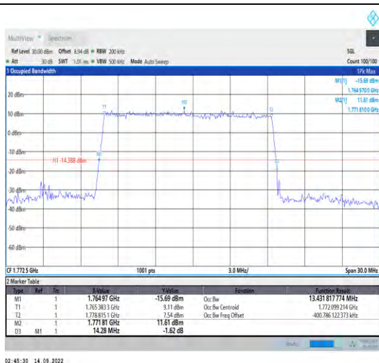
1-N66-PC3-15-15-H-5-DFT-256QAM-Outer_Full-75 @0-Ant1-13.432-14.280-≤15-PASS
