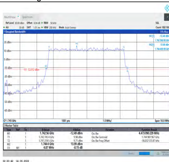
1-N66-PC3-15-5-M-1-DFT-QPSK-Outer_Full-25@0-Ant1-4.473-4.870-≤5-PASS
