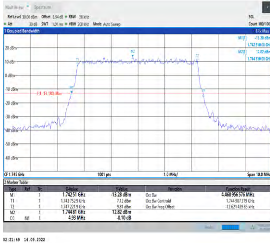
1-N66-PC3-15-5-M-4-DFT-64QAM-Outer_Full-25@0-Ant1-4.469-4.930-≤5-PASS
