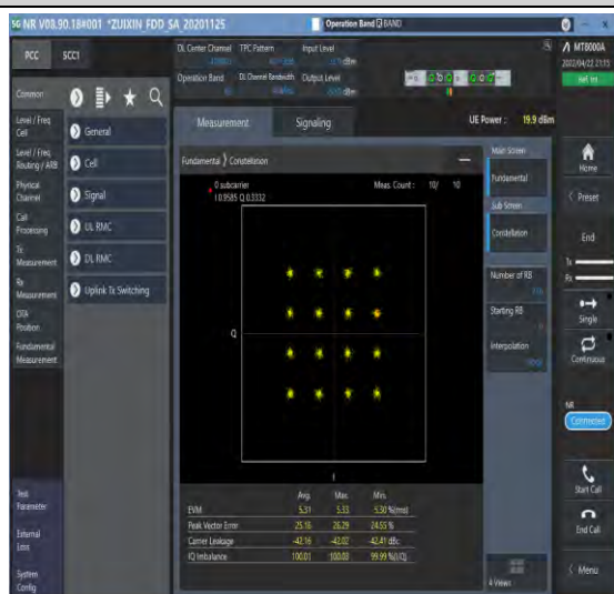
1-N66-PC3-15-40-M-7-CP-16QAM-Outer_Full-216@0-Ant1-see graph-PASS
