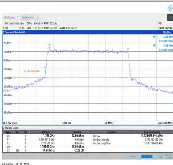
1-N66-PC3-15-15-H-7-CP-16QAM-Outer_Full-79@0 -Ant1-14.126-14.940-≤15-PASS
