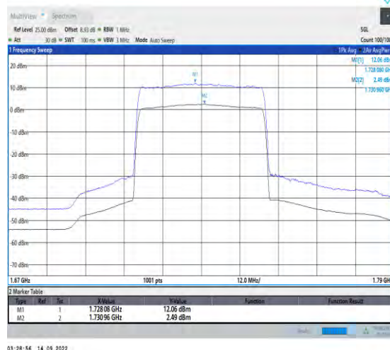
1-N66-PC3-15-40-L-2-CP-256QAM-Outer_Full-216 @0-Ant1-9.57-100%-0.00-9.57-PASS<13
