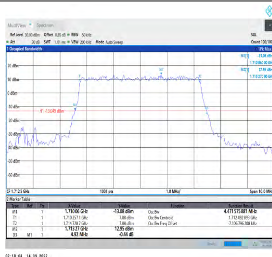
1-N66-PC3-15-5-L-2-DFT-PI2BPSK-Outet_Full-25@ 0-Ant1-4.472-4.920-≤5-PASS
