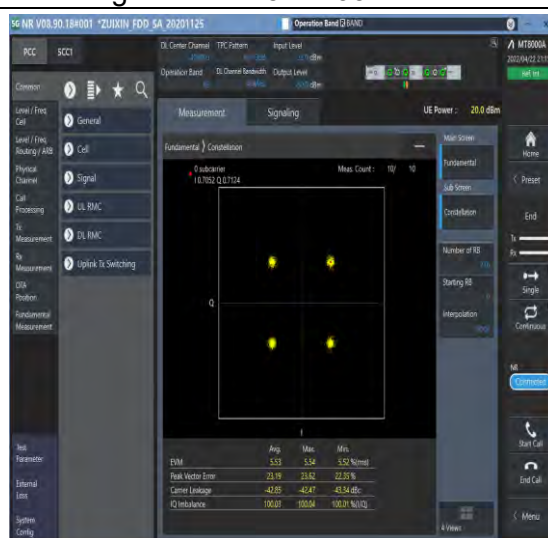
1-N66-PC3-15-40-M-6-CP-QPSK-Outer_Full-216@0-Ant1-see graph-PASS
