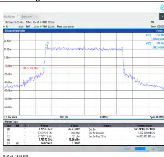
1-N66-PC3-15-15-H-6-CP-QPSK-Outer_Full-79@0- Ant1-14.125-14.820-≤15-PASS
