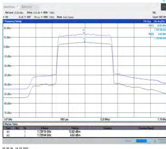
1-N66-PC3-15-40-L-1-DFT-256QAM-Outer_Full-216 @0-Ant1-9.19-100%-0.00-9.19-PASS<13
