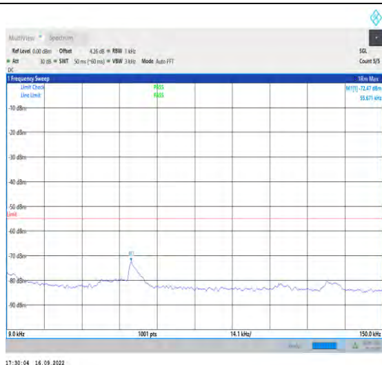
1-N41-PC2-30-100-L-1-DFT-PI2BPSK-Inner_1RB_L eft-1@1-0.009-0.15-Ant1-0.06--72.47--55-PASS
