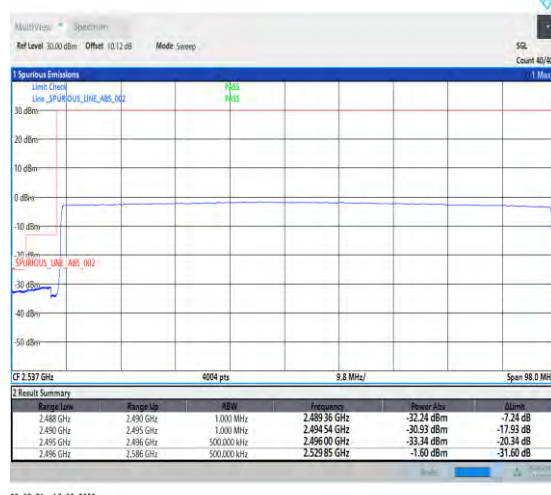
1-N41-PC2-30-90-L-6-CP-QPSK-Outer_Full-245@0-Ant1-1--PASS-see graph
