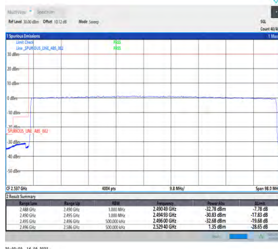
1-N41-PC2-30-90-L-3-DFT-PI2BPSK-Outer_Full-243@0-Ant1-1--PASS-see graph
