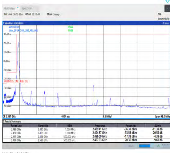
1-N41-PC2-30-90-L-4-CP-QPSK-Edge_1RB_Left-1@0-Ant1-1--PASS-see graph
