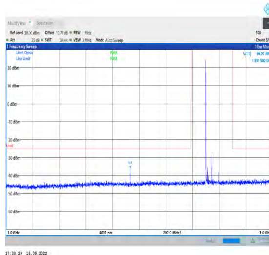
1-N41-PC2-30-100-L-1-DFT-PI2BPSK-Inner_1RB_Le ft-1@1-1000-3000-Ant1-1931.50--36.07--25-PASS
