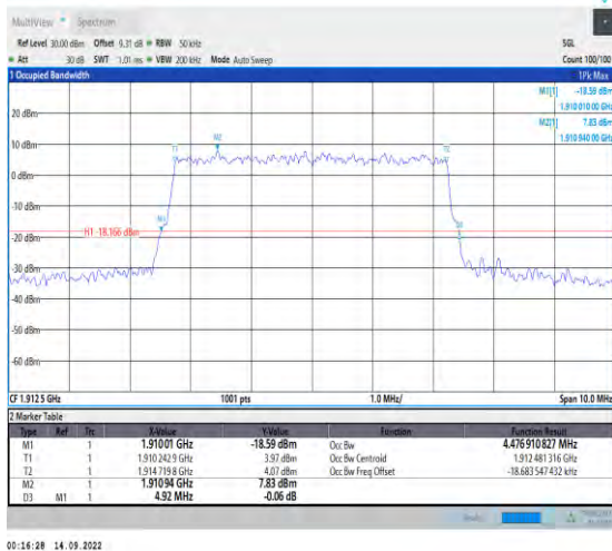
1-N25-PC3-15-5-H-9-CP-256QAM-Outer_Full-25@0- -Ant1-4.477-4.920-≤5-PASS
