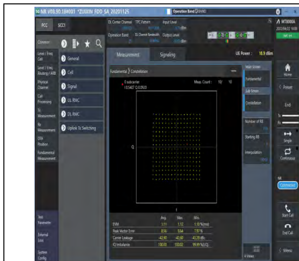
1-N25--15-40-M-5-DFT-256QAM-Outer_Full-216@0-A nt1-see graph-PASS
