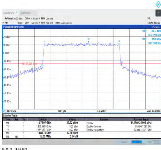
1-N25-PC3-15-15-M-8-CP-64QAM-Outet_Full-79@0-Ant1-14.15-15.060-≤15-PASS
