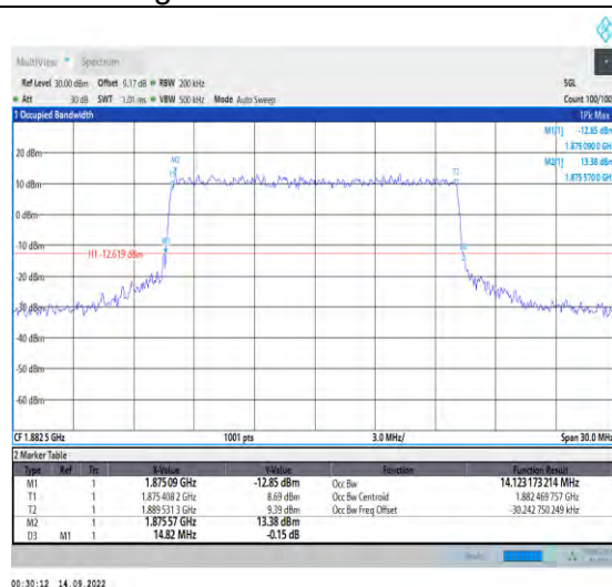
1-N25-PC3-15-15-M-7-CP-16QAM-Outet_Full-79@0-Ant1-14.123-14.820-≤15-PASS
