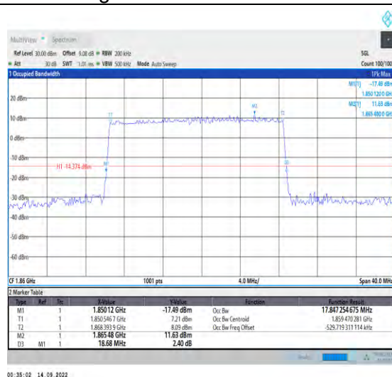
1-N25-PC3-15-20-L-5-DFT-256QAM-Outer_Full-100 @0-Ant1-17.847-18.680-≤20-PASS
