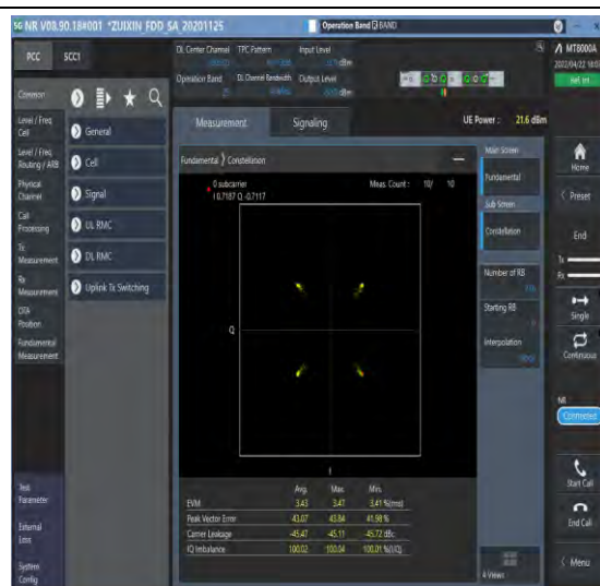
1-N25--15-40-M-2-DFT-QPSK-Outer_Full-216@0-An t1-see graph-PASS
