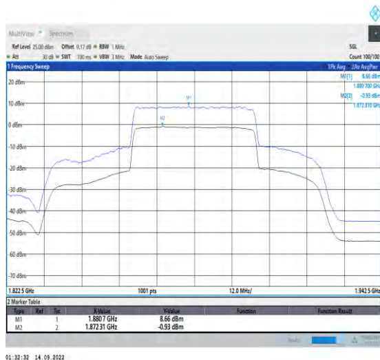
1-N25-PC3-15-40-M-1-DFT-256QAM-Outer_Full-216 @0-Ant1-9.59-100%-0.00-9.59-PASS-≤13
