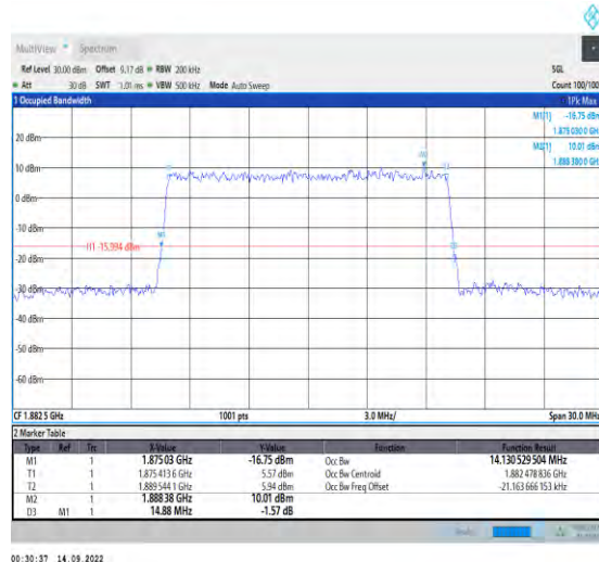
1-N25-PC3-15-15-M-9-CP-256QAM-Outet_Full-79@0-Ant1-14.131-14.880-≤15-PASS
