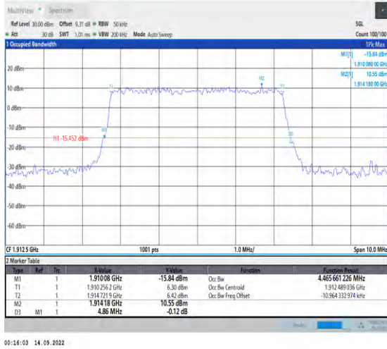
1-N25-PC3-15-5-H-7-CP-16QAM-Outer_Full-25@0- Ant1-4.466-4.860-≤5-PASS
