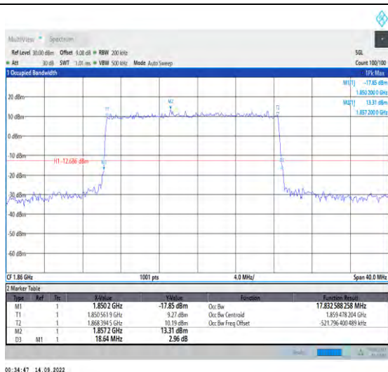
1-N25-PC3-15-20-L-4-DFT-64QAM-Outer_Full-100 @0-Ant1-17.833-18.640-≤20-PASS
