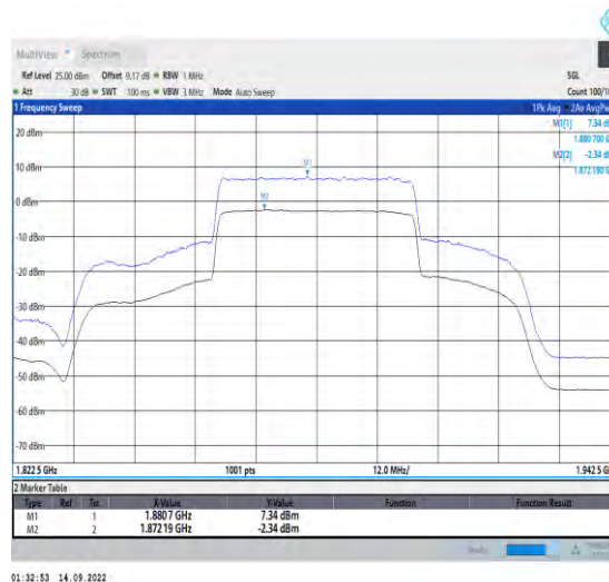
1-N25-PC3-15-40-M-2-CP-256QAM-Outer_Full-216 @0-Ant1-9.68-100%-0.00-9.68-PASS-≤13
