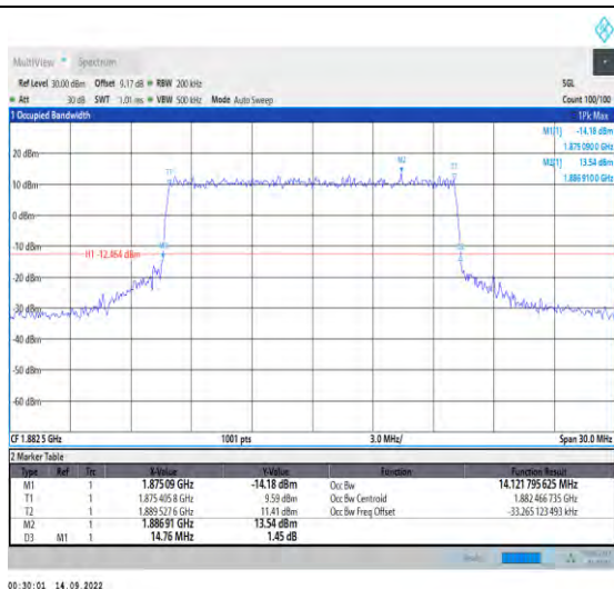
1-N25-PC3-15-15-M-6-CP-QPSK-Outet_Full-79@0-Ant1-14.122-14.760-≤15-PASS
