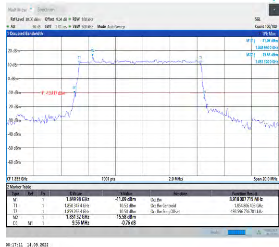
1-N25-PC3-15-10-L-1-DFT-QPSK-Outer_Full-50@0- Ant1-8.918-9.560-≤10-PASS
