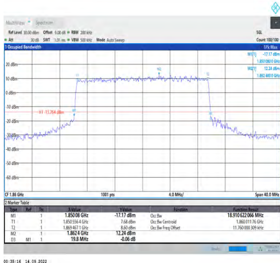
1-N25-PC3-15-20-L-6-CP-QPSK-Outer_Full-106@0-Ant1-18.911-19.800-≤20-PASS
