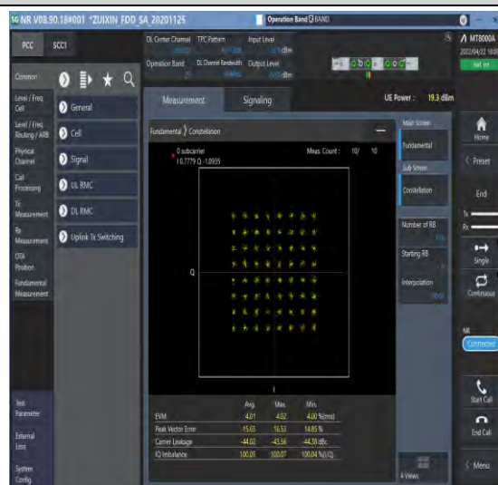
1-N25--15-40-M-8-CP-64QAM-Outer_Full-216@0-A nt1-see graph-PASS
