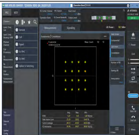
1-N25--15-40-M-7-CP-16QAM-Outer_Full-216@0-Ant 1-see graph-PASS
