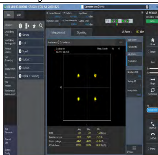
1-N25--15-40-M-6-CP-QPSK-Outer_Full-216@0-Ant 1-see graph-PASS
