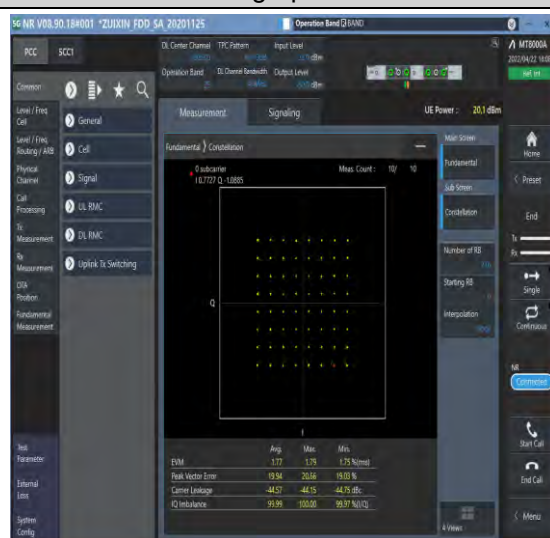
1-N25--15-40-M-4-DFT-64QAM-Outer_Full-216@0- Ant1-see graph-PASS
