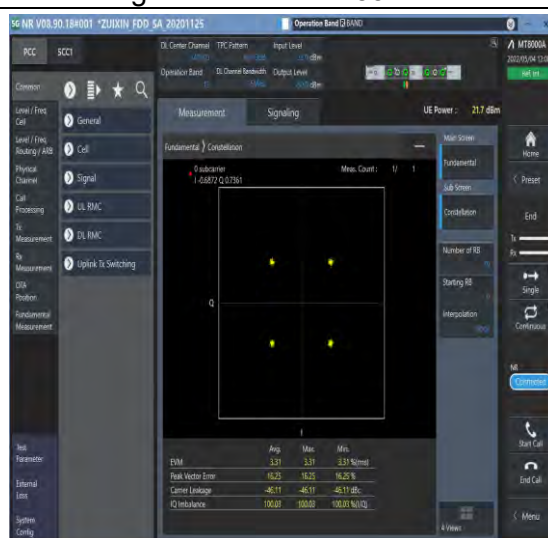
1-N12-PC3-15-15-M-6-CP-QPSK-Outer_Full-79@0-Ant1-see graph-PASS
