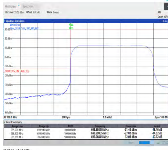
1-N12-PC3-15-5-L-6-CP-QPSK-Outer_Full-25@0-Ant1-1--PASS-see graph
