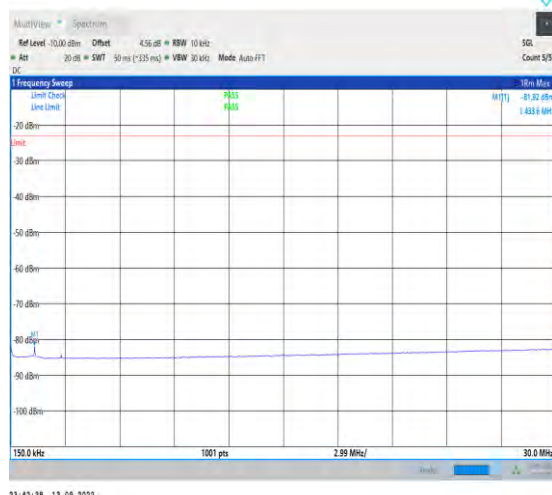
1-N12-PC3-15-15-H-1-DFT-PI2BPSK-Inner_1RB_Lef t-1@1-0.15-30-Ant1-1.43--81.92--23-PASS
