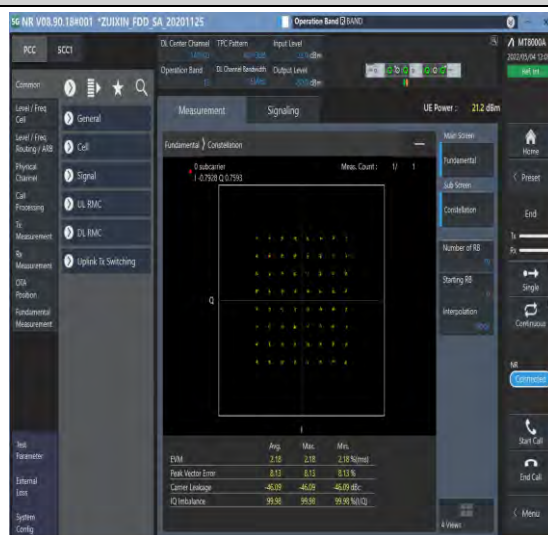
1-N12-PC3-15-15-M-8-CP-64QAM-Outer_Full-79@0-Ant1-see graph-PASS
