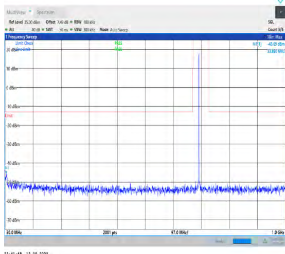
1-N12-PC3-15-15-M-1-DFT-PI2BPSK-Inner_1RB_L eft-1@1-30-1000-Ant1-33.88--45.69--13-PASS
