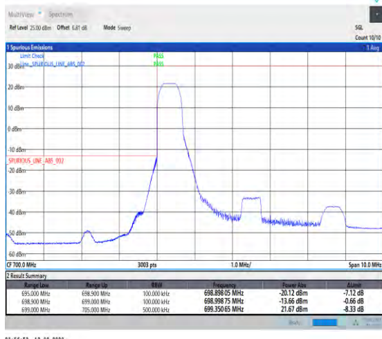
1-N12-PC3-15-5-L-4-CP-QPSK-Edge_1RB_Left-1@0-Ant1-1--PASS-see graph
