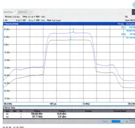
1-N12-PC3-15-15-M-2-CP-256QAM-Outer_Full-79@0 -Ant1-10.12-100%-0.00-10.12-PASS-≤13
