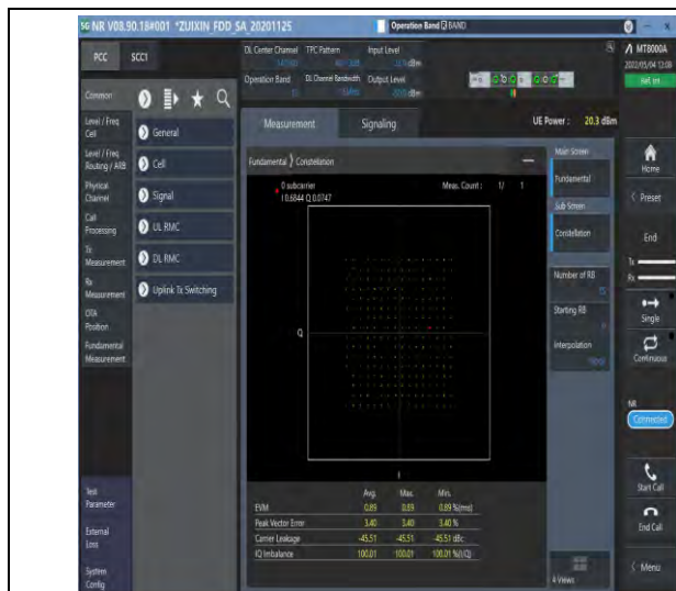
1-N12-PC3-15-15-M-5-DFT-256QAM-Outer_Full-75@0-Ant1-see graph-PASS
