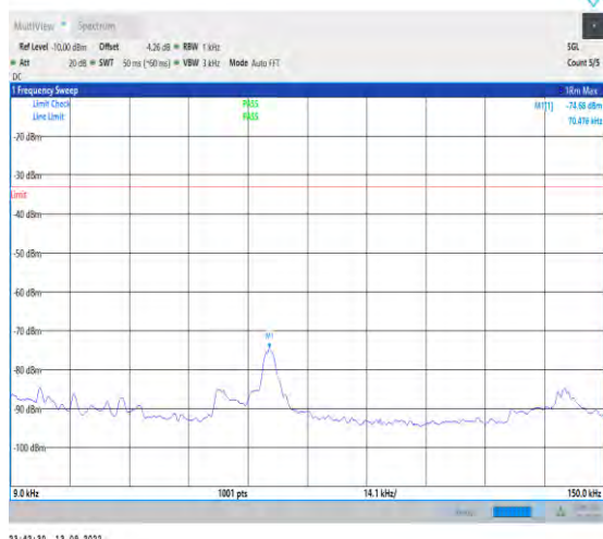
1-N12-PC3-15-15-H-1-DFT-PI2BPSK-Inner_1RB_L eft-1@1-0.009-0.15-Ant1-0.07--74.68--33-PASS
