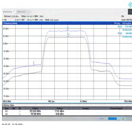
1-N12-PC3-15-15-M-1-DFT-256QAM-Outer_Full-75 @0-Ant1-9.01-100%-0.00-9.01-PASS-≤13
