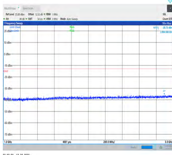
1-N12-PC3-15-15-H-1-DFT-PI2BPSK-Inner_1RB_Lef t-1@1-1000-3000-Ant1-2894.50--35.73--13-PASS
