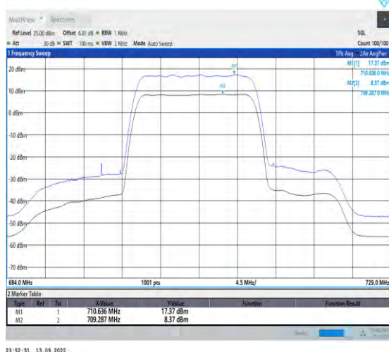
1-N12-PC3-15-15-L-1-DFT-256QAM-Outer_Full-75@ 0-Ant1-9.00-100%-0.00-9.00-PASS-≤13
