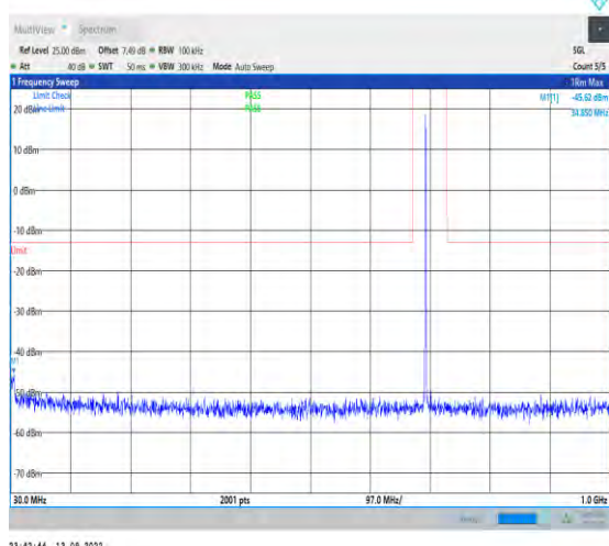
1-N12-PC3-15-15-H-1-DFT-PI2BPSK-Inner_1RB_L eft-1@1-30-1000-Ant1-34.85--45.62--13-PASS
