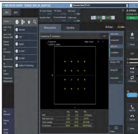
1-N12-PC3-15-15-M-7-CP-16QAM-Outer_Full-79@0-Ant1-see graph-PASS
