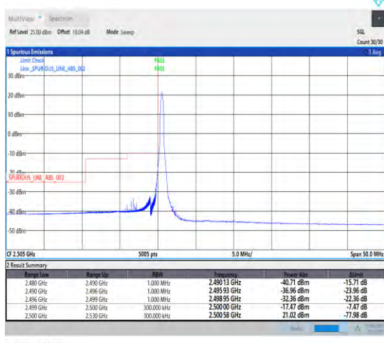
1-N7-PC3-15-20-L-4-CP-QPSK-Edge_1RB_Left-1@0-Ant1-1--PASS-see graph
