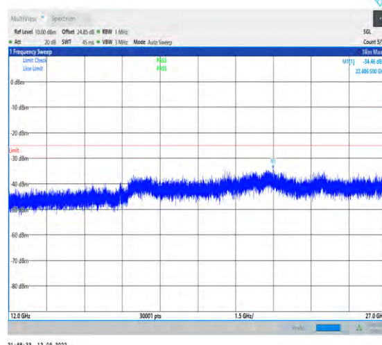
1-N7-PC3-15-40-M-1-DFT-PI2BPSK-Inner_1RB_Left- 1@1-12000-27000-Ant1-22486.50--34.46--25-PASS
