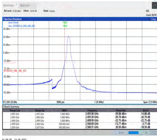
1-N7-PC3-15-5-L-1-DFT-PI2BPSK-Edge_1RB_Left-1@ 0-Ant1-1--PASS-see graph
