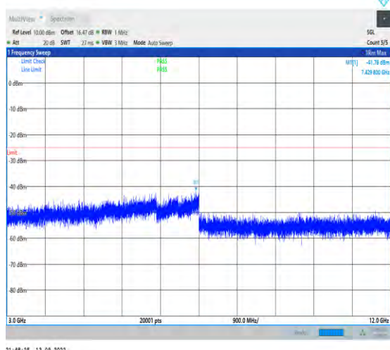
1-N7-PC3-15-40-M-1-DFT-PI2BPSK-Inner_1RB_Lef t-1@1-3000-12000-Ant1-7429.80--41.78--25-PASS
