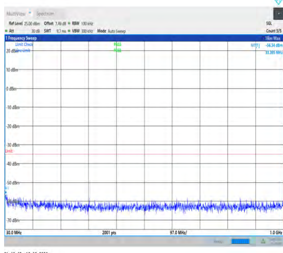
1-N7-PC3-15-40-H-1-DFT-PI2BPSK-Inner_1RB_Lef t-1@1-30-1000-Ant1-33.40--56.34--35-PASS
