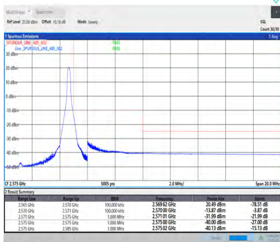
1-N7-PC3-15-5-H-2-DFT-PI2BPSK-Edge_1RB_Right-1 @24-Ant1-1--PASS-see graph
