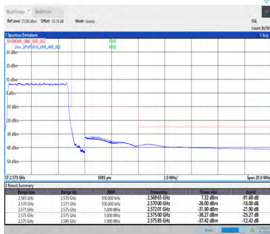
1-N7-PC3-15-5-H-3-DFT-PI2BPSK-Outer_Full-25 @0-Ant1-1--PASS-see graph
