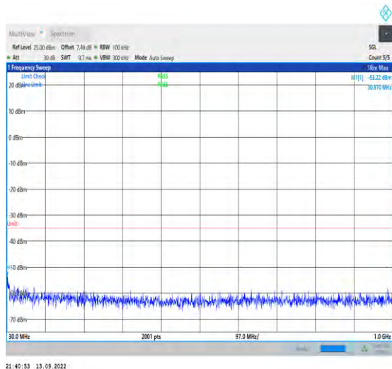
1-N7-PC3-15-40-L-1-DFT-PI2BPSK-Inner_1RB_Left -1@1-30-1000-Ant1-30.00--53.22--35-PASS
