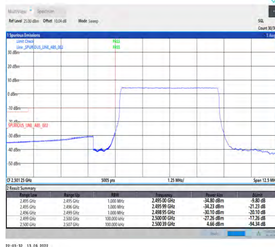
1-N7-PC3-15-5-L-6-CP-QPSK-Outer_Full-25@0-A nt1-1--PASS-see graph
