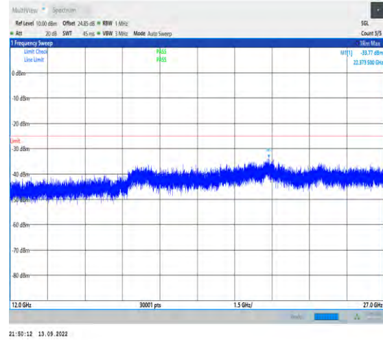
1-N7-PC3-15-40-H-1-DFT-PI2BPSK-Inner_1RB_Left- 1@1-12000-27000-Ant1-22373.50--33.77--25-PASS
