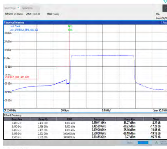
1-N7-PC3-15-20-L-6-CP-QPSK-Outer_Full-106@0-Ant1-1--PASS-see graph
