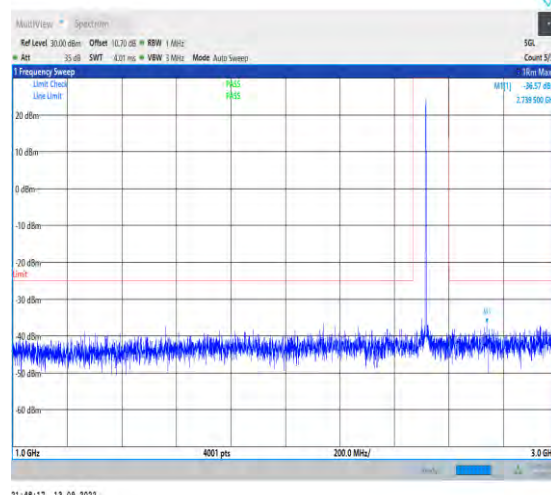
1-N7-PC3-15-40-M-1-DFT-PI2BPSK-Inner_1RB_Left- 1@1-1000-3000-Ant1-2739.50--36.57--25-PASS
