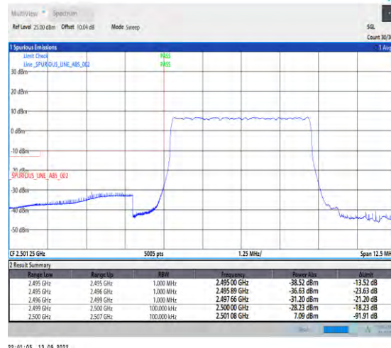
1-N7-PC3-15-5-L-3-DFT-PI2BPSK-Outer_Full-25 @0-Ant1-1--PASS-see graph
