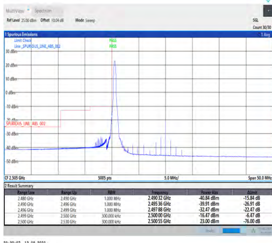
1-N7-PC3-15-20-L-1-DFT-PI2BPSK-Edge_1RB_Left-1 @0-Ant1-1--PASS-see graph
