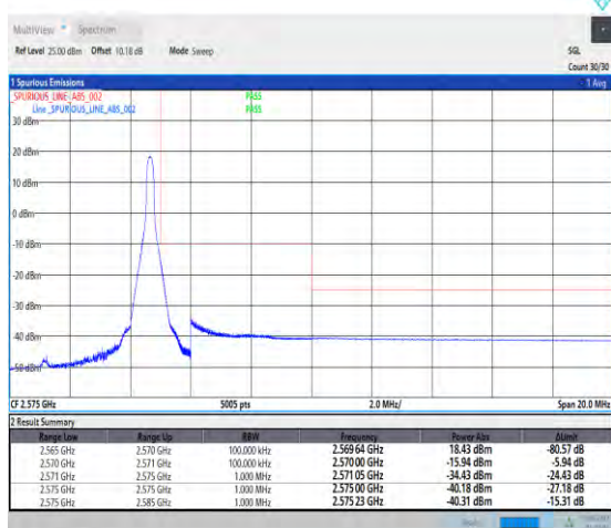
1-N7-PC3-15-5-H-5-CP-QPSK-Edge_1RB_Right-1@2 4-Ant1-1--PASS-see graph
