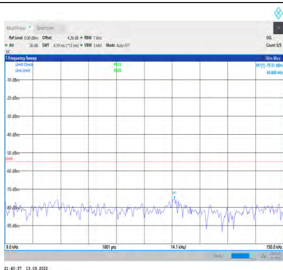
1-N7-PC3-15-40-L-1-DFT-PI2BPSK-Inner_1RB_Left -1@1-0.009-0.15-Ant1-0.13--75.51--55-PASS
