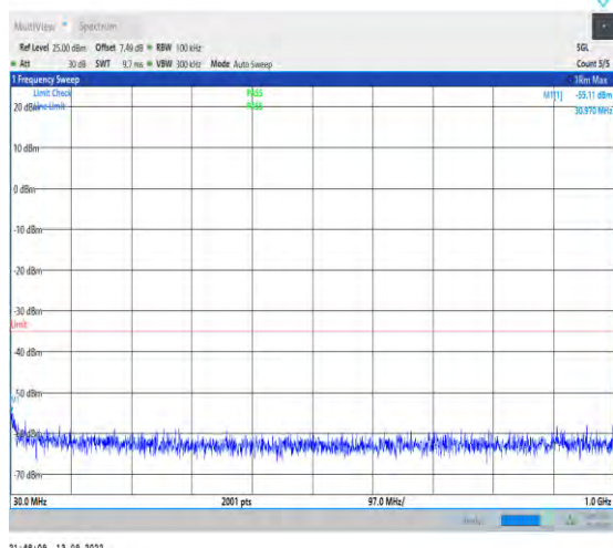
1-N7-PC3-15-40-M-1-DFT-PI2BPSK-Inner_1RB_Lef t-1@1-30-1000-Ant1-30.97--55.11--35-PASS
