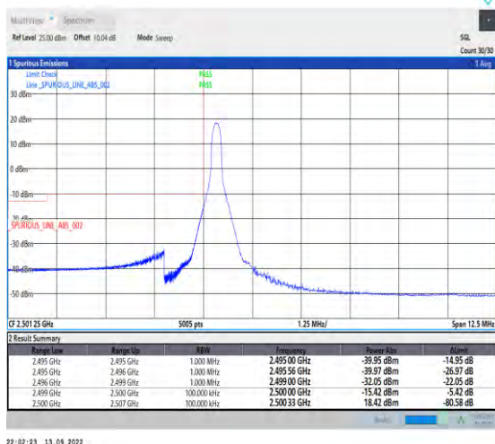
1-N7-PC3-15-5-L-4-CP-QPSK-Edge_1RB_Left-1@0-A nt1-1--PASS-see graph
