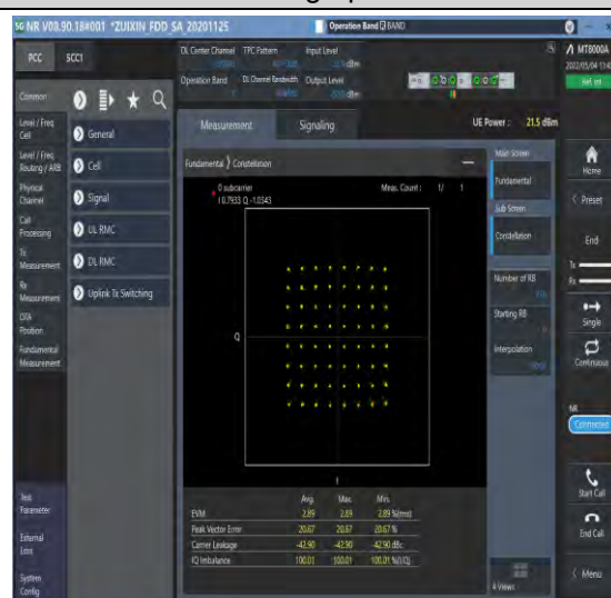
1-N7-PC3-15-40-M-4-DFT-64QAM-Outter_Full-216@0 0-Ant1-see graph-PASS
