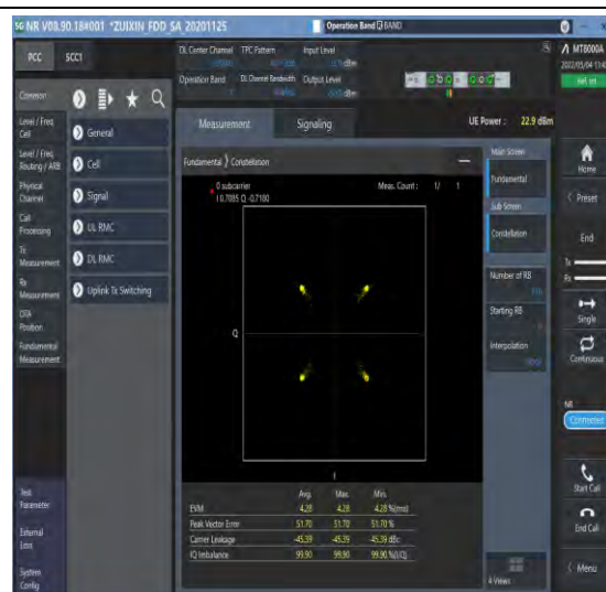
1-N7-PC3-15-40-M-2-DFT-QPSK-Outter_Full-216@0 -Ant1-see graph-PASS
