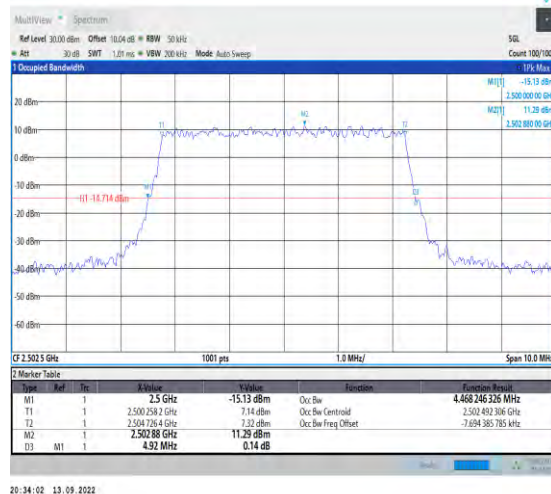
1-N7-PC3-15-5-L-4-DFT-64QAM-Outer_Full-25@0-A nt1-4.468-4.920-≤5-PASS
