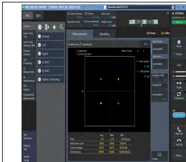
1-N7-PC3-15-40-M-1-DFT-PI2BPSK-Outter_Full-216@ 0-Ant1-see graph-PASS
