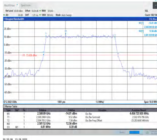
1-N7-PC3-15-5-L-2-DFT-PI2BPSK-Outer_Full-25@0 -Ant1-4.457-4.810-≤5-PASS
