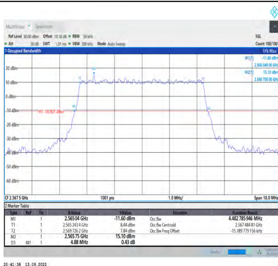
1-N7-PC3-15-5-H-1-DFT-QPSK-Outer_Full-25@0-A nt1-4.483-4.880-≤5-PASS
