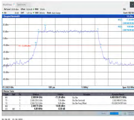
1-N7-PC3-15-5-L-1-DFT-QPSK-Outer_Full-25@0-An t1-4.483-4.890-≤5-PASS
