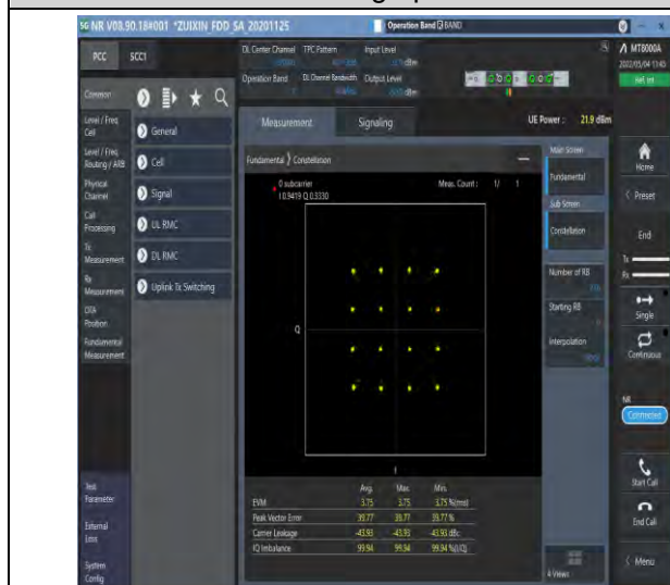
1-N7-PC3-15-40-M-3-DFT-16QAM-Outter_Full-216@0 -Ant1-see graph-PASS
