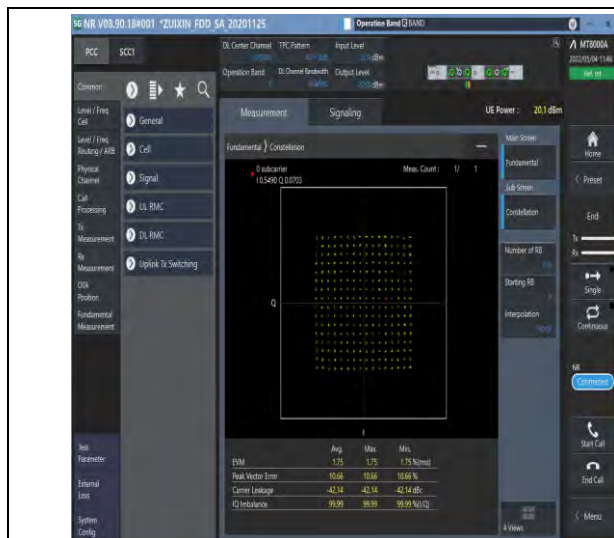
1-N7-PC3-15-40-M-5-DFT-256QAM-Outer_Full-216@ 0-Ant1-see graph-PASS
