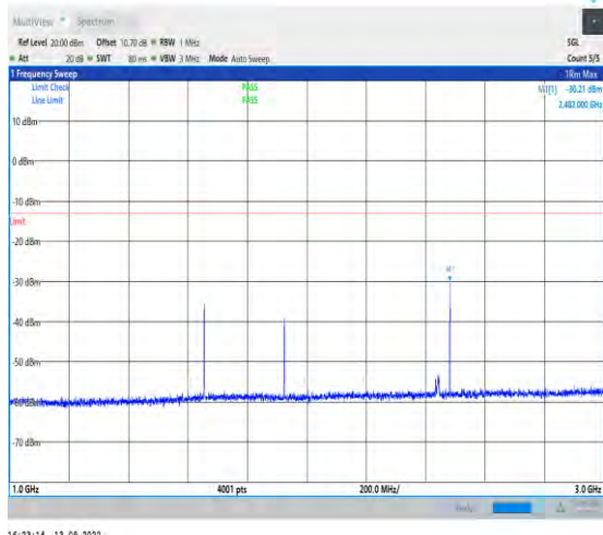
1-N5-PC3-15-20-M-1-DFT-PI2BPSK-Inner_1RB_Left -1@1-1000-3000-Ant1-2481.50--30.21--13-PASS
