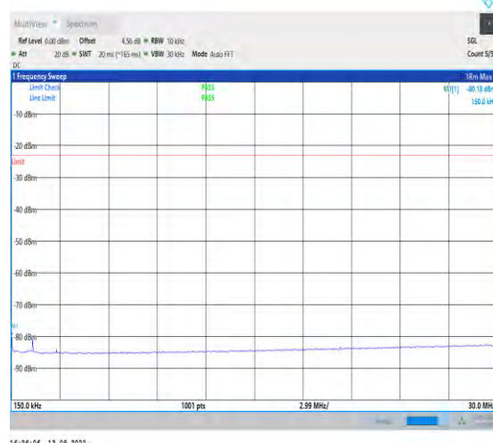
1-N5-PC3-15-20-H-1-DFT-PI2BPSK-Inner_1RB_Left -1@1-0.15-30-Ant1-0.51--80.18--23-PASS
