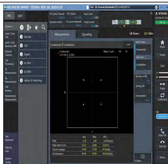
1-N5--15-20-M-2-DFT-QPSK-Outter_Full-100@0-Ant 1-see graph-PASS
