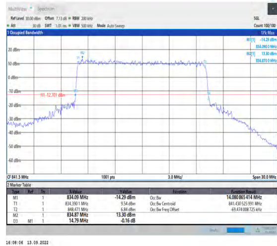
1-N5-PC3-15-15-H-6-CP-QPSK-Outer_Full-79@0-Ant1-14.081-14.790-≤15-PASS
