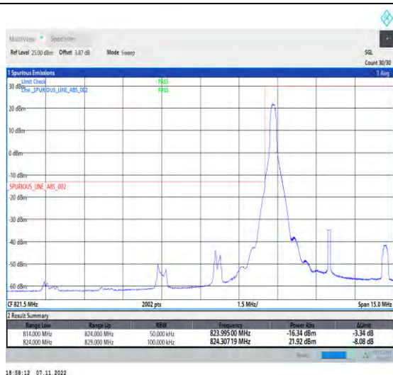
1-N5-PC3-15-5-L-1-DFT-PI2BPSK-Edge_1RB_Left-1 @0-Ant1-1-seegraph-PASS-see graph
