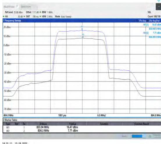
1-N5-PC3-15-20-L-1-DFT-256QAM-Outer_Full-100@ 0-Ant1-8.76-100%-0.00-8.76-PASS-≤13
