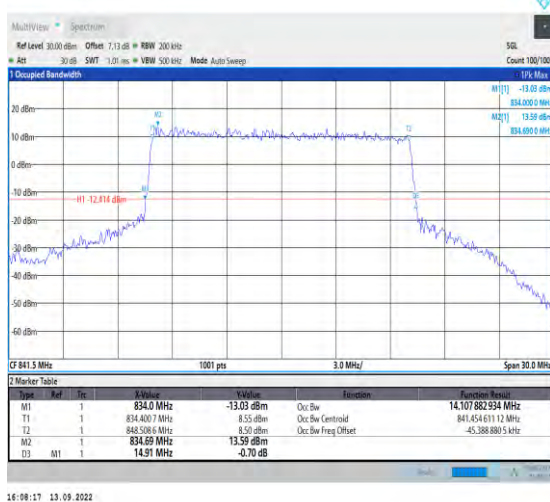
1-N5-PC3-15-15-H-7-CP-16QAM-Outer_Full-79@0-Ant1-14.108-14.910-≤15-PASS
