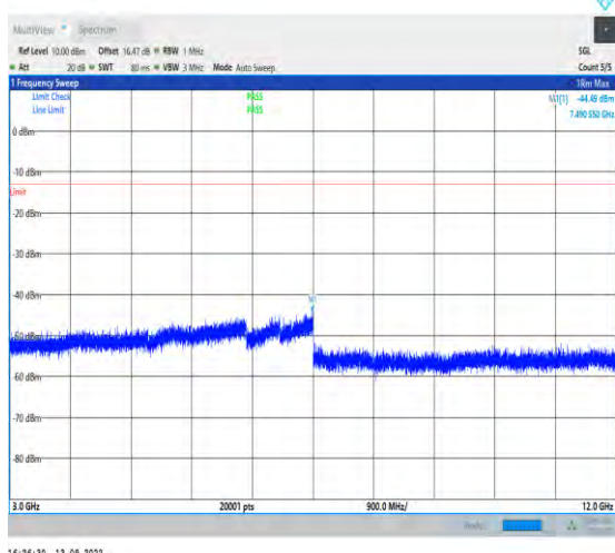
1-N5-PC3-15-20-H-1-DFT-PI2BPSK-Inner_1RB_Left -1@1-3000-12000-Ant1-7488.30--44.49--13-PASS
