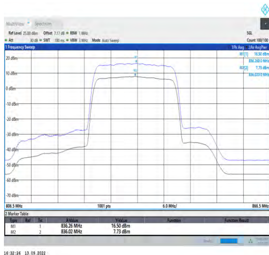
1-N5-PC3-15-20-M-1-DFT-256QAM-Outer_Full-100@ 0-Ant1-8.77-100%-0.00-8.77-PASS-≤13
