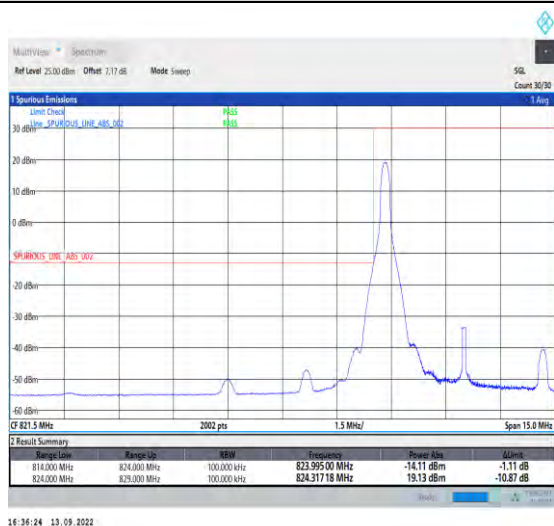
1-N5-PC3-15-5-L-4-CP-QPSK-Edge_1RB_Left-1@0-A nt1-1-seegraph-PASS-see graph
