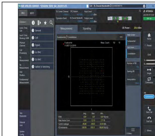
1-N5--15-20-M-5-DFT-256QAM-Outer_Full-100@0-Ant t1-see graph-PASS
