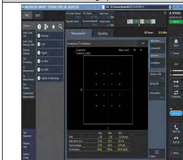
1-N5--15-20-M-3-DFT-16QAM-Outter_Full-100@0-Ant 1-see graph-PASS
