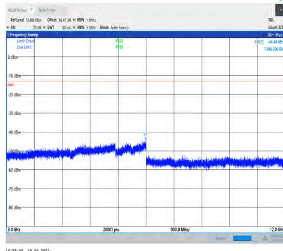
1-N5-PC3-15-20-M-1-DFT-PI2BPSK-Inner_1RB_Left -1@1-3000-12000-Ant1-7355.10--44.40--13-PASS
