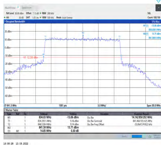
1-N5-PC3-15-15-H-8-CP-64QAM-Outer_Full-79@0-Ant1-14.143-14.850-≤15-PASS
