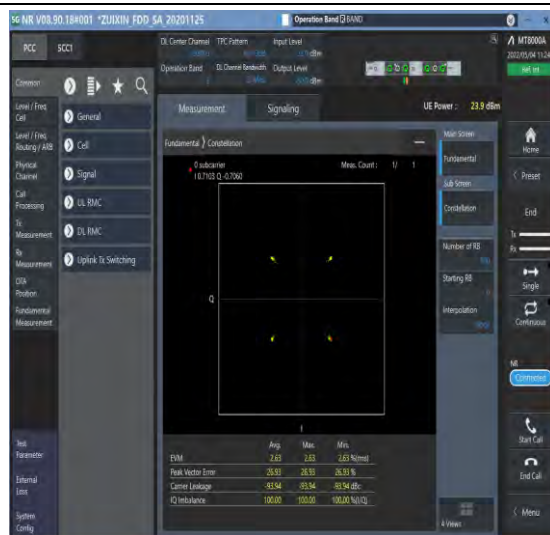
1-N2-PC3-15-20-M-2-DFT-QPSK-Outer_Full-100@0 -Ant1-see graph-PASS
