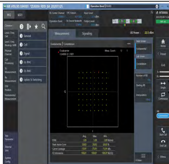
1-N2-PC3-15-20-M-4-DFT-64QAM-Outer_Full-100@ 0-Ant1-see graph-PASS
