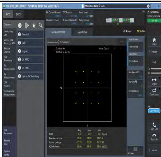
1-N2-PC3-15-20-M-3-DFT-16QAM-Outer_Full-100@0 -Ant1-see graph-PASS
