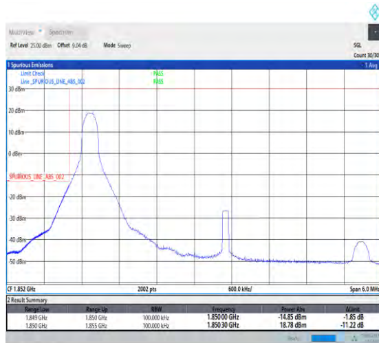
1-N2-PC3-15-5-L-1-DFT-PI2BPSK-Edge_1RB_Left-1 @0-Ant1-1-seegraph-PASS-see graph
