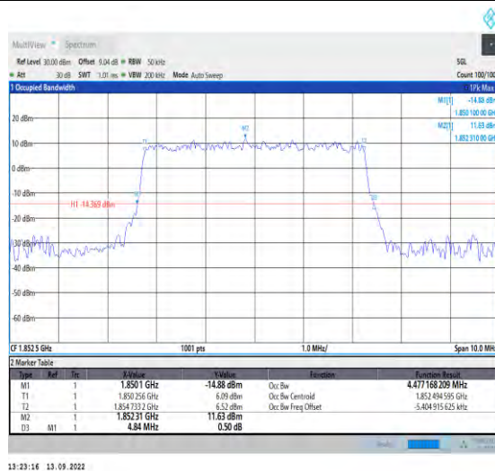
1-N2-PC3-15-5-L-4-DFT-64QAM-Outet_Full-25@0-A nt1-4.477-4.840-<math>\leq 5</math>-PASS
