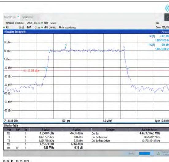
1-N2-PC3-15-5-L-2-DFT-PI2BPSK-Outet_Full-25@0 -Ant1-4.472-4.850-<math>\leq 5</math>-PASS
