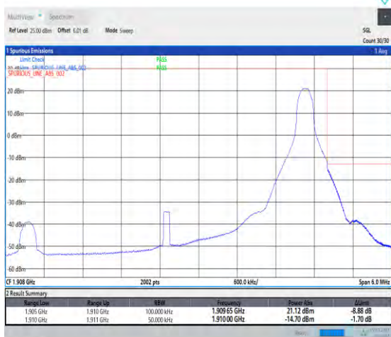
1-N2-PC3-15-5-H-2-DFT-PI2BPSK-Edge_1RB_Right-1 @24-Ant1-1-seegraph-PASS-see graph
