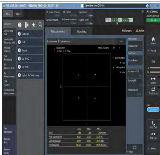
1-N2-PC3-15-20-M-1-DFT-PI2BPSK-Outer_Full-100@ 0-Ant1-see graph-PASS
