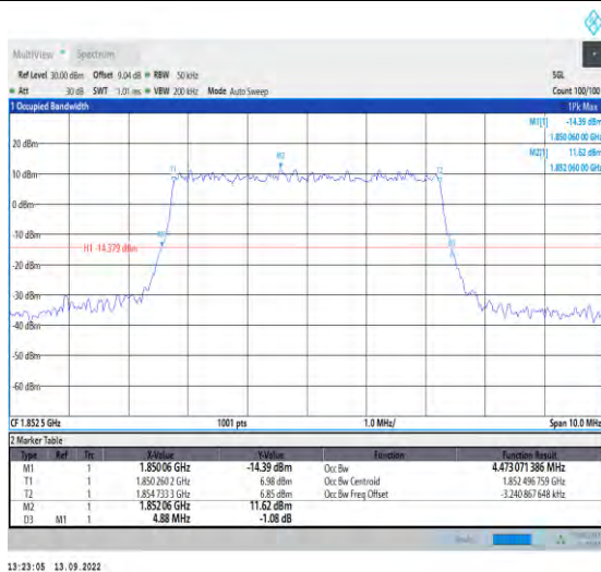
1-N2-PC3-15-5-L-3-DFT-16QAM-Outet_Full-25@0-A Ant1-4.473-4.880-<math>\leq 5</math>-PASS
