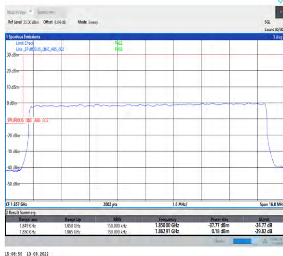
1-N2-PC3-15-15-L-3-DFT-PI2BPSK-Outer_Full-75 @0-Ant1-1-seegraph-PASS-see graph
