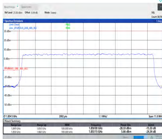
1-N2-PC3-15-10-L-3-DFT-PI2BPSK-Outer_Full-50 @0-Ant1-1-seegraph-PASS-see graph
