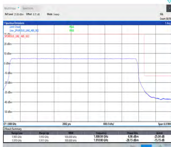
1-N2-PC3-15-5-H-6-CP-QPSK-Outer_Full-25@0-A nt1-1-seegraph-PASS-see graph
