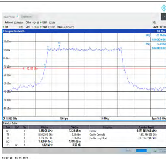
1-N2-PC3-15-5-L-1-DFT-QPSK-Outet_Full-25@0-An t1-4.471-4.820-<math>\leq 5</math>-PASS
