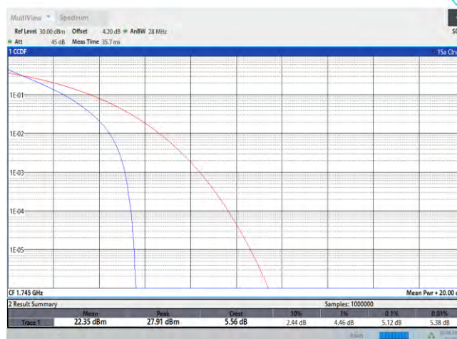
Band66-20MHz-QPSK-132322-100RB#0
