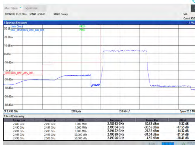
Band41-5MHz-QPSK-39675-25RB#0
