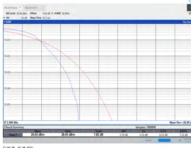
Band41-20MHz-QPSK-40620-100RB#0
