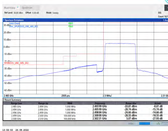
Band7-5MHz-QPSK-20775-25RB#0
