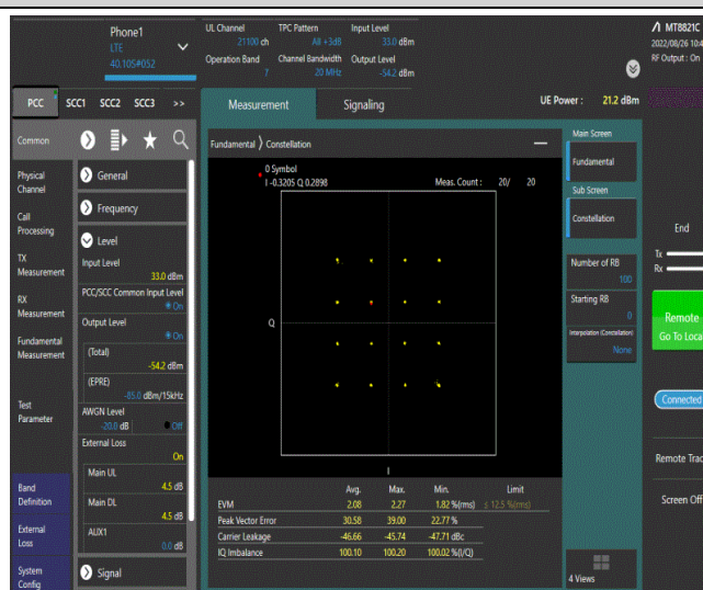
Band7-20MHz-16QAM-21100-100RB#0
