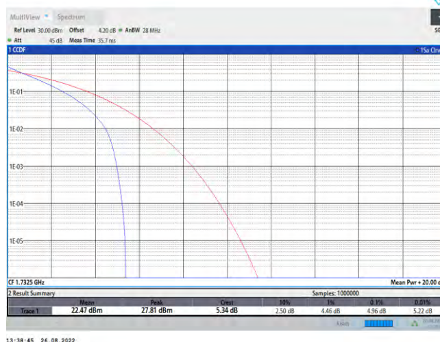
Band4-20MHz-QPSK-20175-100RB#0
