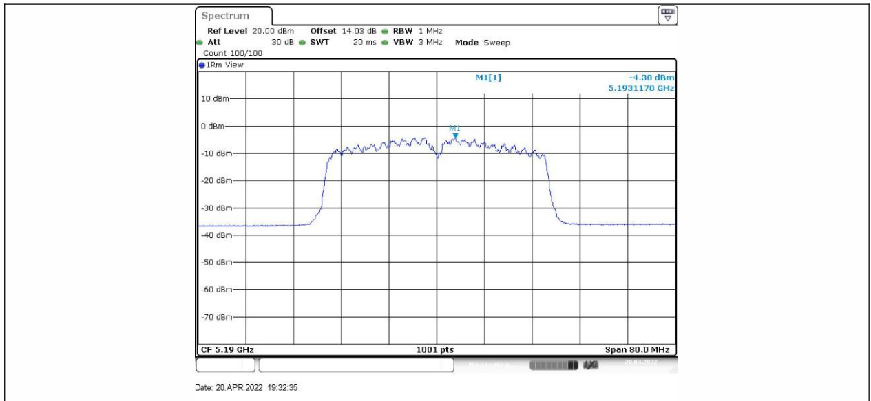
11AC40SISO_Ant2_5190
