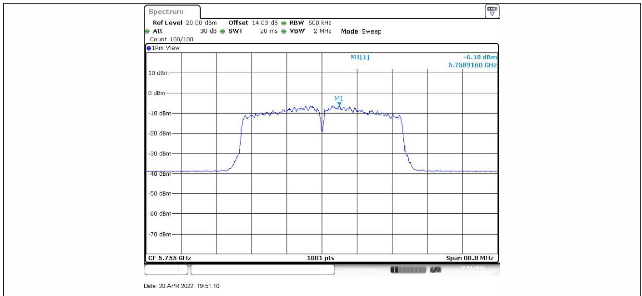
11AC40SISO_Ant2_5755
