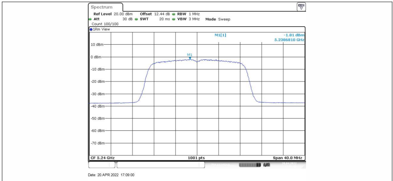
11N20SISO_Ant2_5240
