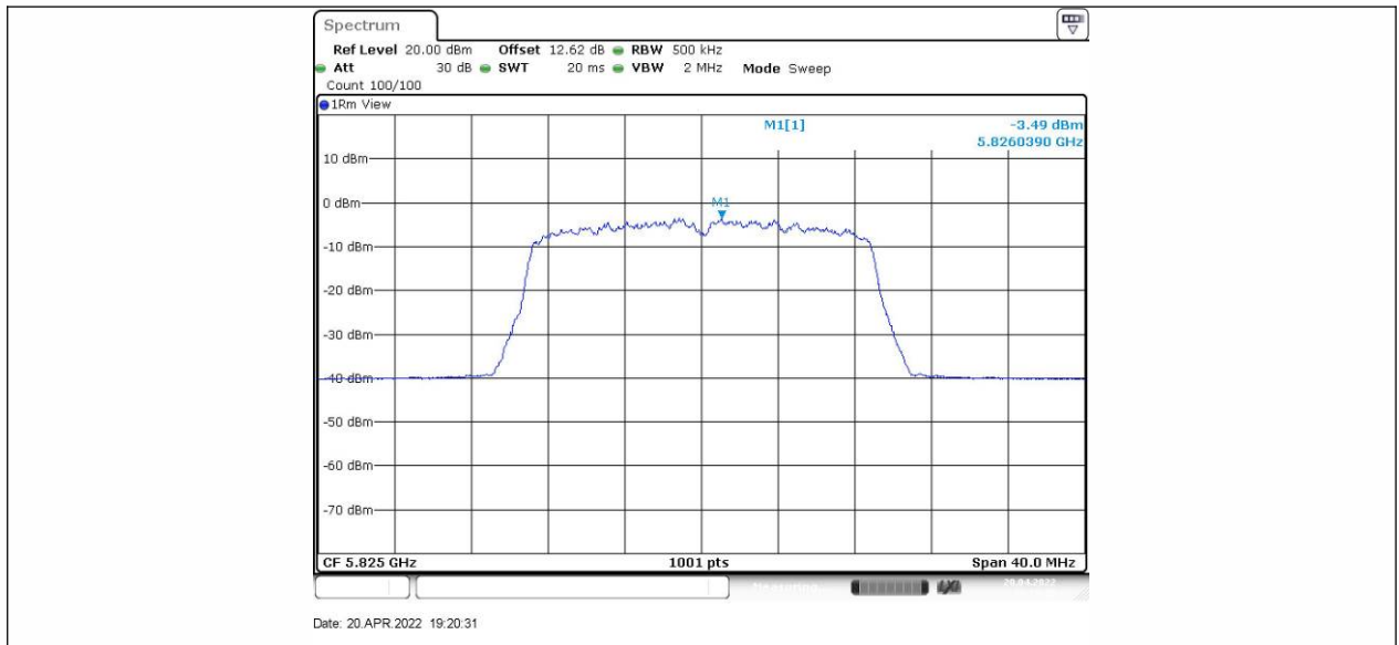
11AC20SISO_Ant2_5825
