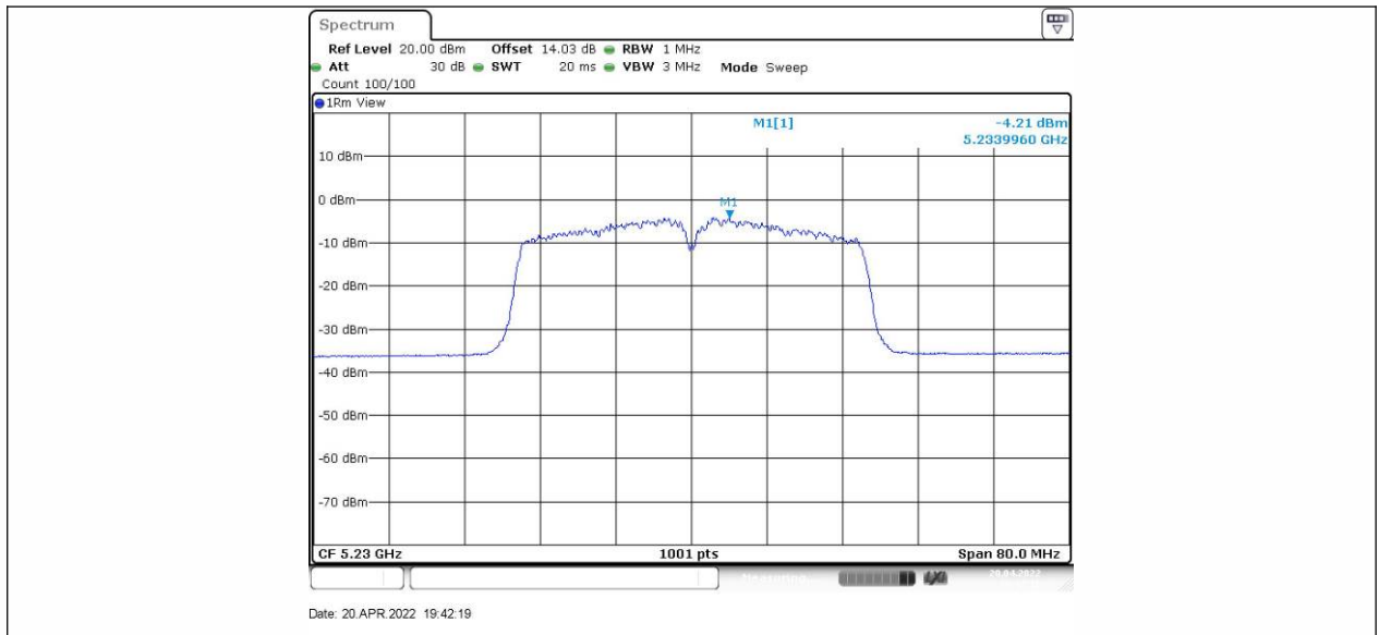
11AC40SISO_Ant2_5230
