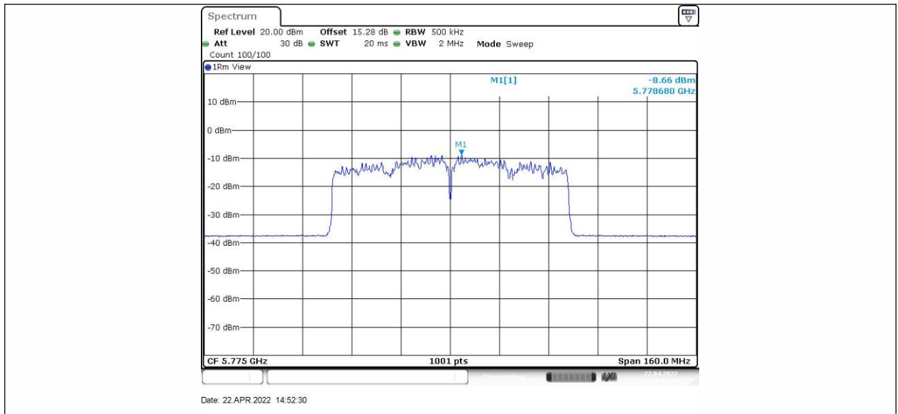
11AC80SISO_Ant2_5775
