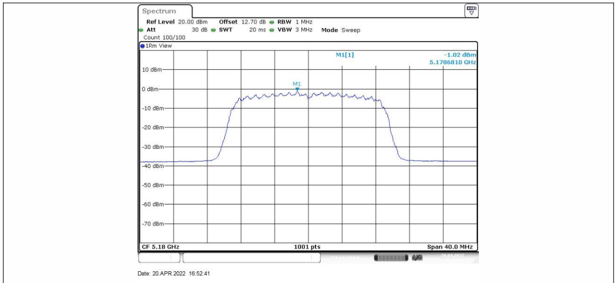
11N20SISO_Ant2_5180
