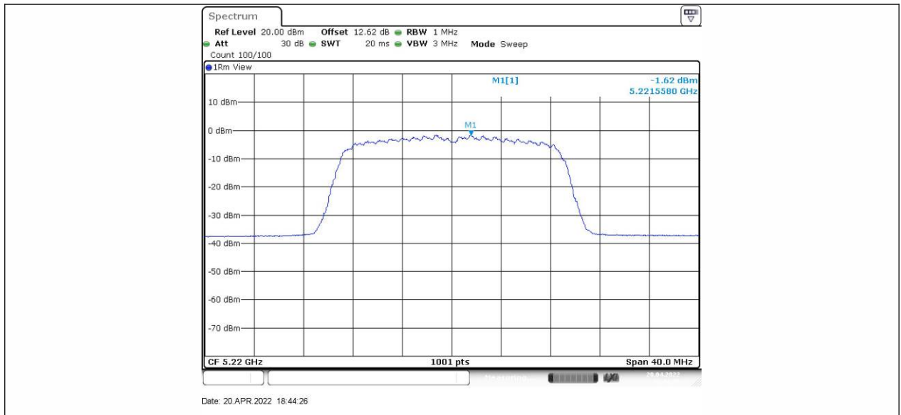
11AC20SISO_Ant2_5220
