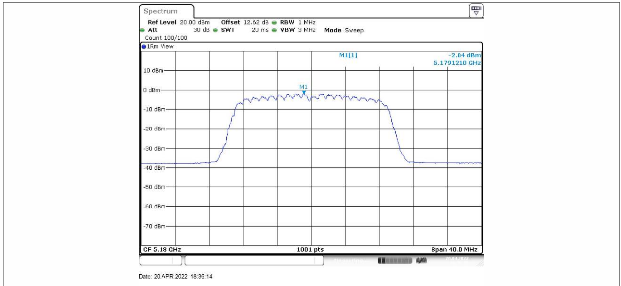
11AC20SISO_Ant2_5180
