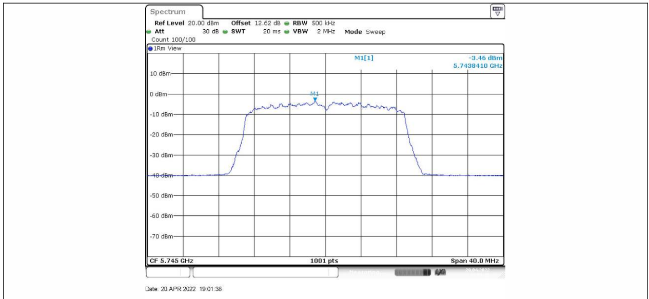
11AC20SISO_Ant2_5745
