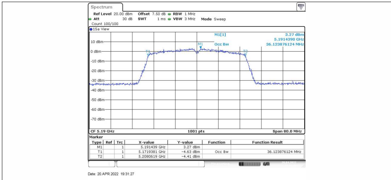
11AC40SISO_Ant2_5190
