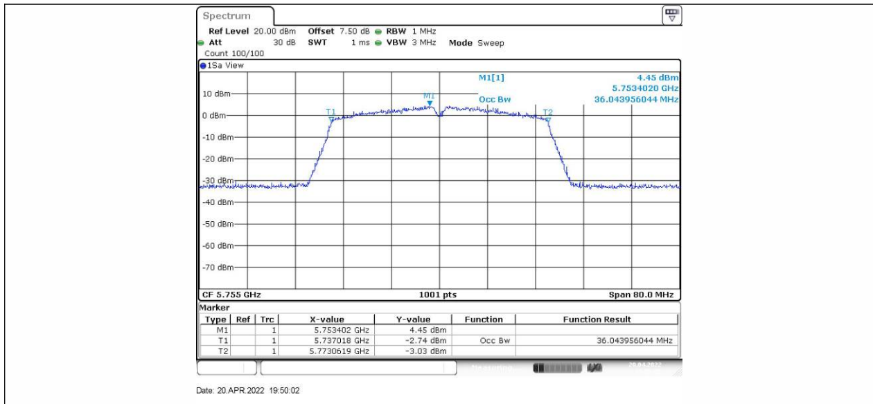
11AC40SISO_Ant2_5755
