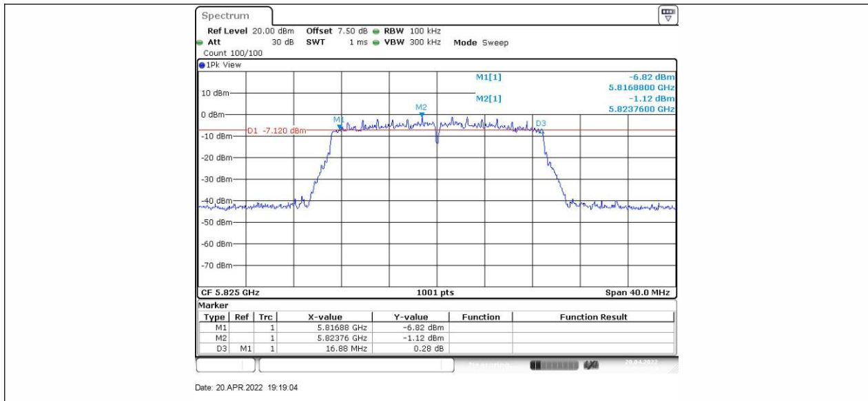
11AC20SISO_Ant2_5825
