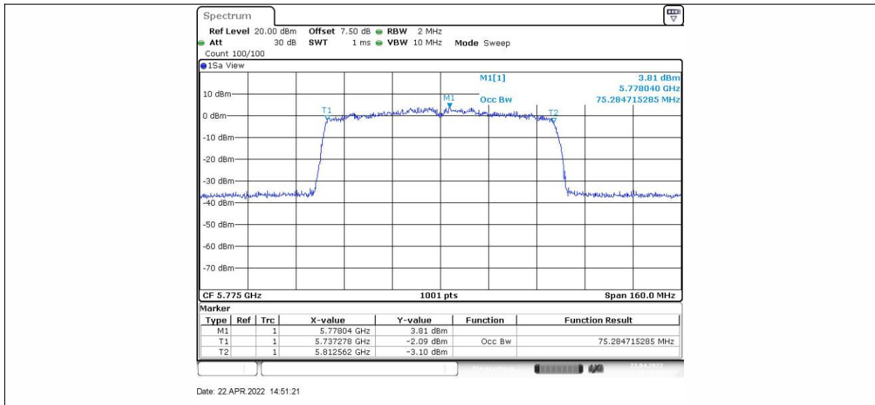
11AC80SISO_Ant2_5775
