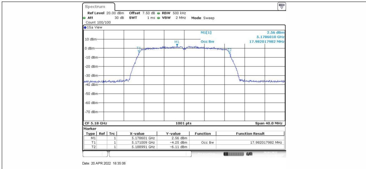
11AC20SISO_Ant2_5180
