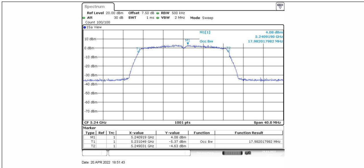
11AC20SISO_Ant2_5240
