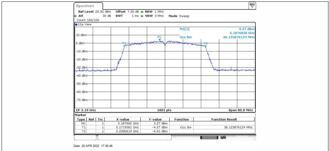
11N40SISO_Ant2_5190
