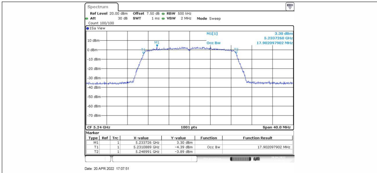
11N20SISO_Ant2_5240
