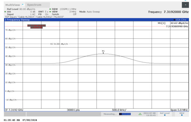
Plot 7.6.21 Radiated emission measurements at the 9 harmonic of low carrier frequency
