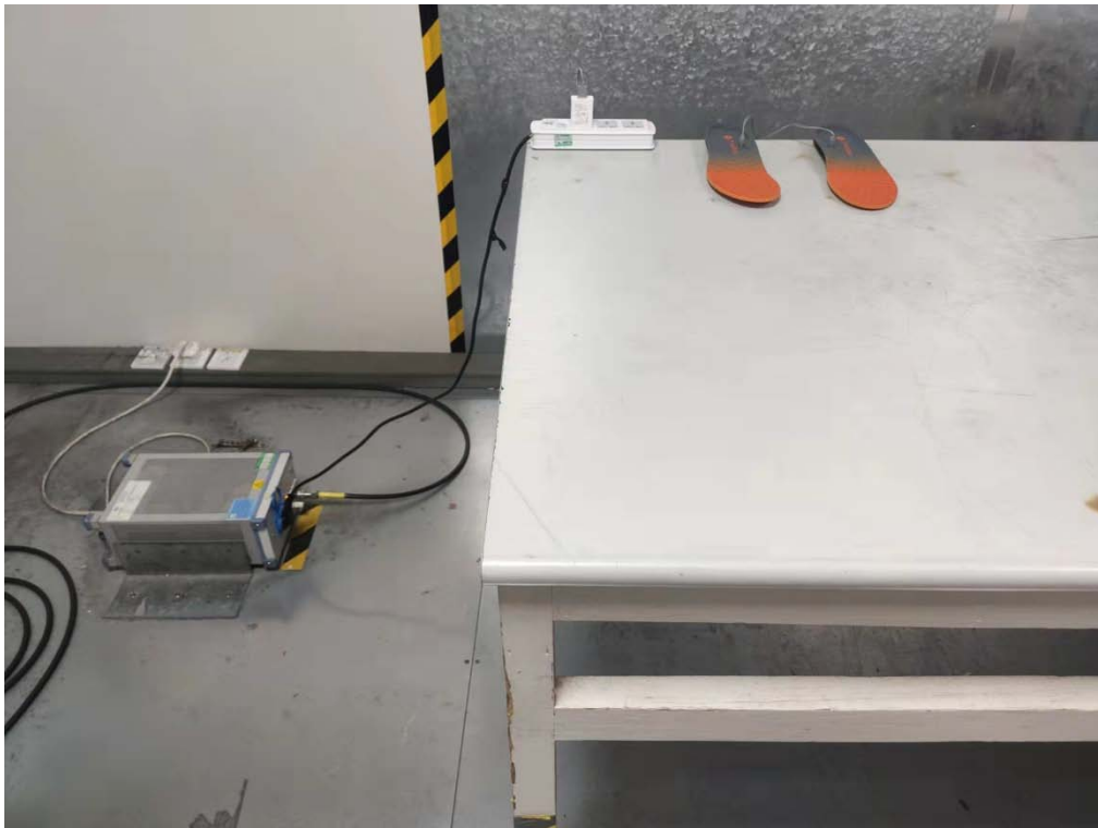
AC Mains conducted emission test
