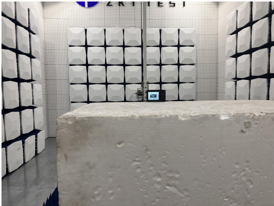
RADIATED EMISSION MEASUREMENT (Above 1G)
