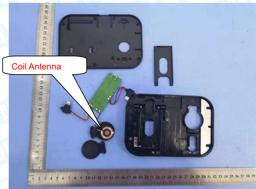
Photo 11 Internal of EUT
