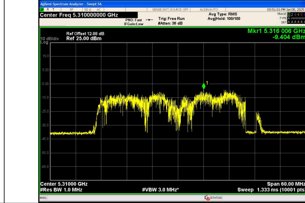
IEEE 802.11ac Channel 62 40MHz Antenna 0
