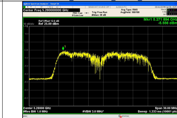
IEEE 802.11n Channel 56 20MHz Antenna 0
