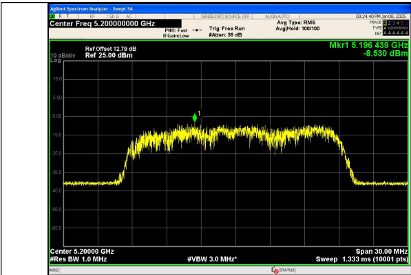
IEEE 802.11ac Channel 40 20MHz Antenna 0
