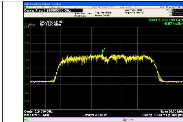
IEEE 802.11n Channel 48 20MHz Antenna 0
