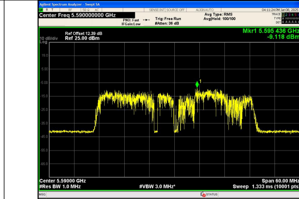
IEEE 802.11ac Channel 118 40MHz Antenna 0
