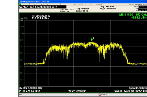
IEEE 802.11ac Channel 100 20MHz Antenna 0
