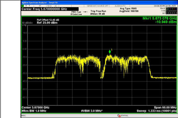
IEEE 802.11n Channel 134 40MHz Antenna 0
