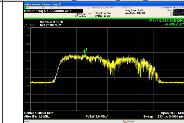
IEEE 802.11n Channel 100 20MHz Antenna 0
