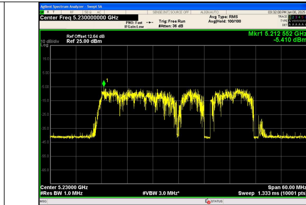
IEEE 802.11ac Channel 46 40MHz Antenna 0
