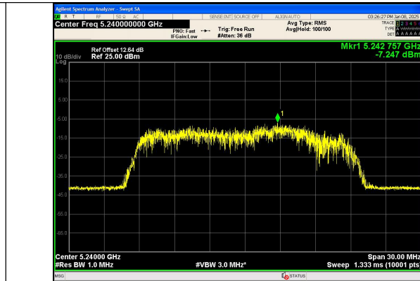
IEEE 802.11ac Channel 48 20MHz Antenna 0
