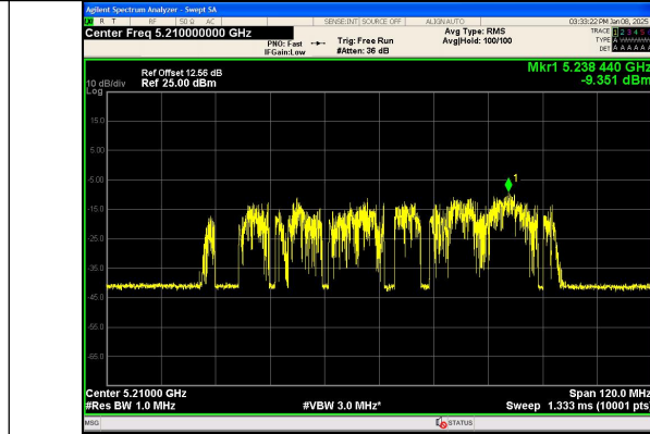
IEEE 802.11ac Channel 42 80MHz Antenna 0
