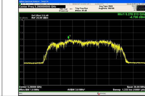
IEEE 802.11ac Channel 56 20MHz Antenna 0
