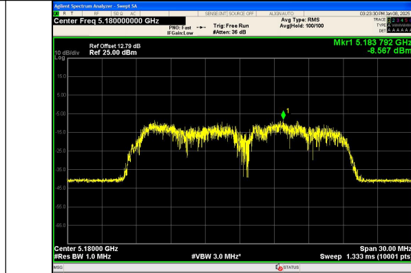
IEEE 802.11ac Channel 36 20MHz Antenna 0
