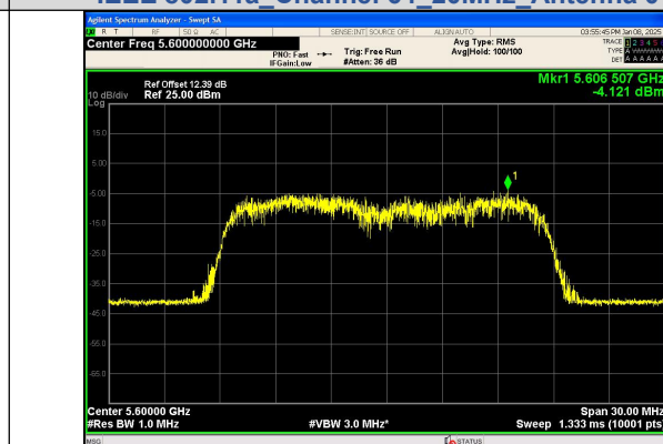
IEEE 802.11a Channel 120 20MHz Antenna 0
