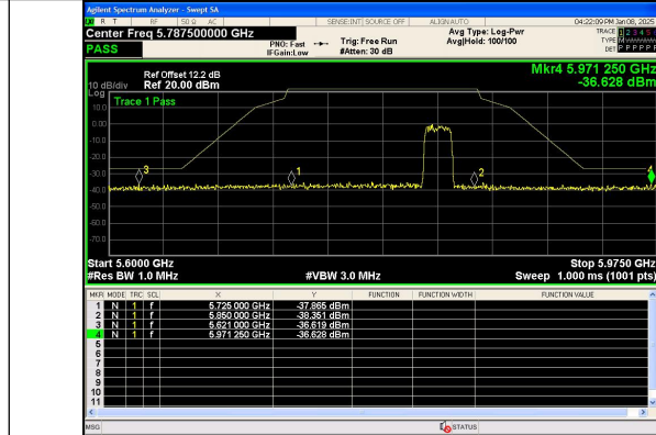
Out Of Band Emission IEEE 802.11n Channel 165_20MHz_Antenna 0
