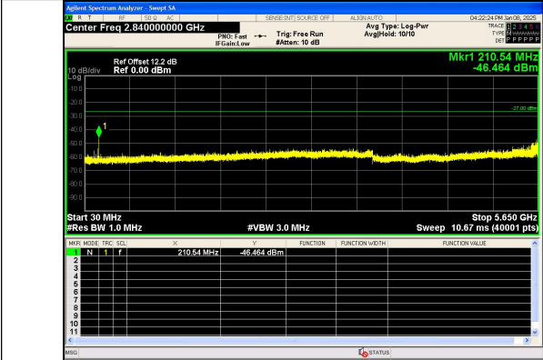
Spurious Emission:30.0~5650 MHz IEEE 802.11n Channel 165_20MHz_Antenna 0
