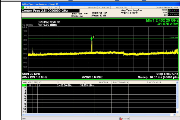
Spurious Emission:30.0~5650 MHz IEEE 802.11ac Channel 151 40MHz Antenna 0
