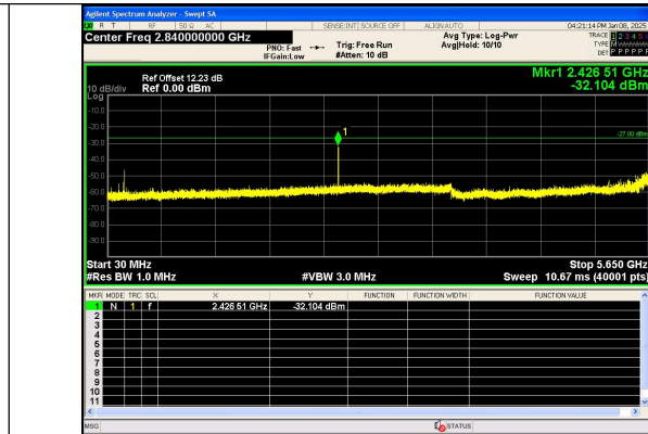
Spurious Emission:30.0~5650 MHz IEEE 802.11n Channel 157_20MHz_Antenna 0
