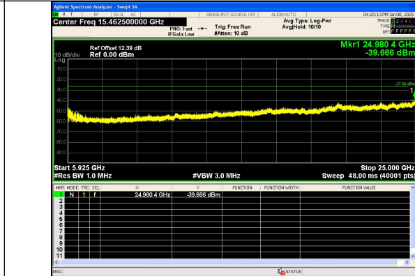
Spurious Emission:5925~25000.0 MHz IEEE 802.11n Channel 149_20MHz_Antenna 0
