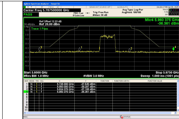
Out Of Band Emission IEEE 802.11n Channel 159 40MHz Antenna 0
