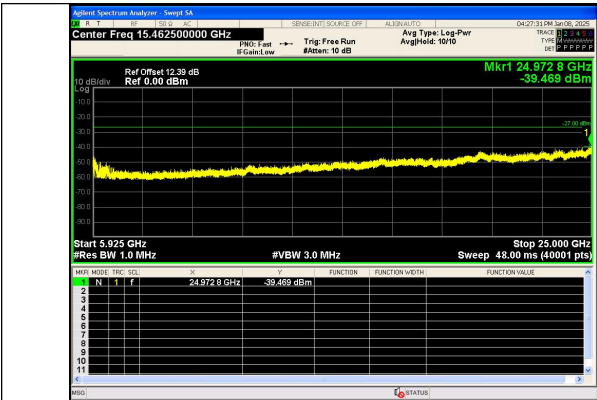
Spurious Emission:5925~25000.0 MHz IEEE 802.11n Channel 151 40MHz Antenna 0
