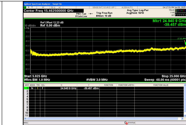
Spurious Emission:5925~25000.0 MHz IEEE 802.11a Channel 157_20MHz_Antenna 0
