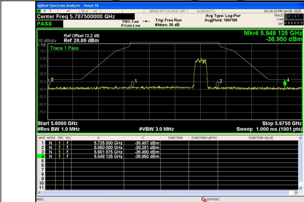
Out Of Band Emission IEEE 802.11a Channel 165_20MHz_Antenna 0
