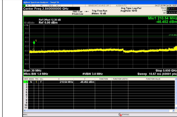
Spurious Emission:30.0~5650 MHz IEEE 802.11n Channel 151_40MHz_Antenna 0
