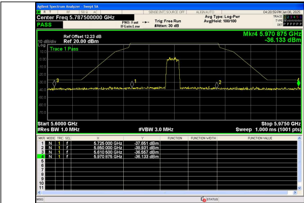
Out Of Band Emission IEEE 802.11n Channel 157_20MHz_Antenna 0
