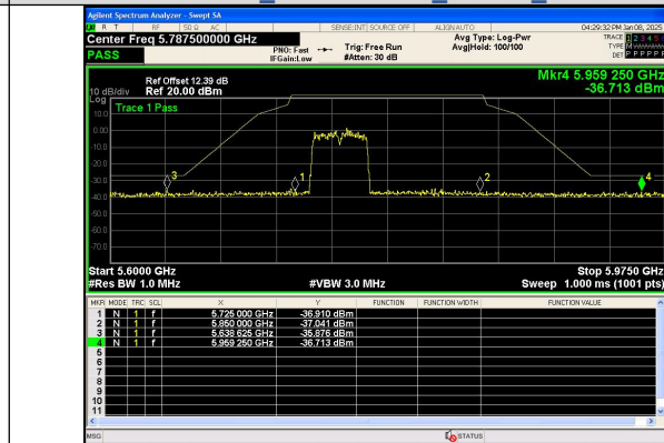
Out Of Band Emission IEEE 802.11ac Channel 151 40MHz Antenna 0
