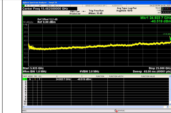
Spurious Emission:5925~25000.0 MHz IEEE 802.11n Channel 165_20MHz_Antenna 0
