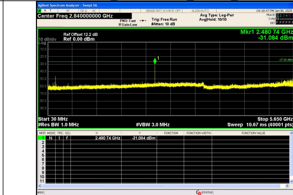
Spurious Emission:30.0~5650 MHz IEEE 802.11a Channel 165_20MHz_Antenna 0
