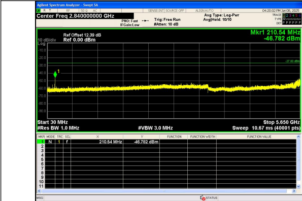
Spurious Emission:30.0~5650 MHz IEEE 802.11n Channel 149_20MHz_Antenna 0
