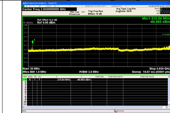
Spurious Emission:30.0~5650 MHz IEEE 802.11ac Channel 165 20MHz Antenna 0
