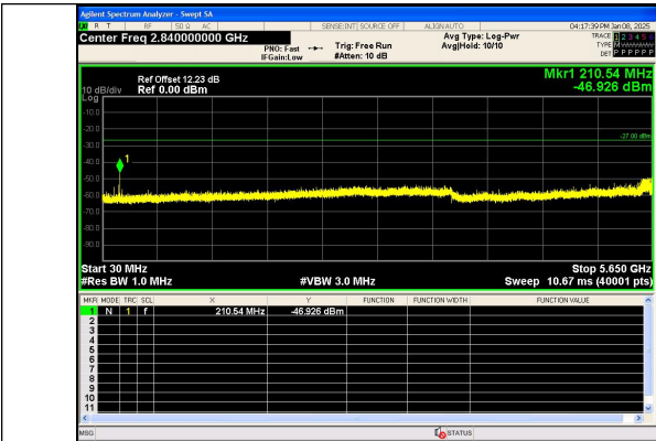
Spurious Emission:30.0~5650 MHz IEEE 802.11a Channel 157_20MHz_Antenna 0
