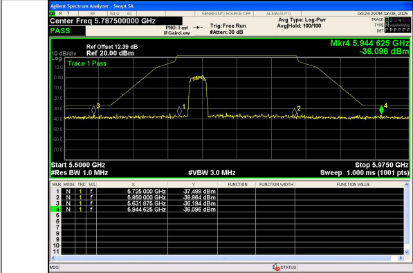
Out Of Band Emission IEEE 802.11ac Channel 149 20MHz Antenna 0
