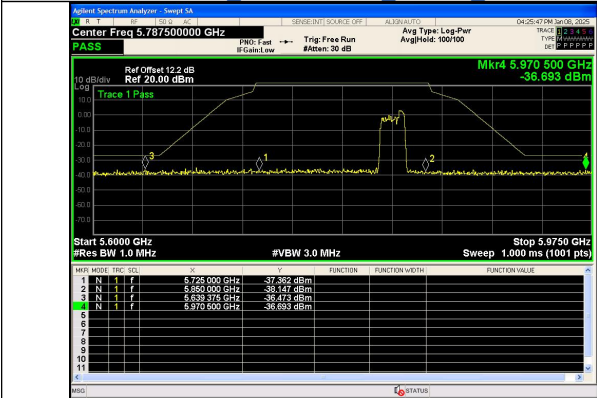
Out Of Band Emission IEEE 802.11ac Channel 165 20MHz Antenna 0
