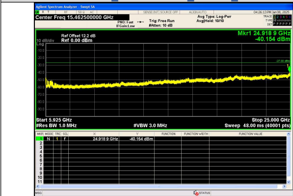
Spurious Emission:5925~25000.0 MHz IEEE 802.11ac Channel 165 20MHz Antenna 0
