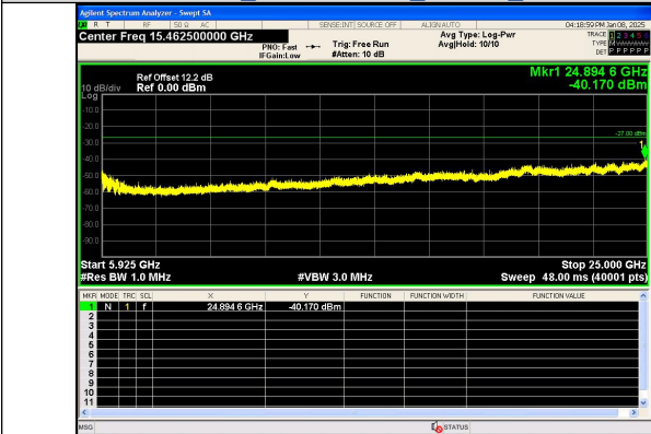
Spurious Emission:5925~25000.0 MHz IEEE 802.11a Channel 165_20MHz_Antenna 0
