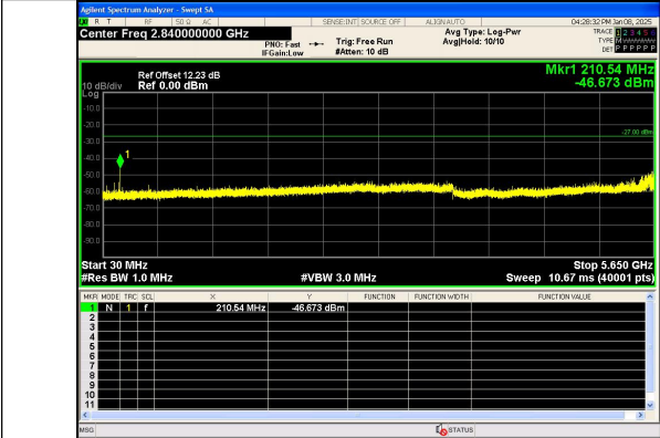
Spurious Emission:30.0~5650 MHz IEEE 802.11n Channel 159 40MHz Antenna 0
