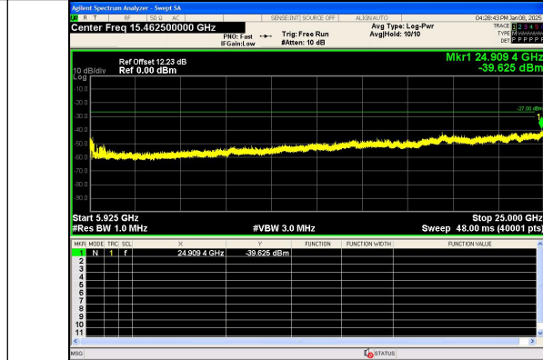
Spurious Emission:5925~25000.0 MHz IEEE 802.11n Channel 159 40MHz Antenna 0
