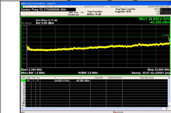
Spurious Emission:5350~25000.0 MHz IEEE 802.11ac Channel 52_20MHz_Antenna 0
