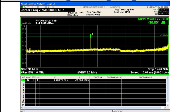
Spurious Emission:30.0~5470 MHz IEEE 802.11ac Channel 100 20MHz Antenna 0
