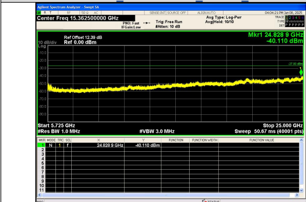
Spurious Emission:5725~25000.0 MHz IEEE 802.11ac Channel 120 20MHz Antenna 0
