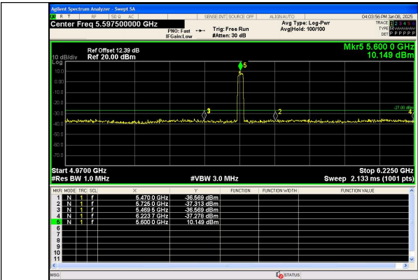
Out Of Band Emission IEEE 802.11ac Channel 120 20MHz Antenna 0
