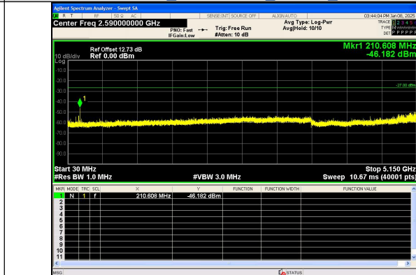
Spurious Emission:30.0~5150 MHz IEEE 802.11ac Channel 52_20MHz_Antenna 0
