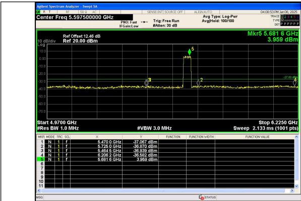
Out Of Band Emission IEEE 802.11n Channel 134 40MHz Antenna 0
