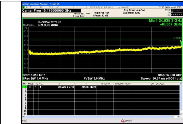
Spurious Emission:5350~25000.0 MHz IEEE 802.11ac Channel 40_20MHz_Antenna 0
