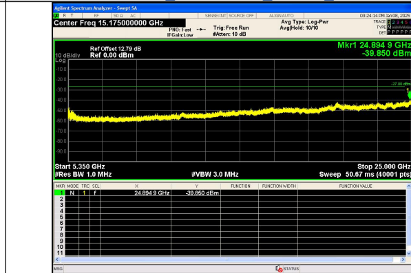
Spurious Emission:5350~25000.0 MHz IEEE 802.11ac Channel 36 20MHz Antenna 0
