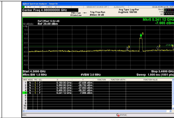
Out Of Band Emission IEEE 802.11ac Channel 48_20MHz_Antenna 0
