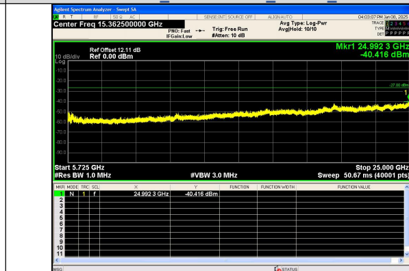
Spurious Emission:5725~25000.0 MHz IEEE 802.11ac Channel 100 20MHz Antenna 0
