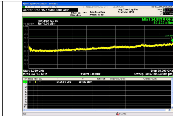
Spurious Emission:5350~25000.0 MHz IEEE 802.11ac Channel 56 20MHz Antenna 0
