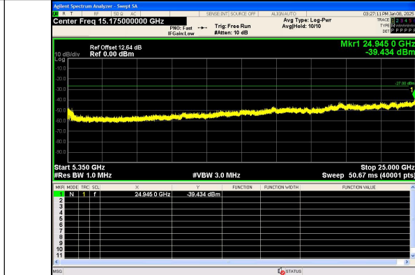
Spurious Emission:5350~25000.0 MHz IEEE 802.11ac Channel 48_20MHz_Antenna 0
