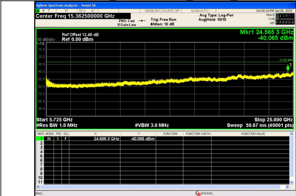
Spurious Emission:5725~25000.0 MHz IEEE 802.11n Channel 134 40MHz Antenna 0
