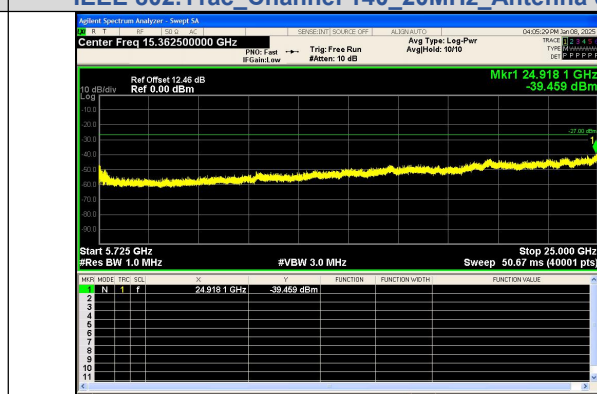
Spurious Emission:5725~25000.0 MHz IEEE 802.11ac Channel 140 20MHz Antenna 0
