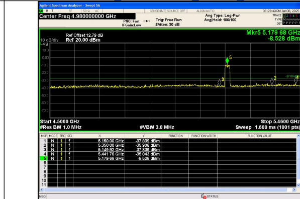
Out Of Band Emission IEEE 802.11ac Channel 36 20MHz Antenna 0
