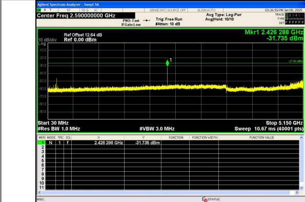
Spurious Emission:30.0~5150 MHz IEEE 802.11ac Channel 48_20MHz_Antenna 0
