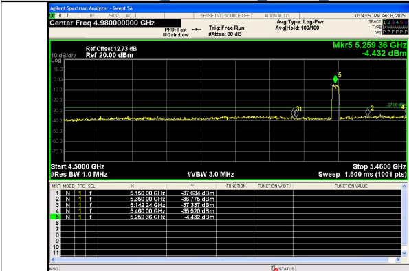
Out Of Band Emission IEEE 802.11ac Channel 52_20MHz_Antenna 0
