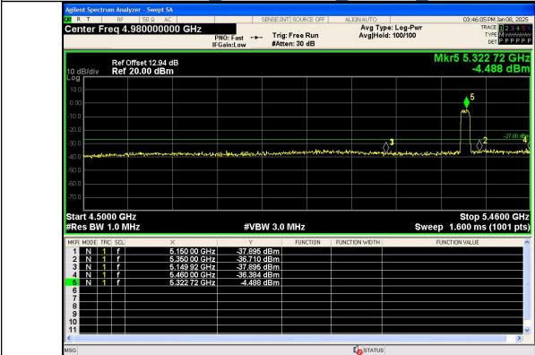
Out Of Band Emission IEEE 802.11ac Channel 64 20MHz Antenna 0
