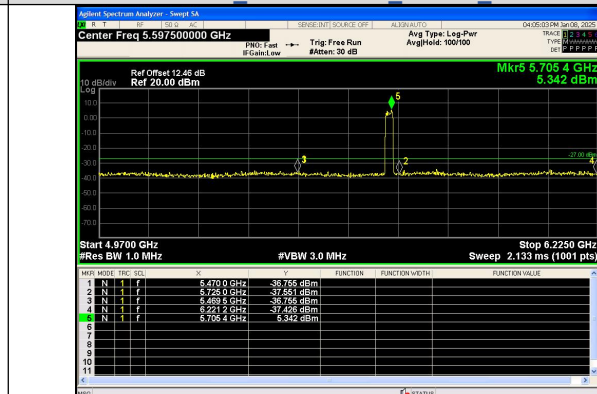
Out Of Band Emission IEEE 802.11ac Channel 140 20MHz Antenna 0
