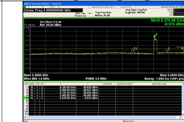
Out Of Band Emission IEEE 802.11ac Channel 56_20MHz_Antenna 0
