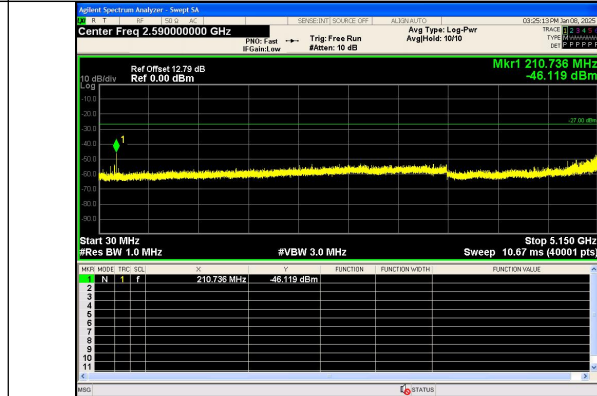
Spurious Emission:30.0~5150 MHz IEEE 802.11ac Channel 40 20MHz Antenna 0
