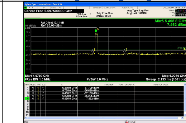
Out Of Band Emission IEEE 802.11ac Channel 100 20MHz Antenna 0
