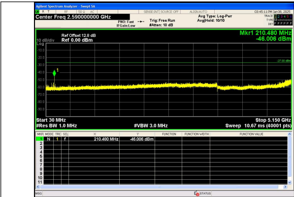
Spurious Emission:30.0~5150 MHz IEEE 802.11ac Channel 56 20MHz Antenna 0
