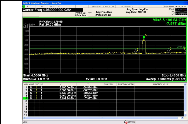
Out Of Band Emission IEEE 802.11ac Channel 40 20MHz Antenna 0
