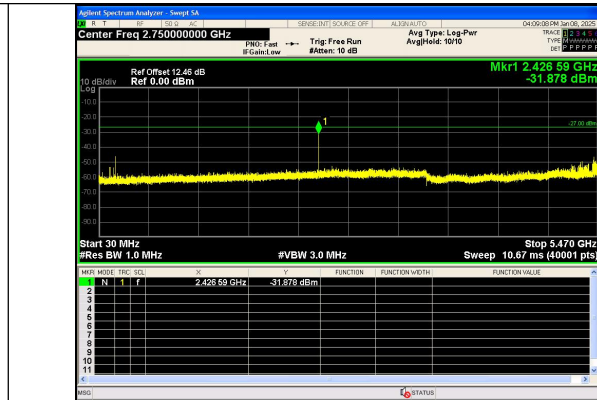
Spurious Emission:30.0~5470 MHz IEEE 802.11n Channel 134 40MHz Antenna 0
