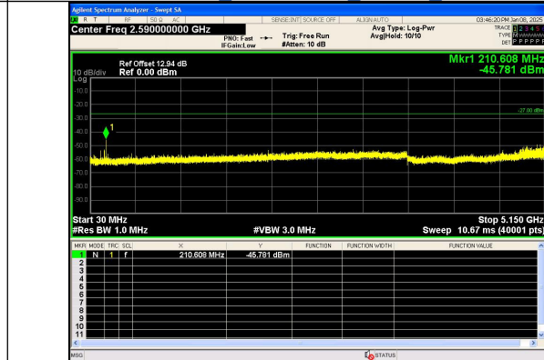
Spurious Emission:30.0~5150 MHz IEEE 802.11ac Channel 64 20MHz Antenna 0
