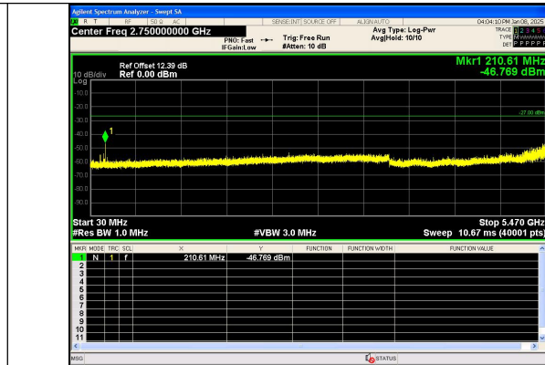
Spurious Emission:30.0~5470 MHz IEEE 802.11ac Channel 120 20MHz Antenna 0
