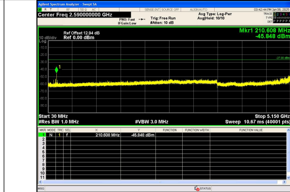
Spurious Emission:30.0~5150 MHz IEEE 802.11n Channel 64 20MHz Antenna 0
