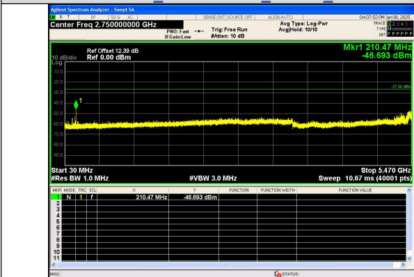
Spurious Emission:30.0~5470 MHz IEEE 802.11n Channel 118 40MHz Antenna 0
