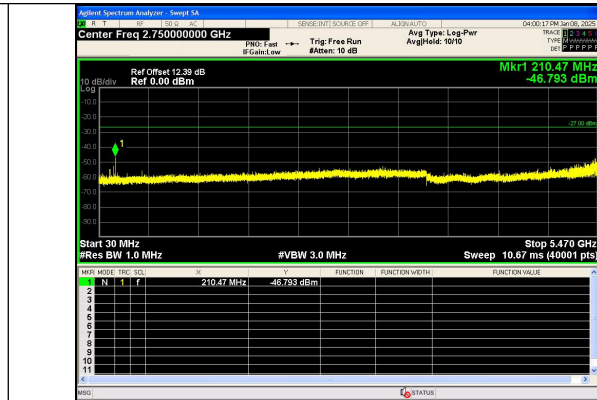
Spurious Emission:30.0~5470 MHz IEEE 802.11n Channel 120 20MHz Antenna 0
