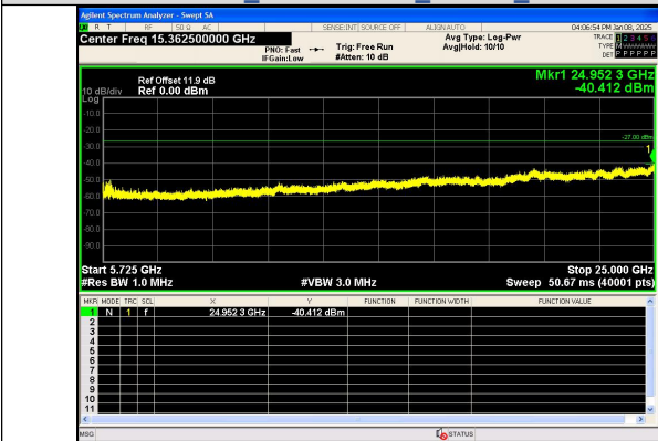
Spurious Emission:5725~25000.0 MHz IEEE 802.11n Channel 102 40MHz Antenna 0
