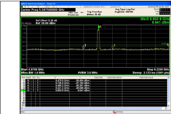
Out Of Band Emission IEEE 802.11n Channel 120 20MHz Antenna 0
