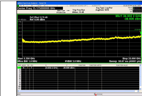
Spurious Emission:5350~25000.0 MHz IEEE 802.11n Channel 38 40MHz Antenna 0
