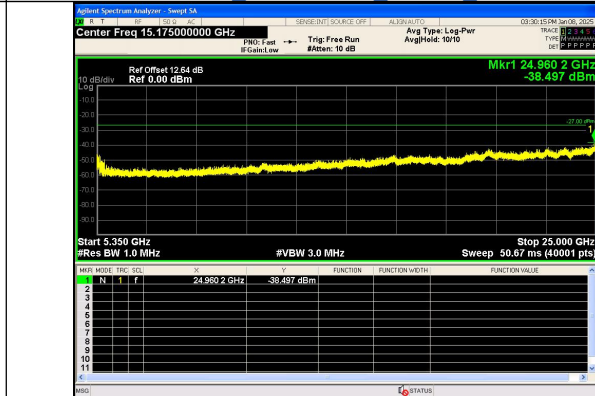
Spurious Emission:5350~25000.0 MHz IEEE 802.11n Channel 46 40MHz Antenna 0
