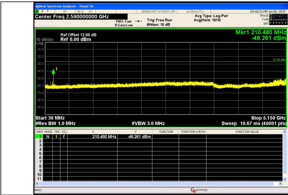
Spurious Emission:30.0~5150 MHz IEEE 802.11n Channel 62 40MHz Antenna 0
