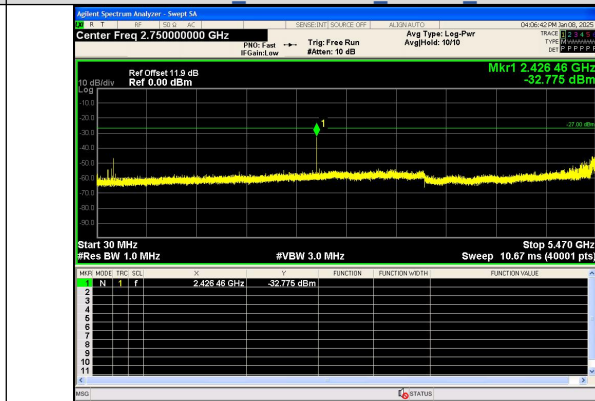
Spurious Emission:30.0~5470 MHz IEEE 802.11n Channel 102 40MHz Antenna 0
