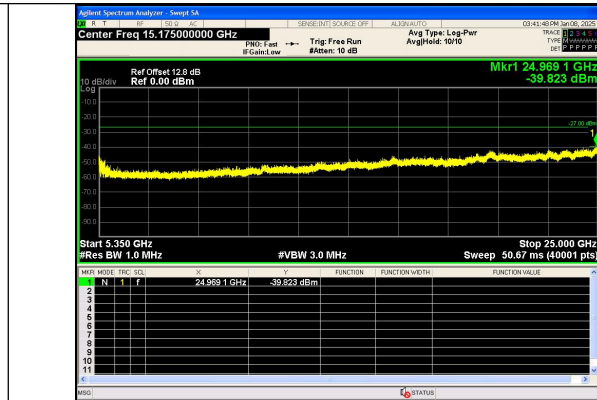
Spurious Emission:5350~25000.0 MHz IEEE 802.11n Channel 56 20MHz Antenna 0
