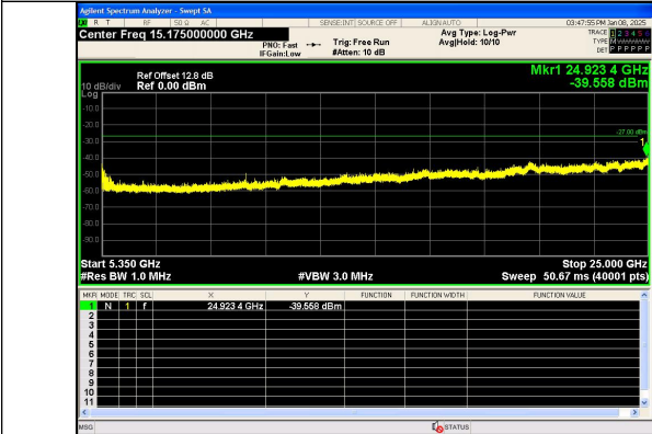
Spurious Emission:5350~25000.0 MHz IEEE 802.11n Channel 54 40MHz Antenna 0
