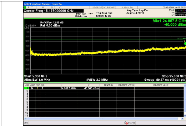
Spurious Emission:5350~25000.0 MHz IEEE 802.11n Channel 62 40MHz Antenna 0
