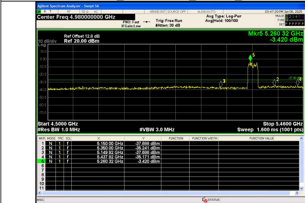
Out Of Band Emission IEEE 802.11n Channel 54 40MHz Antenna 0
