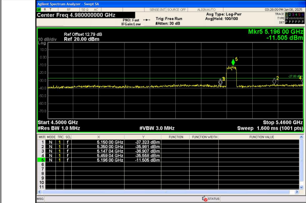
Out Of Band Emission IEEE 802.11n Channel 38 40MHz Antenna 0
