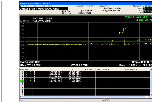
Out Of Band Emission IEEE 802.11n Channel 46 40MHz Antenna 0
