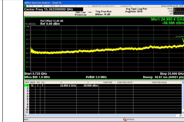
Spurious Emission:5725~25000.0 MHz IEEE 802.11n Channel 140 20MHz Antenna 0
