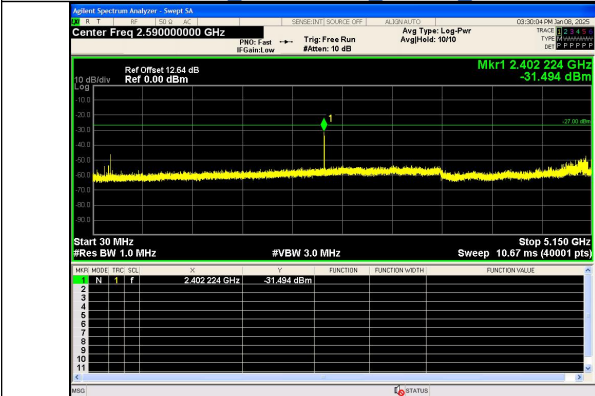
Spurious Emission:30.0~5150 MHz IEEE 802.11n Channel 46 40MHz Antenna 0
