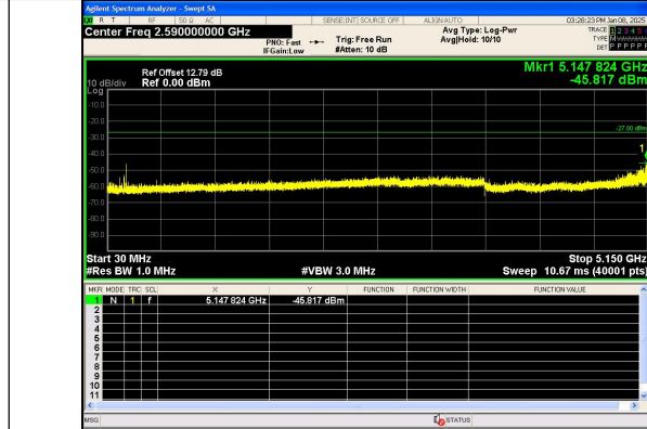
Spurious Emission:30.0~5150 MHz IEEE 802.11n Channel 38 40MHz Antenna 0
