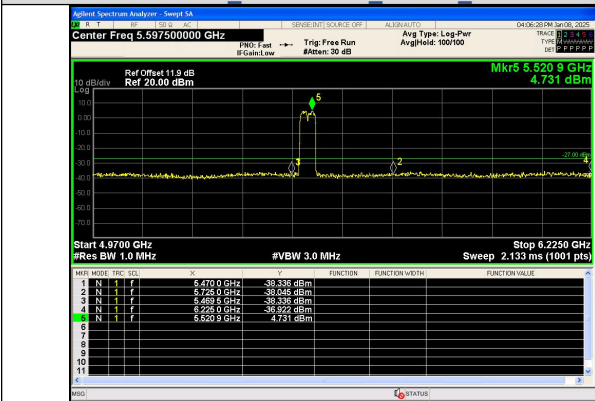
Out Of Band Emission IEEE 802.11n Channel 102 40MHz Antenna 0
