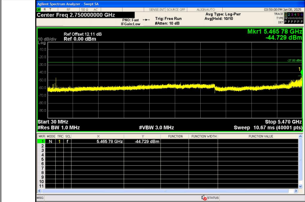
Spurious Emission:30.0~5470 MHz IEEE 802.11n Channel 100 20MHz Antenna 0
