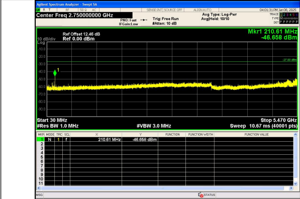
Spurious Emission:30.0~5470 MHz IEEE 802.11n Channel 140 20MHz Antenna 0
