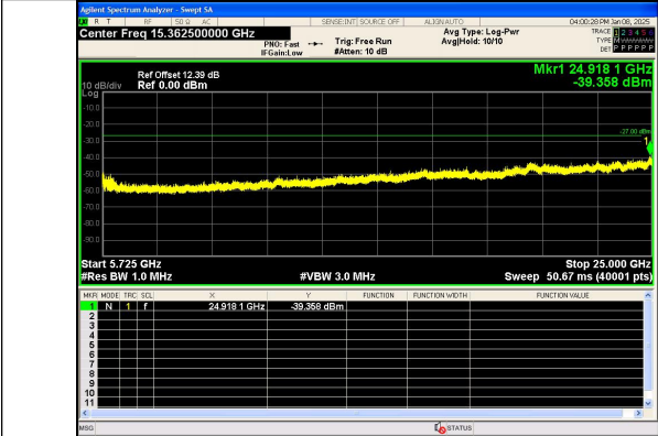
Spurious Emission:5725~25000.0 MHz IEEE 802.11n Channel 120 20MHz Antenna 0
