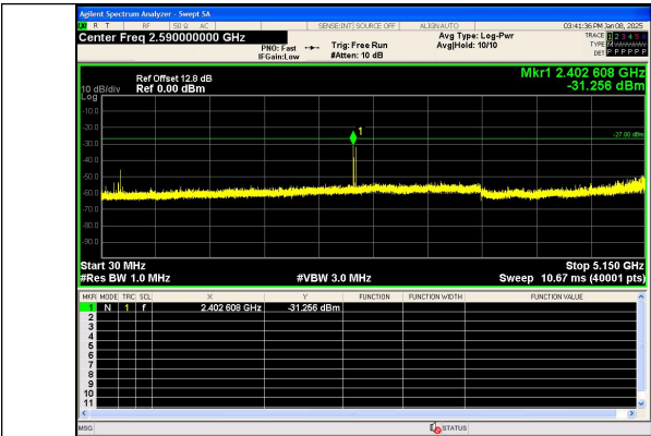
Spurious Emission:30.0~5150 MHz IEEE 802.11n Channel 56 20MHz Antenna 0
