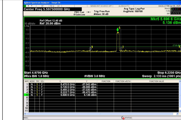
Out Of Band Emission IEEE 802.11n Channel 140 20MHz Antenna 0
