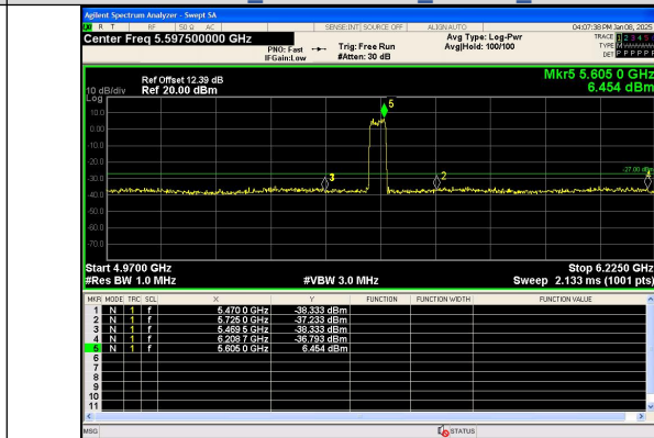
Out Of Band Emission IEEE 802.11n Channel 118 40MHz Antenna 0
