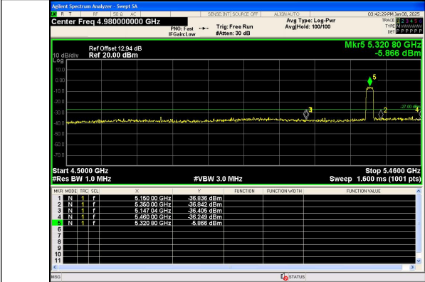
Out Of Band Emission IEEE 802.11n Channel 64 20MHz Antenna 0
