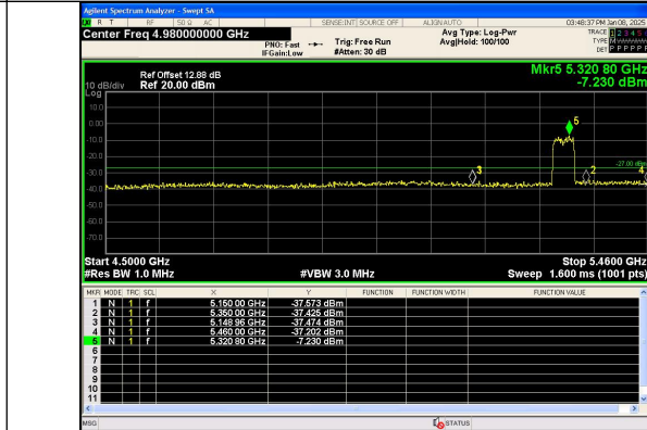
Out Of Band Emission IEEE 802.11n Channel 62 40MHz Antenna 0
