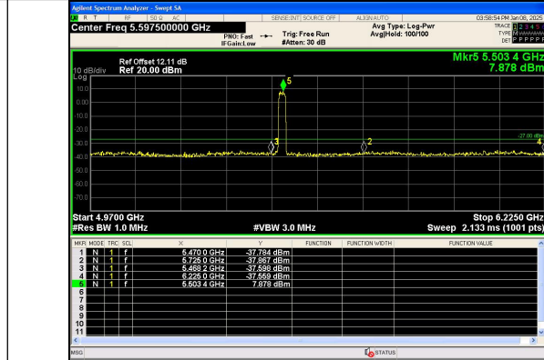
Out Of Band Emission IEEE 802.11n Channel 100 20MHz Antenna 0
