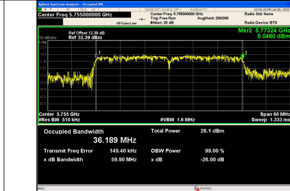
IEEE 802.11ac Channel 151 40MHz Antenna 0
