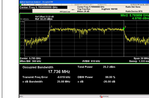
IEEE 802.11ac Channel 157 20MHz Antenna 0
