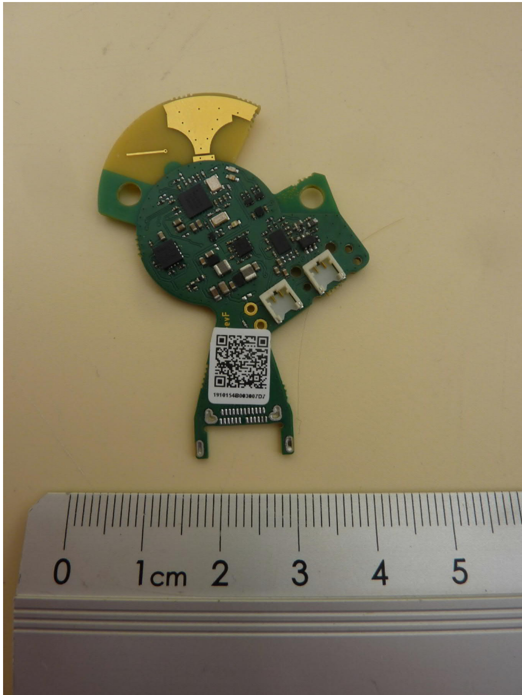
Marker Mini, PCB, top view
