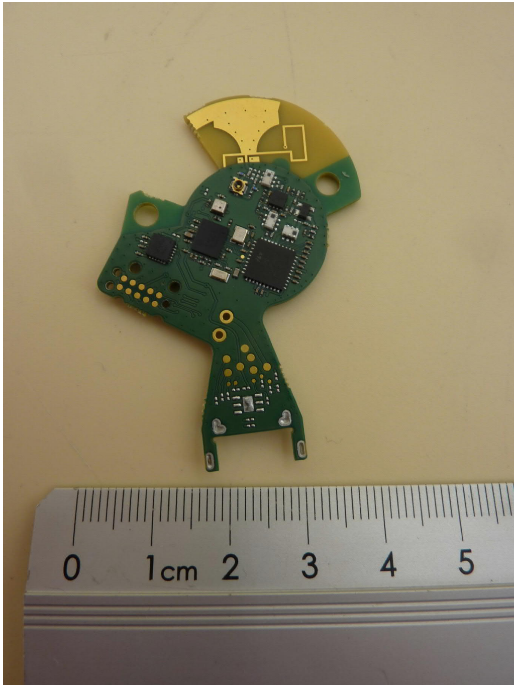
Marker Mini, PCB, bottom view
