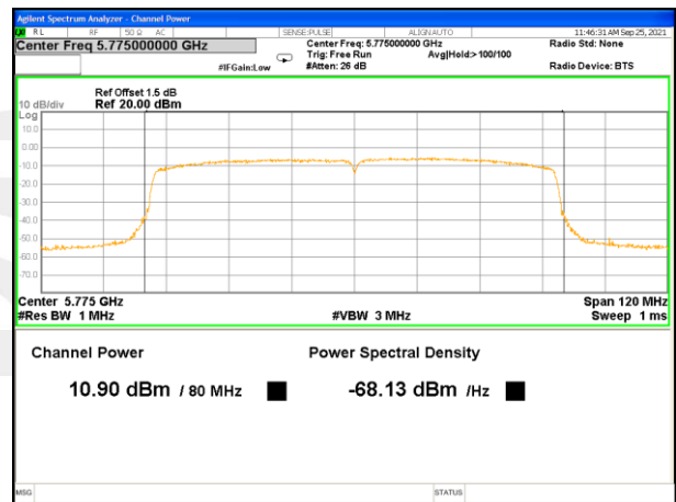
5775MHz_AV_Ant B
