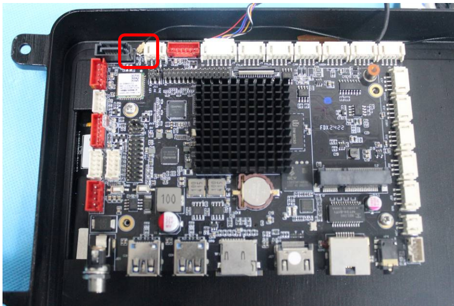
Antenna position
