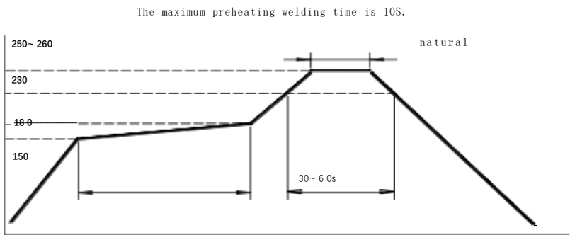
reflow soldering
