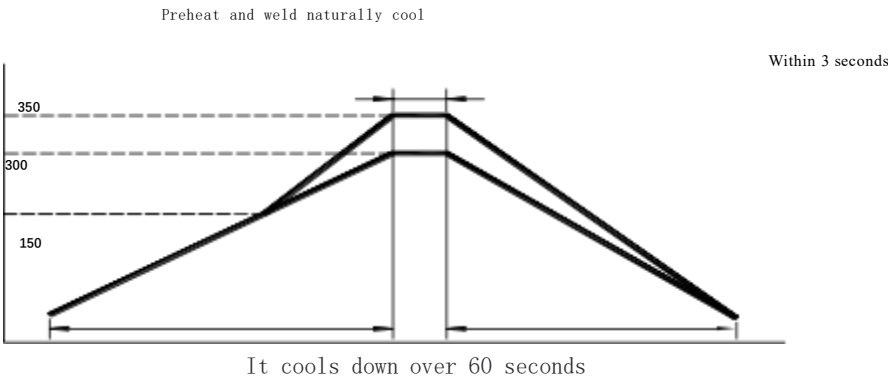
iron soldering
