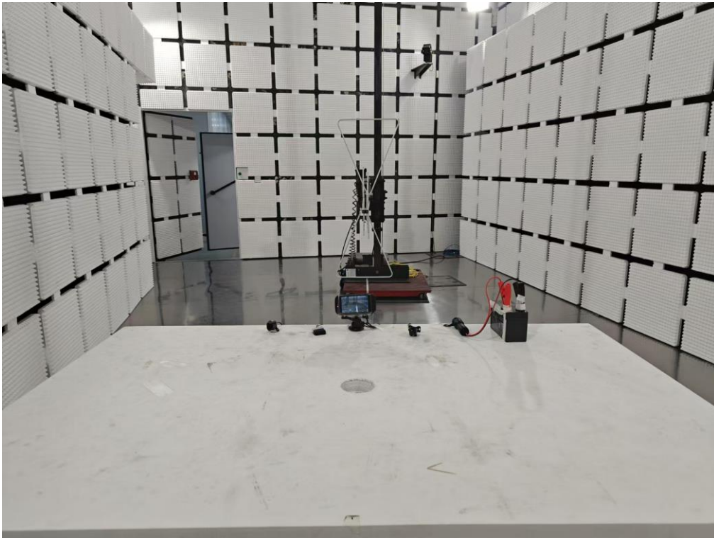
Radiated Emissions Test Photo
