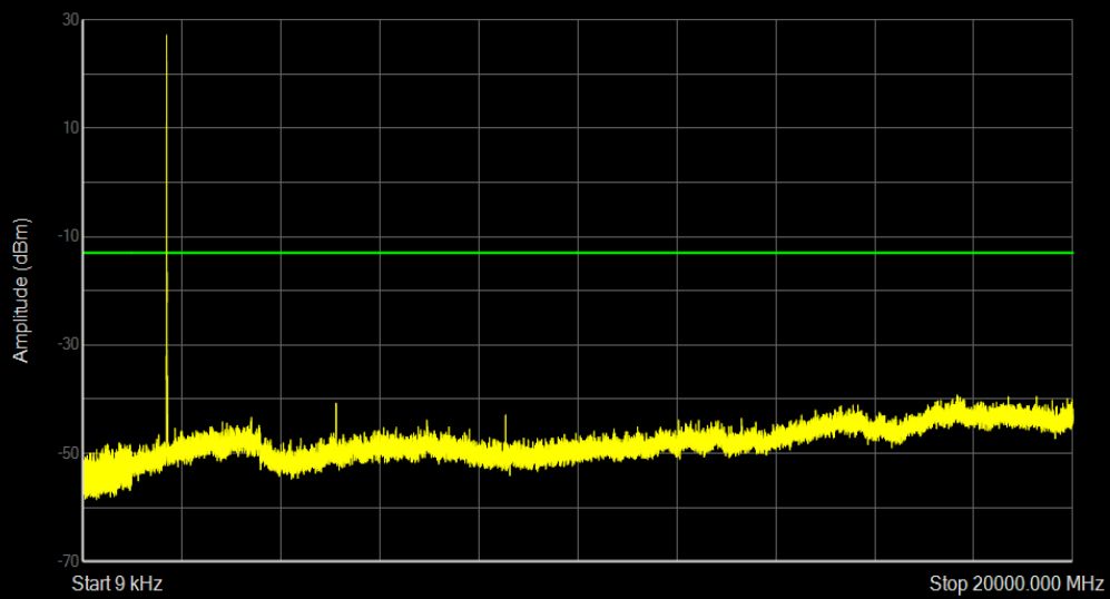
Band4 16QAM BW=3MHz Channel=19965 RB Size=1 Position=#0
