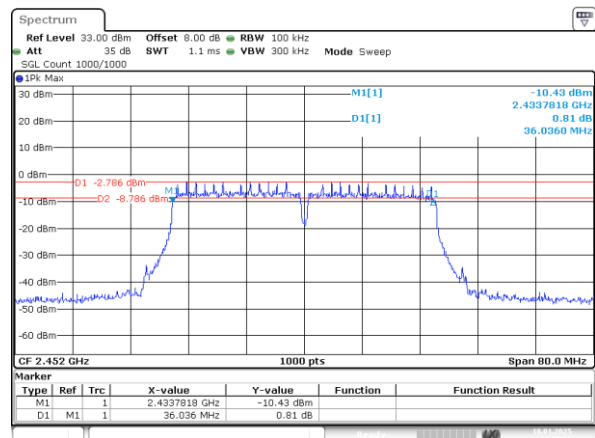
802.11n40_2452MHz
