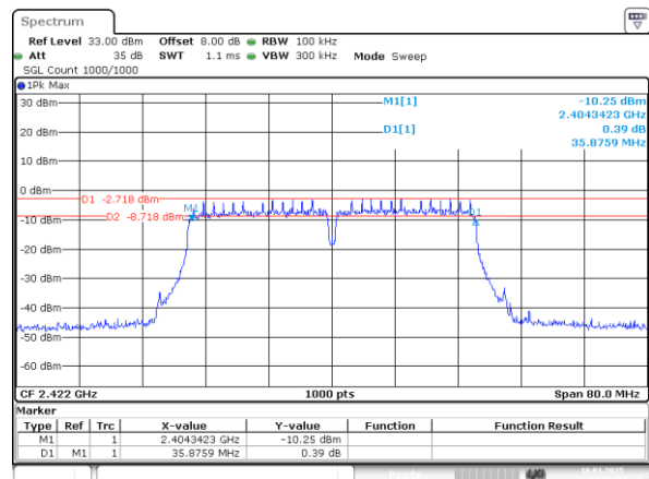
802.11n40_2422MHz
