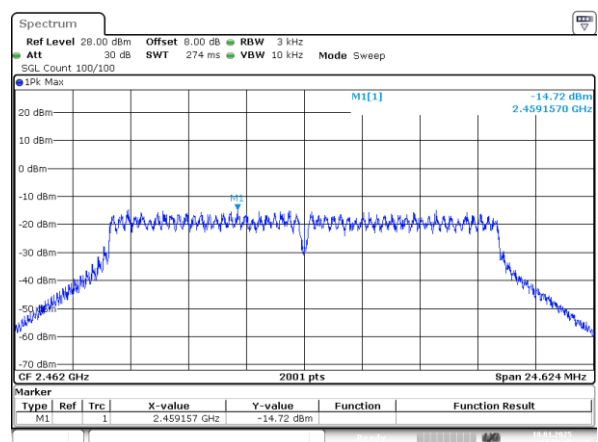
802.11g_2462MHz
