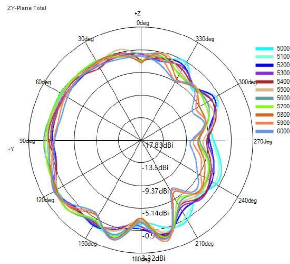
(2) Y-Z Plane(unit:dBi):
