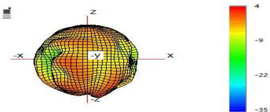
(4) Typical Free Space 3D Radiation Pattern at 5000MHz(unit:dBi):
