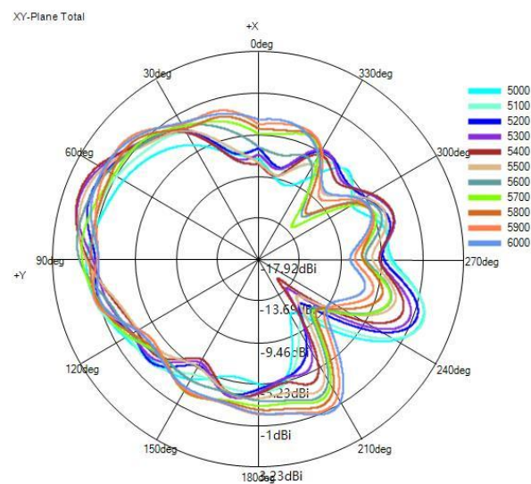
(3) X-Y Plane(unit:dBi):
