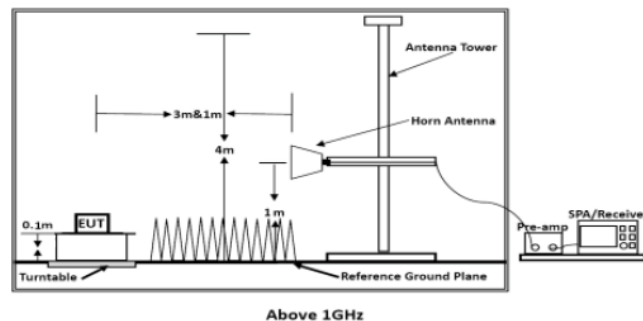
Figure 3. Above 1GHz
