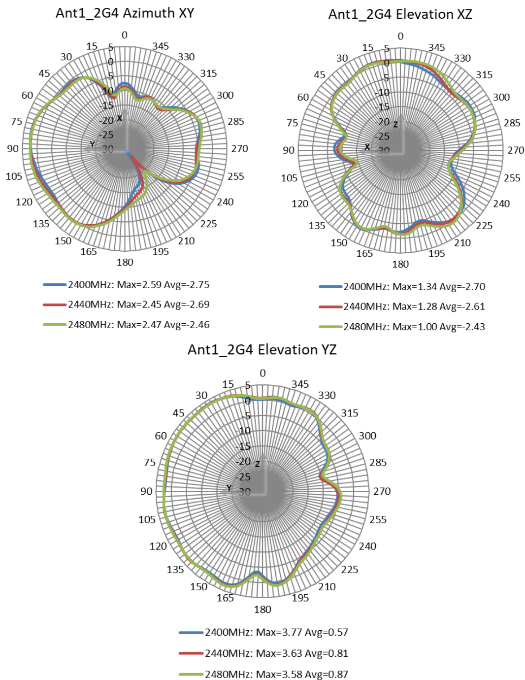
Figure 3: Model M01YCABA Radiation Patterns at 2.4 GHz & 2.44 GHz & 2.48 GHz
