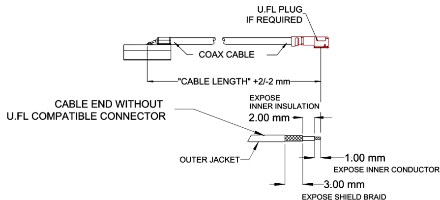
Figure 5: Airgain M01YCABA with connector or stripped cable
