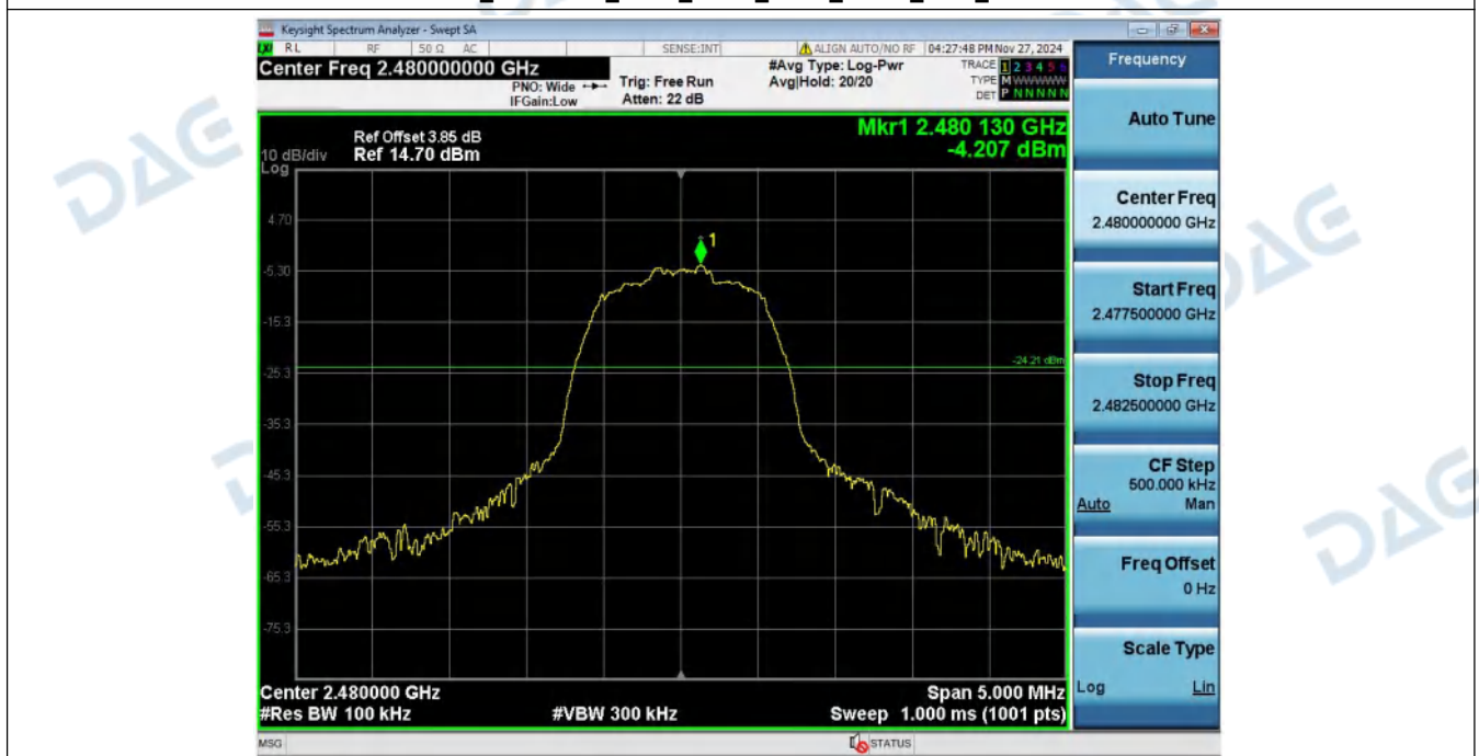
2_Spurious_Emissions_NVNT_ANT1_2-DH5_2480_00
