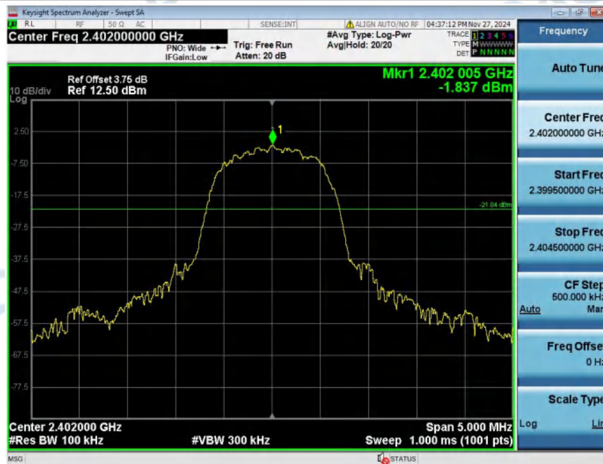
2_Spurious_Emissions_NVNT_ANT1_3-DH5_2402_00
