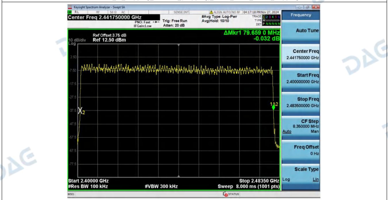
Number_of_Hopping_Channel_(Hopping)_NVNT_ANT1_2-DH5_Hopping
