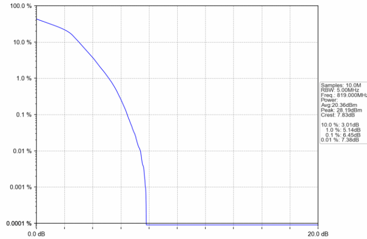
Band26a_1.4MHz_16QAM_MCH_819MHz_RB_6_0_NTNV
