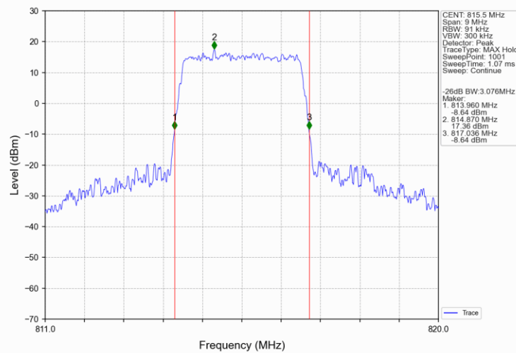
Band26a 3MHz 16QAM LCH 815.5MHz RB 15 0 NTNV
