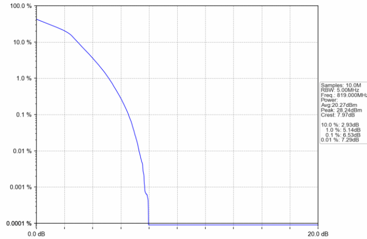
Band26a_3MHz_16QAM_MCH_819MHz_RB_15_0_NTNV
