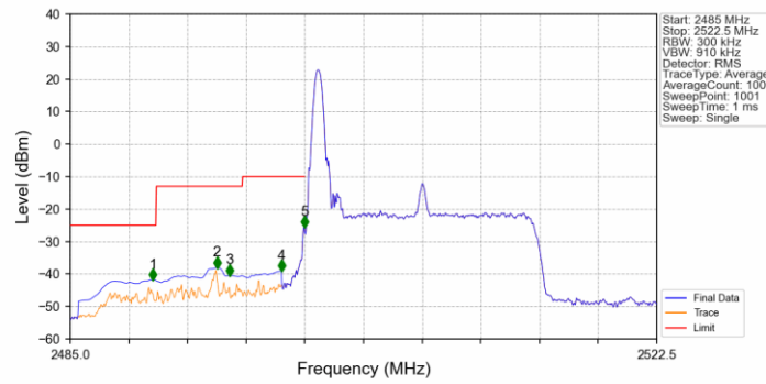
Band7_15MHz_QPSK_LCH_2507.5MHz_RB_1_0_NTNV
