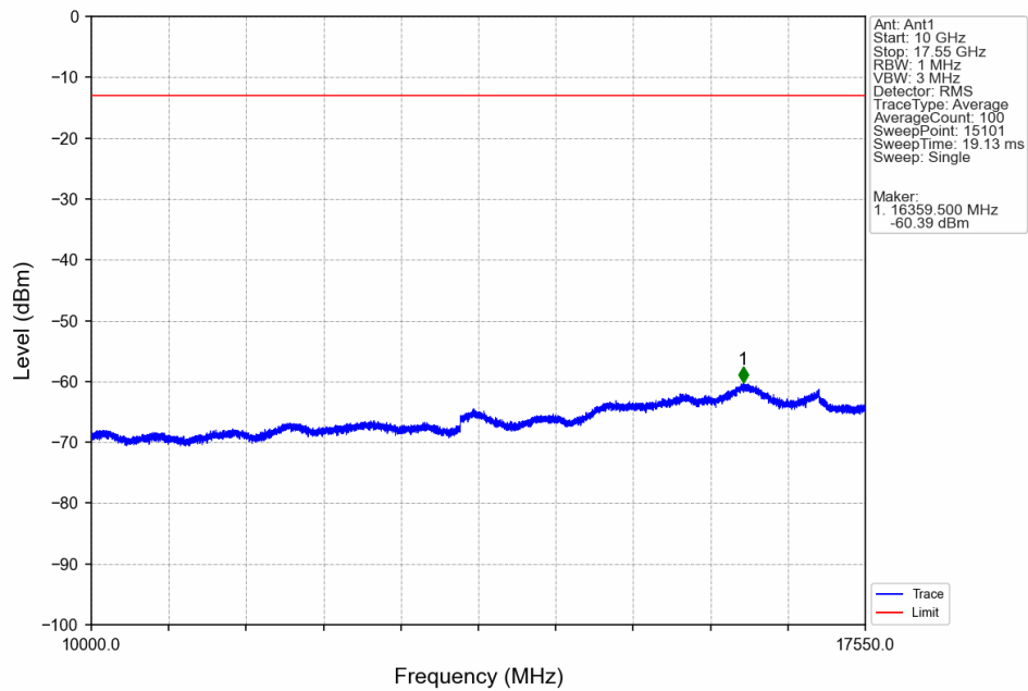
Band4_1.4MHz_16QAM_LCH_1710.7MHz_RB_1_0_NTNV
