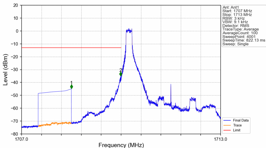
Band4_3MHz_QPSK_LCH_1711.5MHz_RB_1_0_NTNV
