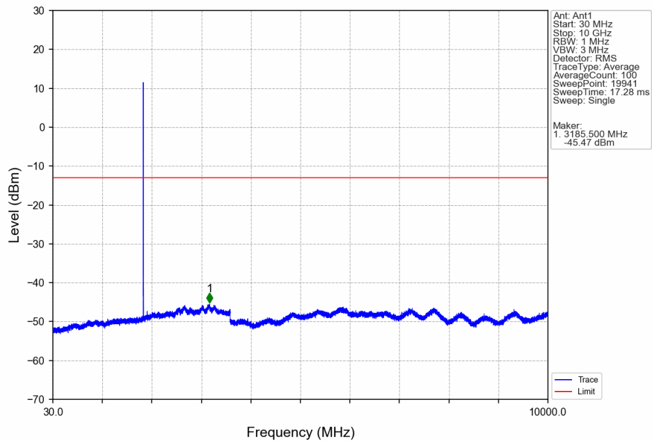
Band2_3MHz_16QAM_LCH_1851.5MHz_RB_1_0_NTV
