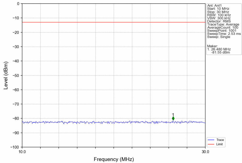
Band2_5MHz_16QAM_LCH_1852.5MHz_RB_1_0_NTV
