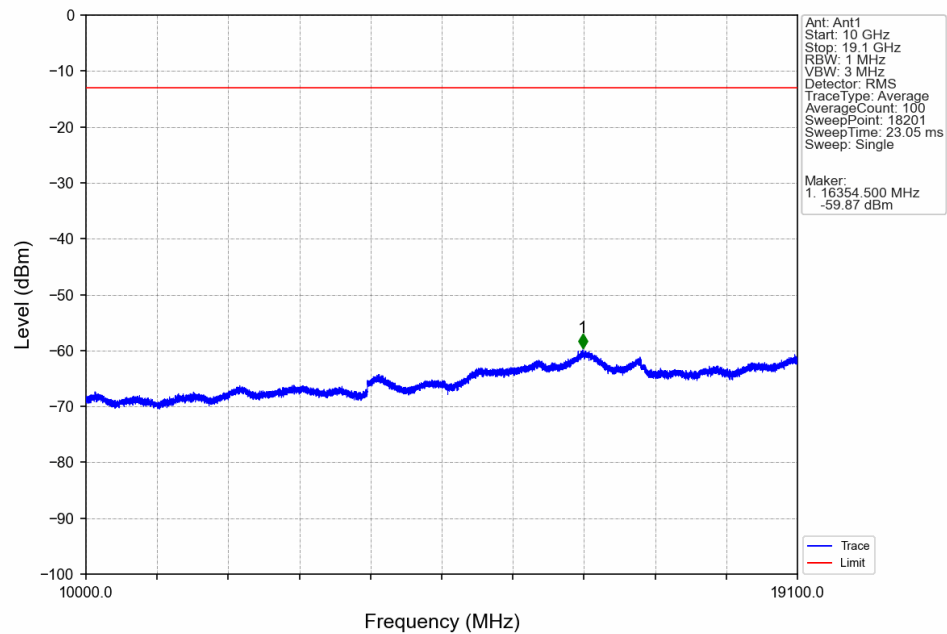
Band2_5MHz_16QAM_LCH_1852.5MHz_RB_1_0_NTV
