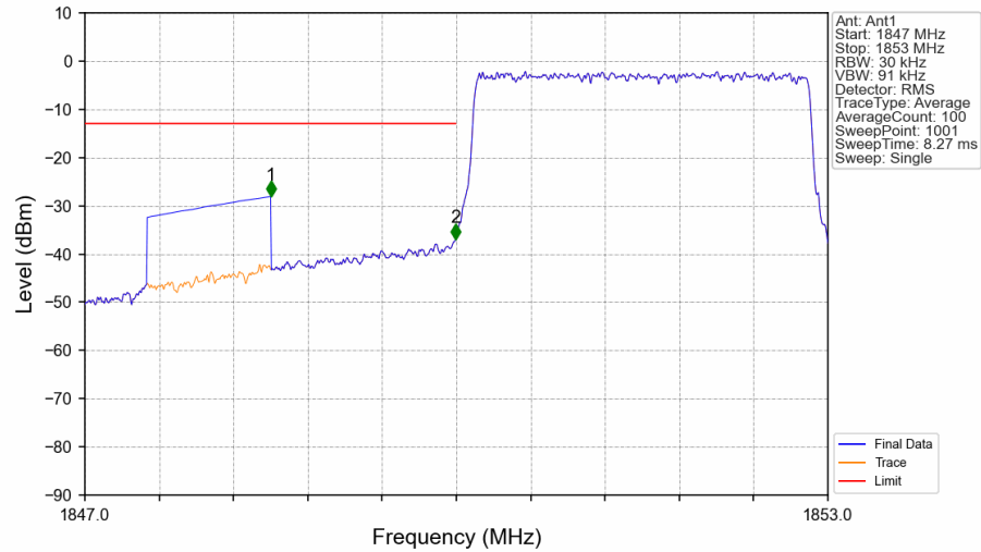
Band2_3MHz_16QAM_LCH_1851.5MHz_RB_15_0_NTNV
