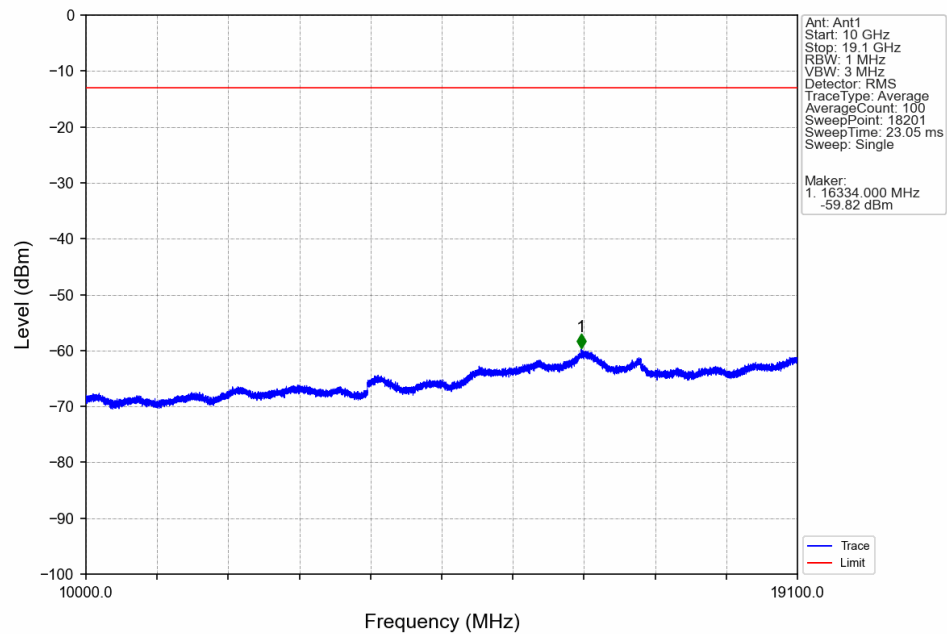
Band2_3MHz_16QAM_LCH_1851.5MHz_RB_1_0_NTV
