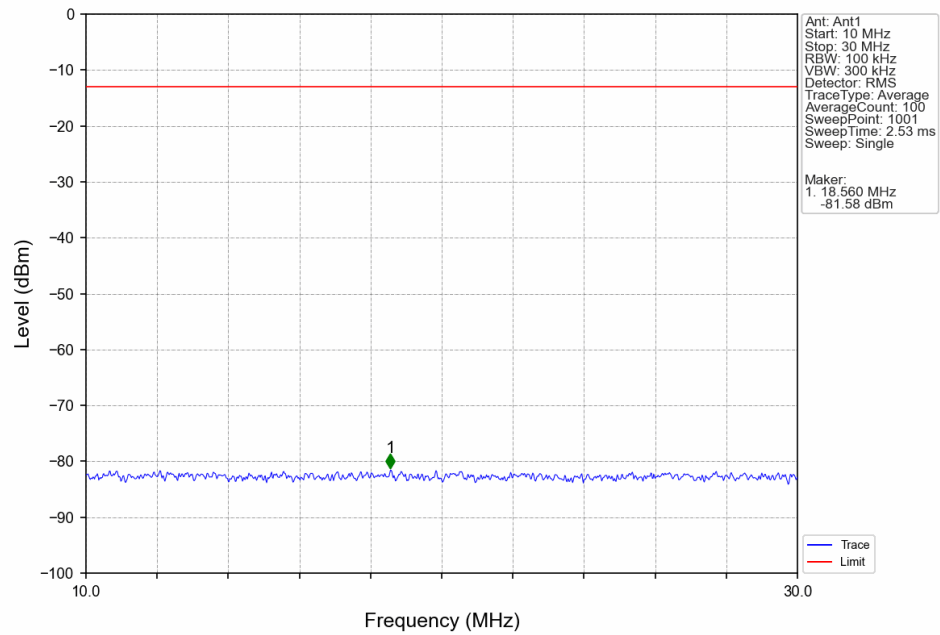
Band2_3MHz_16QAM_LCH_1851.5MHz_RB_1_0_NTV
