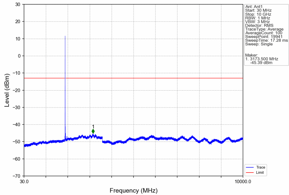
Band2_10MHz_16QAM_HCH_1905MHz_RB_1_0_NTN
