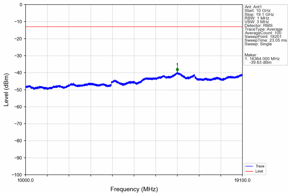
Band2_10MHz_16QAM_HCH_1905MHz_RB_1_0_NTN
