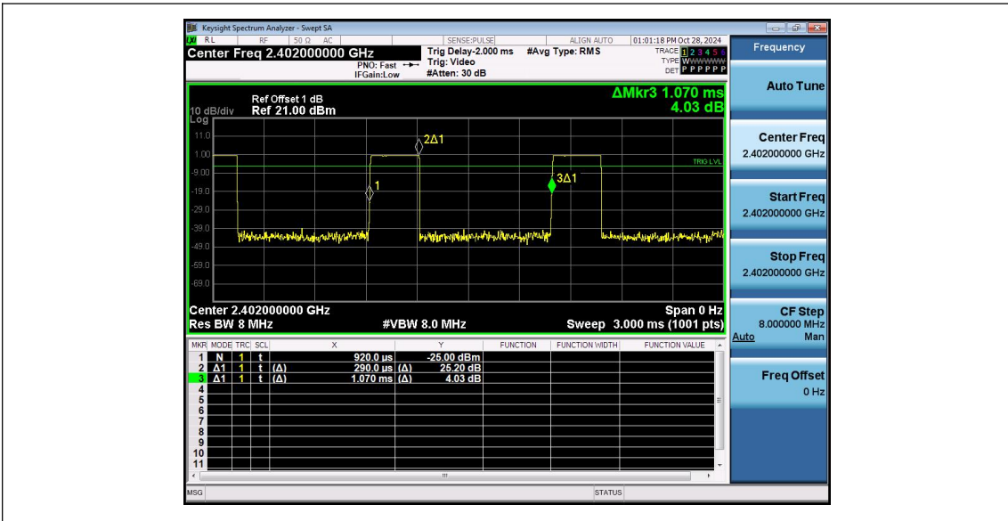
NTNV-BLE_1M-Ant1-2402
