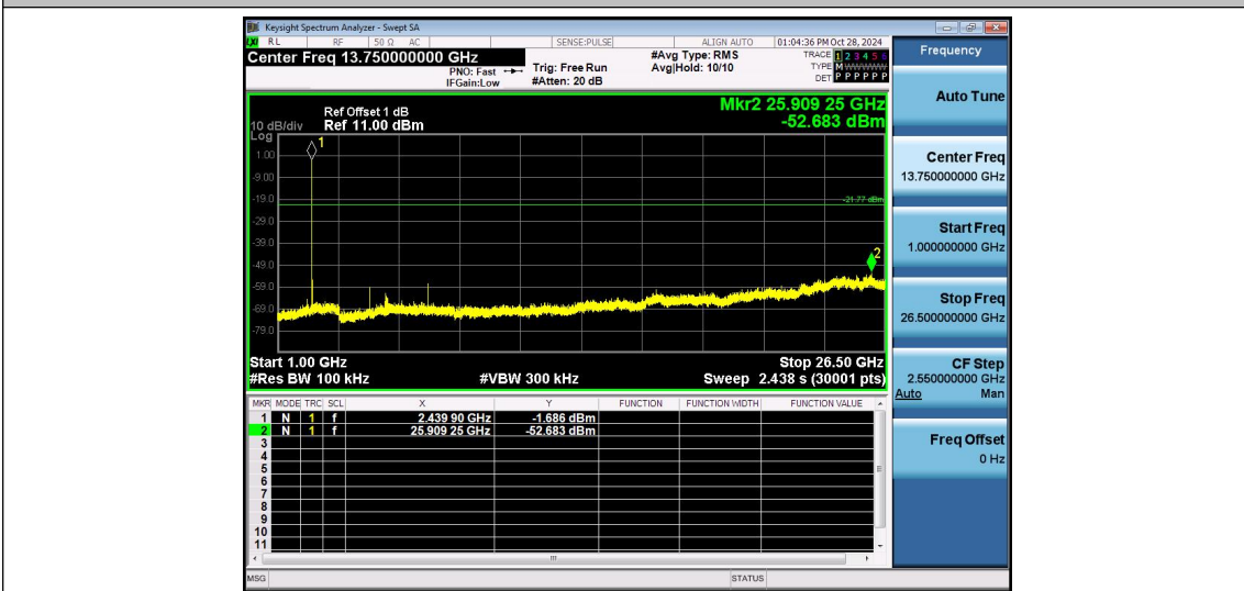
BLE_1M-Ant1-2440-1000~26500-PASS
