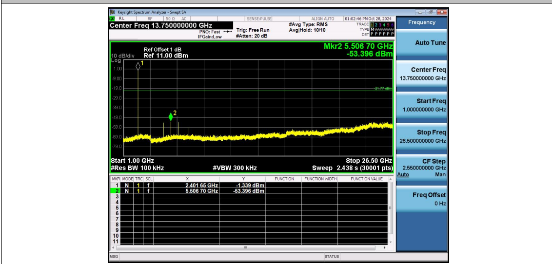
BLE_1M-Ant1-2402-1000~26500-PASS
